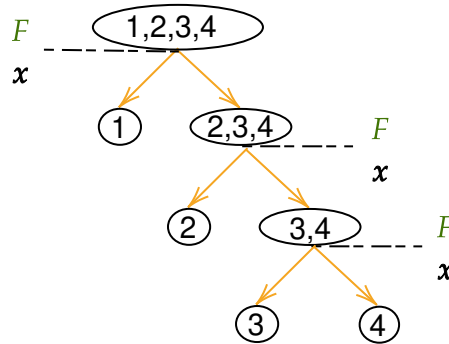
Figure 7: (J - 1) -PCGLM.
