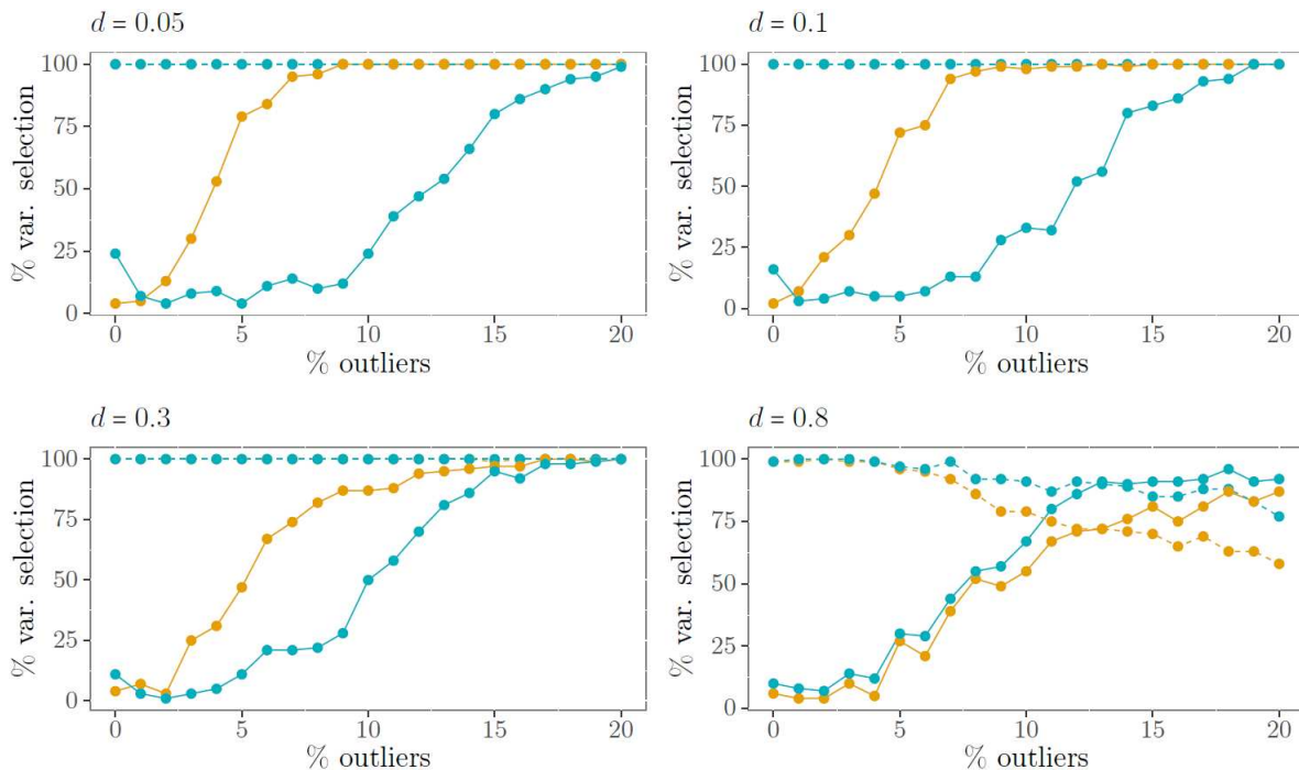
Figure 17: Average number of times the stepwise (backward) algorithm selects discriminant variables (dashed lines) and noisy variables (solid lines) where \delta^t = (1, 0) . The blue and yellow colors respectively represent the Student and logistic links.
