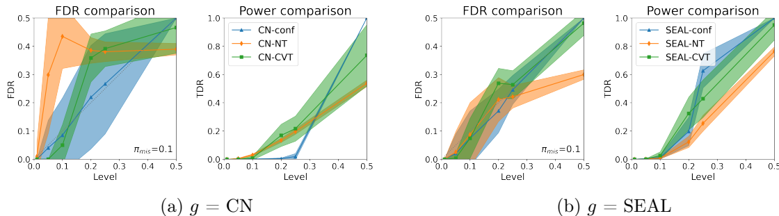
Figure 4.7: FDR (left panel) and TDR (right panel) as a function of the nominal level \alpha . Here \pi_{\text{miss}} = 10\% , |\mathcal{H}_0|/|\mathcal{H}_1| = 50\% , and |\mathcal{D}_{\text{cal}}| = 5000 . In (a) for the scoring function we use Common Neighbors and in (b) we use SEAL (Zhang and Chen, 2018). The bands indicate the standard deviation.
