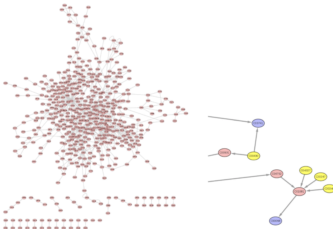
Figure 1.9: A metabolic network (Weber Zendrer et al., 2019): nodes represent molecules, edges denote chemical reactions. The right panel displays a zoom of the network.
