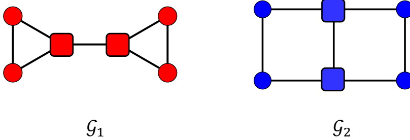
Figure 5.1: Two graphs that are locally equivalent but non-isomorphic. For each graph, the nodes can be separated in two classes; the border ones (circle nodes) and the centre ones (square nodes). Interestingly, while it is easy to see that these two graphs are not isomorphic, nodes have the same neighbourhood in both graphs. Indeed, in each graph the circle nodes have degree two and square nodes have degree three. Moreover, circle nodes are adjacent to a circle node and a square node, and each square node is adjacent to another square node and two circle nodes. All-in-all, they are indistinguishable by their local structure but non-isomorphic.
