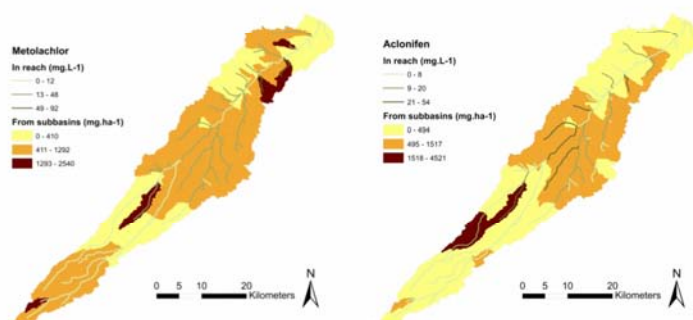
432 Figure 3 Surface water pesticide contamination risk maps on the Save catchment (case of metolachlor and 433 aclonifen). Values represent the magnitude of pesticide concentrations in reach and pesticide loads from subbasins when applying pesticides 15 days before their average spreading date and 15 days later their average spreading date.
