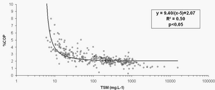
372 Figure 3 Relationship between Particulate Organic Carbon (POC) content (% of dry weight) and Total Sediment Matter (TSM) concentration (mg.L -1 ) at catchment outlet (January 2007 to October 2010).
