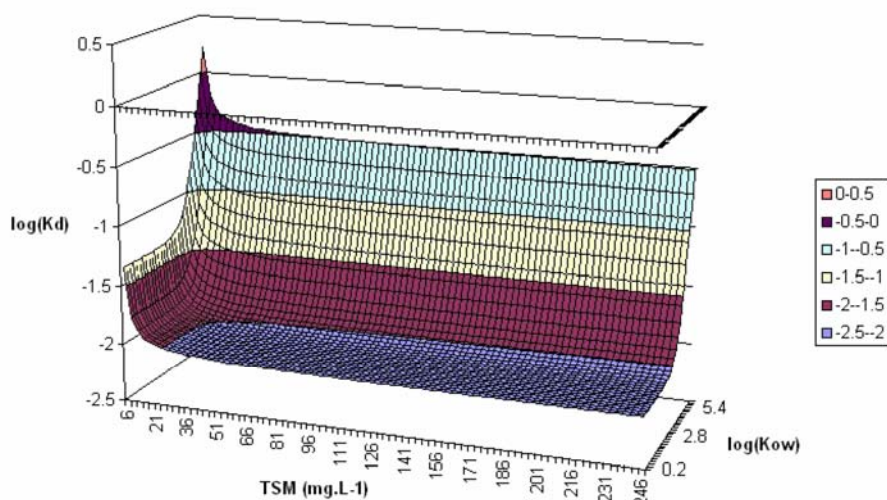
Figure 6 Relationship between \log(K_d) , \log(K_{ow}) and Total Suspended Matter (TSM) concentration.
