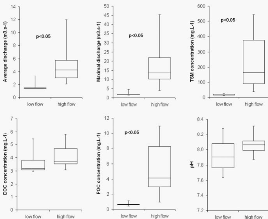
375 Figure 4 Boxplots of average discharge, maximal discharge, Total Sediment Matter (TSM) concentration, Dissolved Organic Carbon (DOC) concentration, Particulate Organic Carbon (POC) concentration and pH during low flow (5 samples) and high flow periods (11 samples) from July 2009 to October 2009. Significantly different means are highlighted by p<0.05 (Fisher's test). 378
