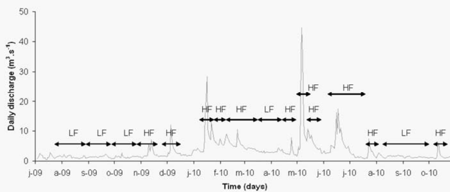
366 Figure 2 Daily observed discharge ( \text{m}^3 \cdot \text{s}^{-1} ), with 11 high flow (HF) periods and 5 low flow (LF) periods (July 2009 – October 2010).
