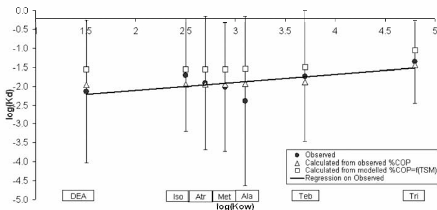
381 Figure 5 Relationship between the K_{ow} of 7 molecules and \log(K_d) calculated from observed pesticide concentrations, from observed percentage of Particulate Organic Carbon (%POC) in Total Suspended Matter (TSM) concentration, and modelled as a function of TSM (July 2009 – October 2010). Error bars represent standard deviations.
