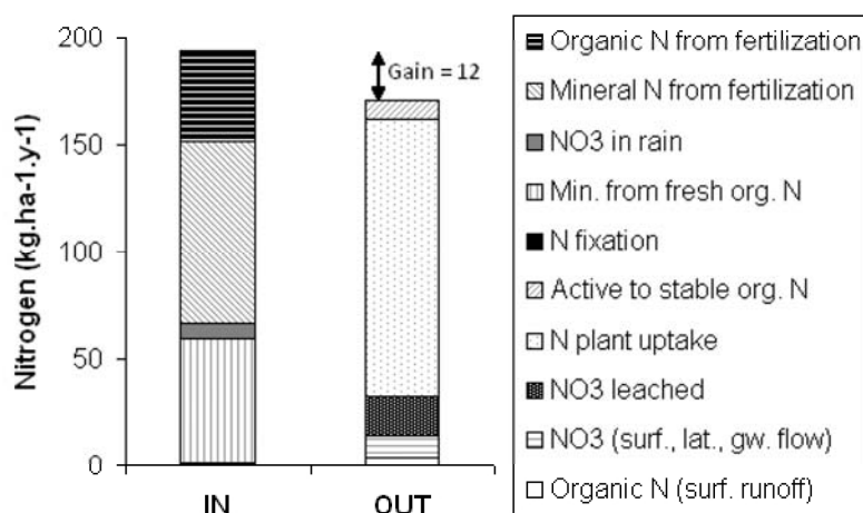
Figure 6 Simulated annual average nitrogen balance ( \text{kg}\cdot\text{ha}^{-1}\cdot\text{y}^{-1} ) on the Save catchment (1998-2010).
