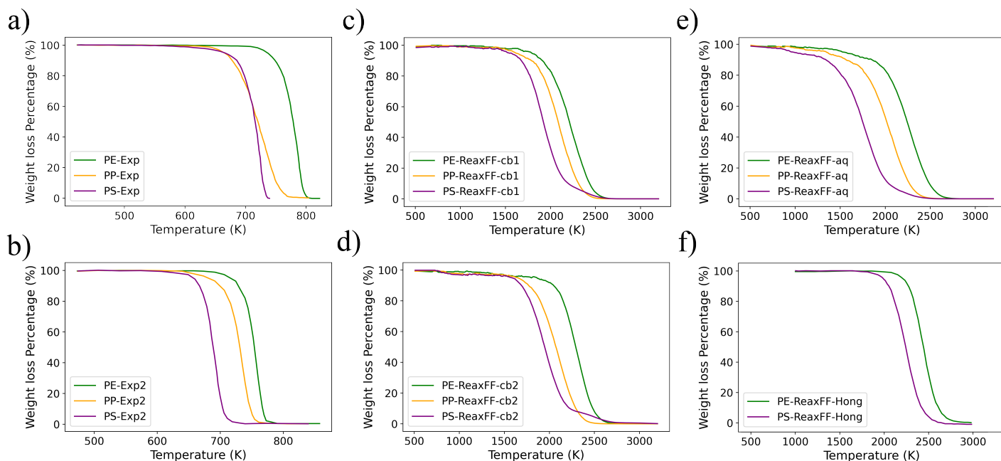
Figure 4.3: Thermogravimetric analyses obtained from experimental studies and ReaxFF simulations for pure PP, PE and PS polymers. a) and b) are experimental work of Abbas-Abadi 269 and Dümichen et al. 253 ; ReaxFF simulations of this work with c) CHOSFCIN potential 60 ; d) CHON-2019 potential 62 ; e) CHONCl-2022_weak 277 . f) ReaxFF simulations from the work of Hong et al. 271 . c), d) and f) correspond to potential from the combustion branch and e) from the aqueous branch. Purple, green and orange curves correspond to the TG of PS, PE and PP respectively.
