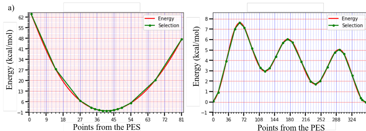
Figure 3.7: Representation of two examples of selected points from two different scans. On the left is the choice from the angle Cl-C-C of the dichlorobenzene meta and on the right is the torsion Cl-C-C-H of the chloroethanol. The red curve represents the full PES, and the green is the selected curve.
