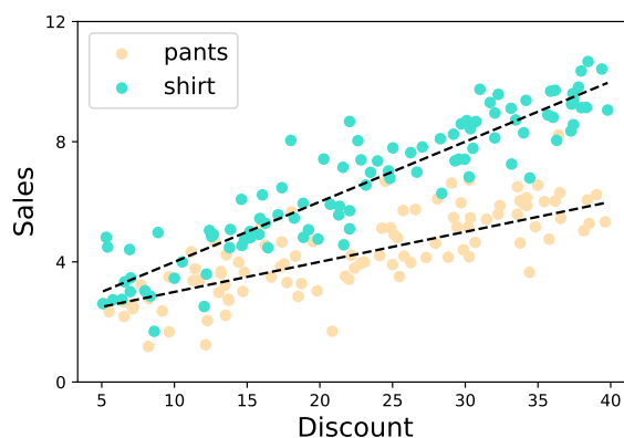
Figure III.1.: Relational linear regression.
