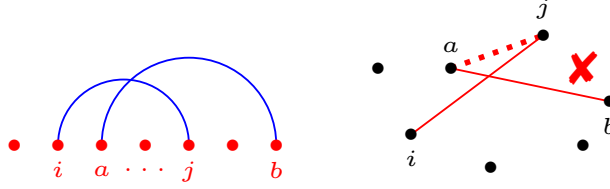
Figure 29: Coherent arborescences on a polytope whose graph is complete are non-crossing. For i < a < j < b with A(i) = j , then Lemma 3.5 ensures that \frac{\langle \omega, v_j - v_a \rangle}{\langle \omega, v_j - v_a \rangle} > \frac{\langle \omega, v_b - v_a \rangle}{\langle \omega, v_b - v_a \rangle} , so A(a) = b is impossible.
