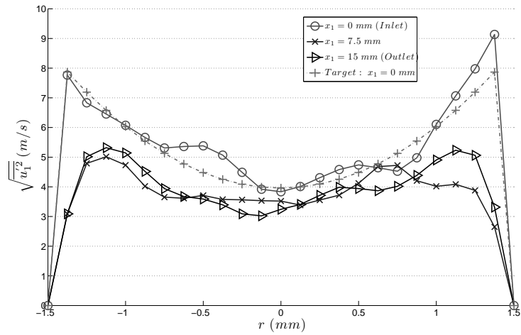
(a) \sqrt{u_1'^2}
