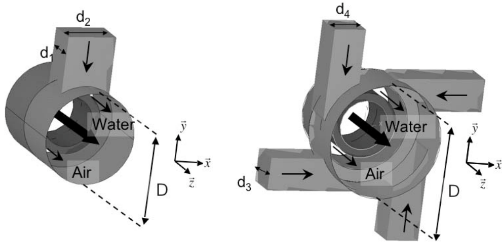
(b) 3D visualisation of the injector with the deviation control system (Dev55)
