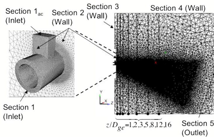
(b) Grid for the configuration (Dev55)
