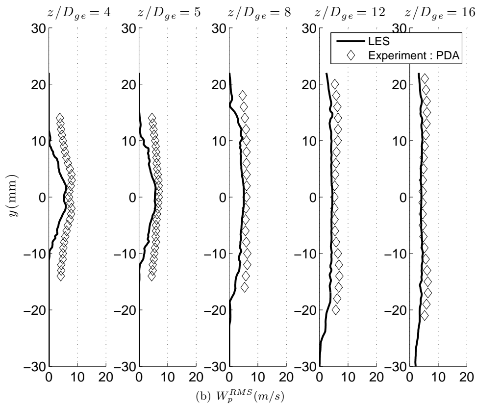
FIGURE 6.30 – (Coax) 50\mu m < d_p < 100\mu m : Radial profiles of mean (Top) and RMS (bottom) axial particle velocity at x = 0 . Comparison between LES and Experiment.
