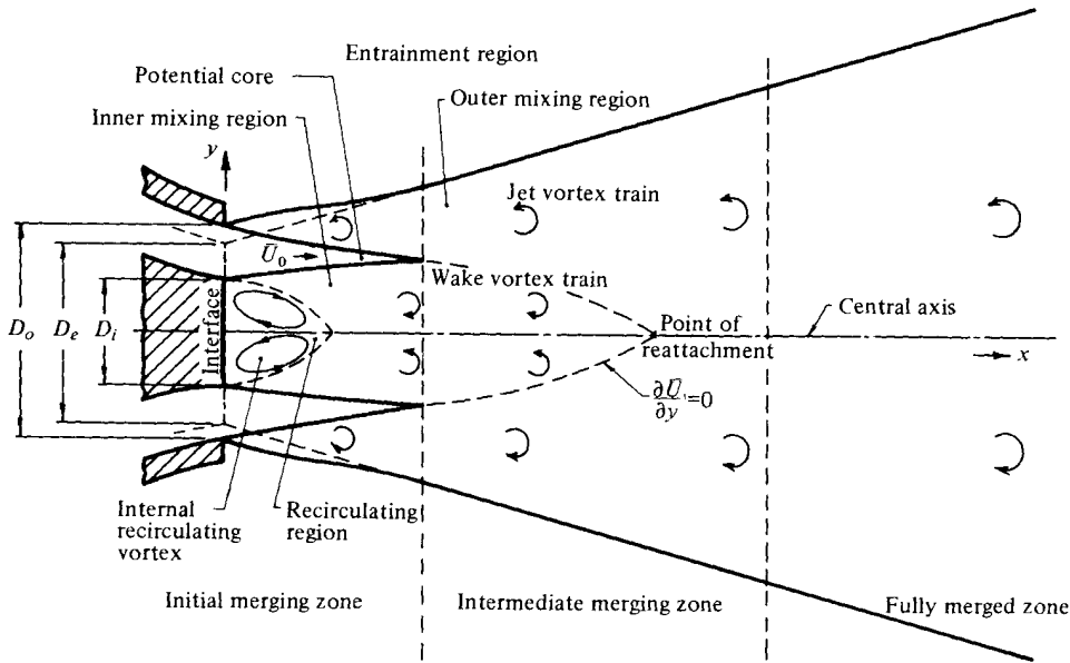
FIGURE 6.5 – Schematic profile of initial region of annular jet (Ko and Chan 1978 [109])
