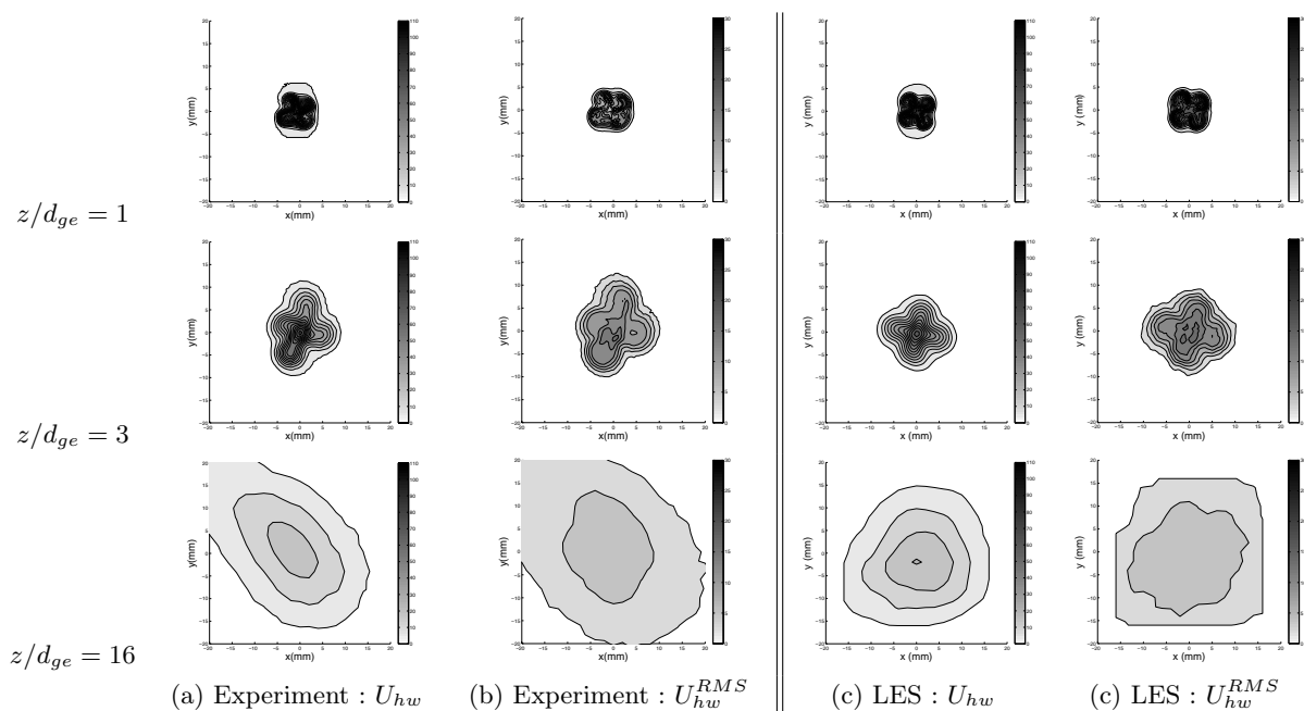
FIGURE 6.11 – (Dev55) : Hot-wire mean and RMS velocity fields. Comparison of Experiment and LES.
