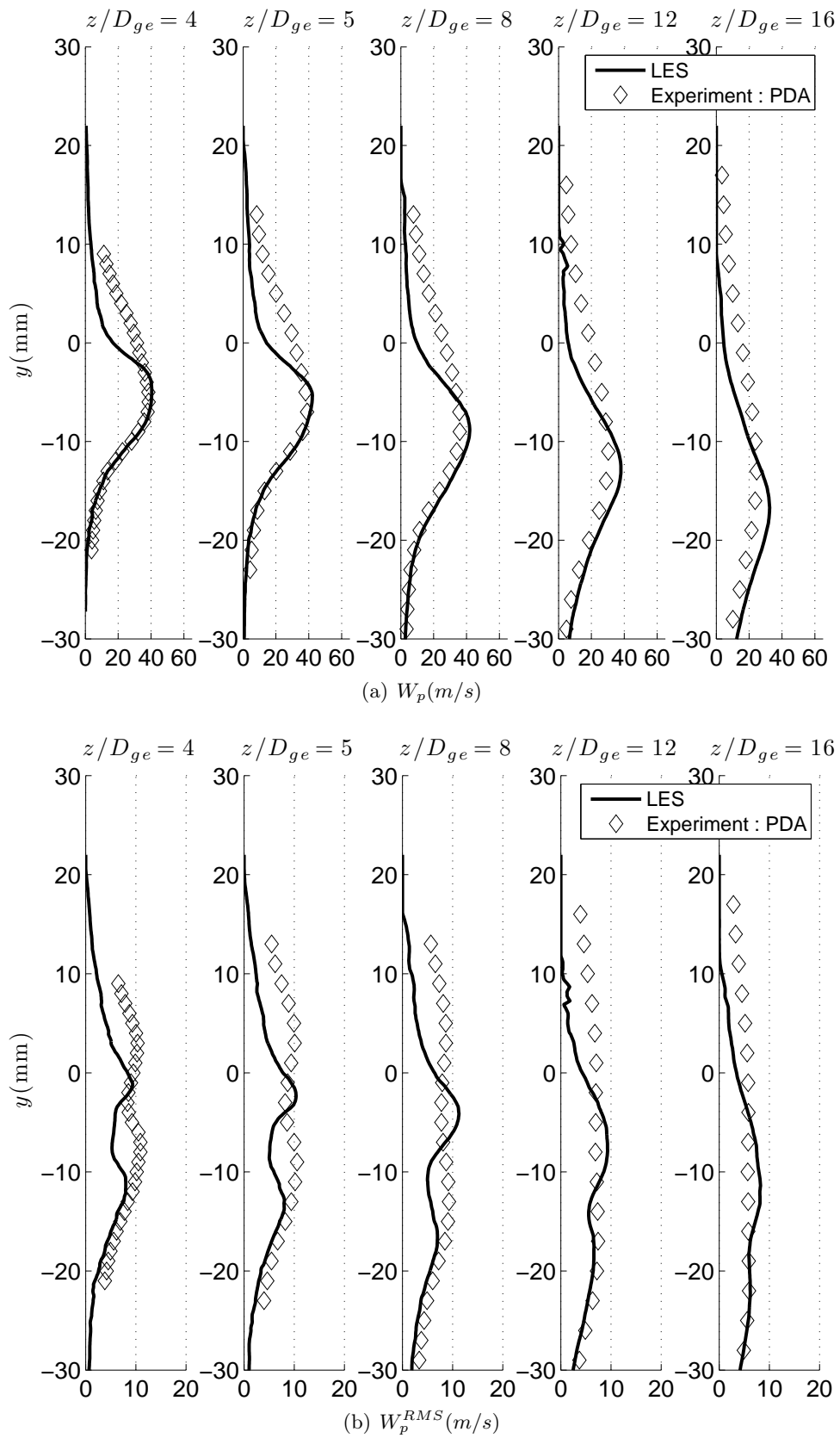
FIGURE 6.32 – (Dev55) 20\mu m < d_p < 50\mu m : Radial profiles of mean (Top) and RMS (bottom) axial particle velocity at x = 0 . Comparison between LES and Experiment.
