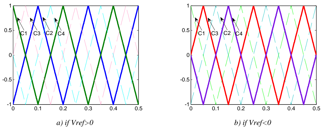
Figure V.8: Equivalence between modified PS and PD for the 3-level parallel converters.
