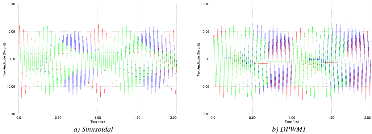
Figure V.12: ICT flux using DPWMI and SPWM techniques.
