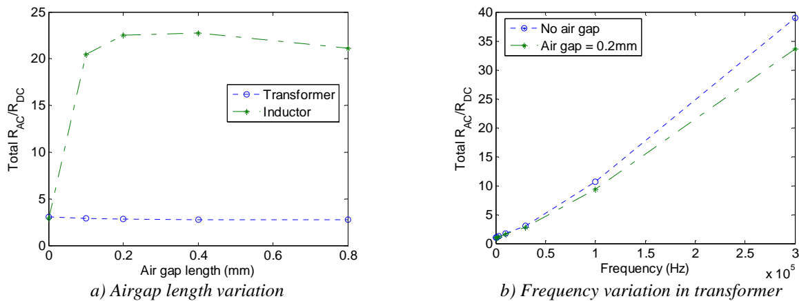
Figure II.20: Influence of airgap in the AC/DC resistance ratio.
