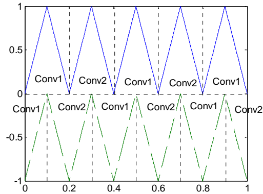
Figure V.7: Carriers for PD technique for 3-level converters.
