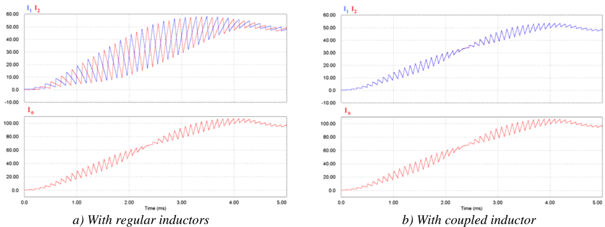
Figure I.12: Cell and output currents for uncoupled and coupled inductors.
