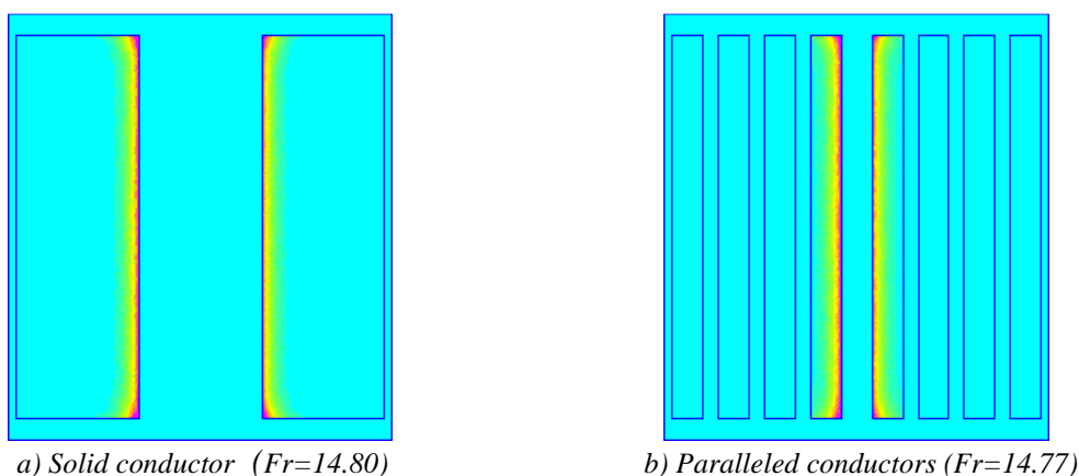
Figure II.29: Current density in solid and paralleled conductors.
