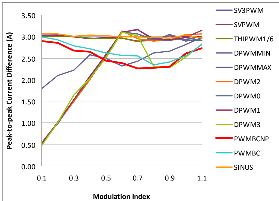
Figure V.50: Comparison of PWM methods: maximum peak-to-peak current difference obtained by experimental results.
