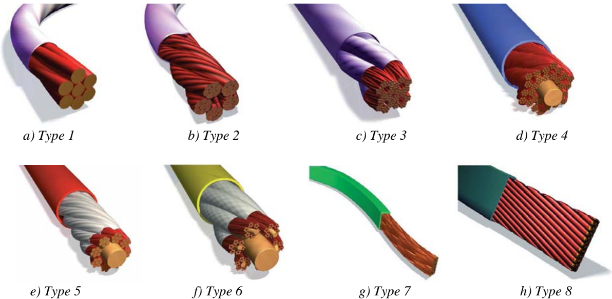
Figure II.30: Litz wire types and construction [77].
