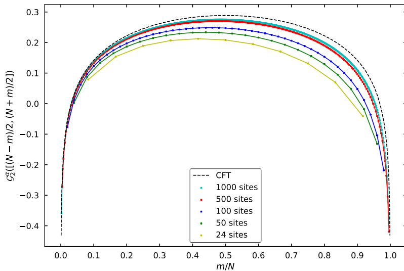
Figure 2.7: Plot of shifted Rényi entropy \mathcal{G}_2^f([(N-m)/2, (N+m)/2]) for a wide range of system sizes. The sizes typically accessible to exact diagonalization ( N \sim 10 ) or DMRG methods ( N \sim 10^3 ) suffer from large finite-size effects.
