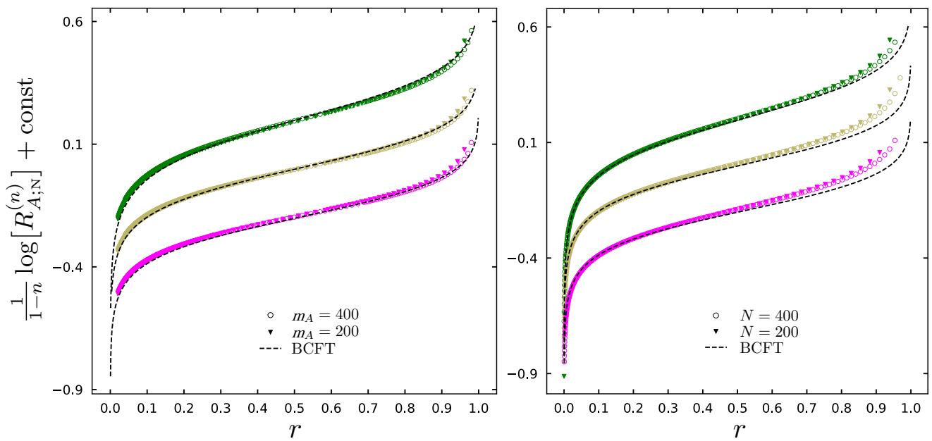
Figure 3.8: The UV finite ratio (3.13) for the bipartitions shown in Figure 3.1 with Neumann BC and n \in \{3, 13, 50\} , with the same colour code of Figure 3.7. We have introduced artificial vertical shifts of the curves for different values of n to enhance the distinguishability of the data.
