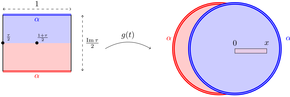
Figure 2.2: The annulus \mathbb{A}_\tau – fundamental domain pictured here – is mapped through g to the two-sheeted disk \mathbb{D}_{2,x} . The black edges are identified.
