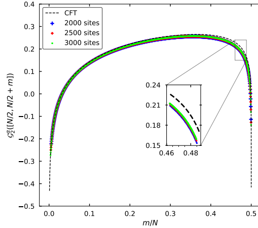
Figure 2.5: Plot of shifted Rényi entropy \mathcal{G}_2^f([N/2, N/2+m]) for the Ising chain with free BC, against the scaled interval size m/N . The deviations from the theoretical predictions are stronger as the interval grows closer to the boundary.
