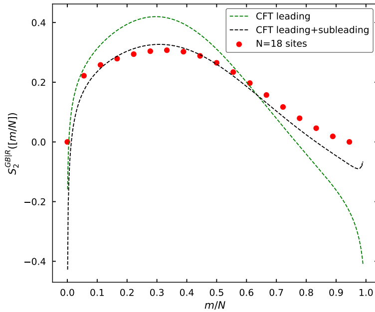
Figure 4.7: Comparison of the second Rényi entropy in the critical three-state Potts chain of size M = 18 with mixed ( GB, R ) BC with CFT results.
