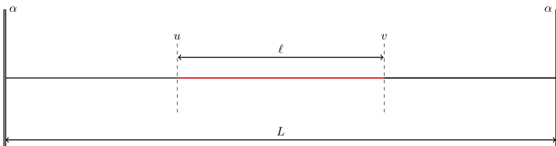
Figure 2.1: Interval in the bulk of a system with open BC
