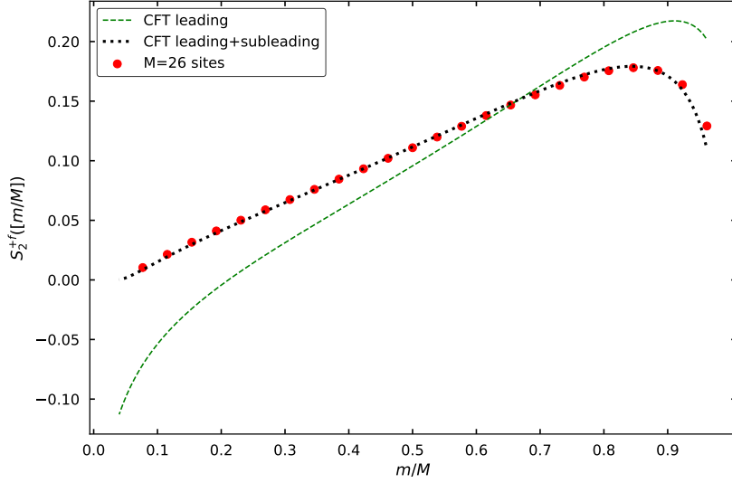
Figure 4.5: Comparison of the second Rényi entropy in the critical Ising chain of size M = 26 with mixed free fixed BC with CFT results. Inclusion of the subleading term in the expansion 4.24 is crucial for obtaining a satisfying agreement with lattice data
