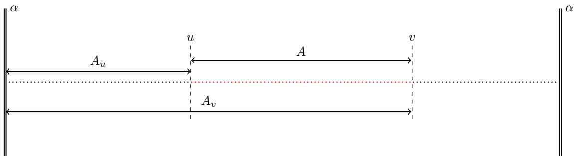
Figure 3.6: The three intervals relevant for constructing UV finite ratios (3.13). For the semi-infinite chain, the \alpha boundary on the right is sent to infinity
