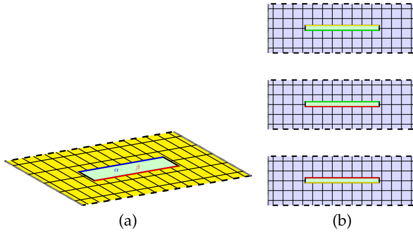
Figure 1.1: (a) The cylinder partition function associated to a matrix element (\rho_A)_{\alpha\beta} of the ground-state density matrix \rho_A . The solid grey edges are identified. (b) The partition function associated to \text{Tr}_A(\rho_A^n) for n = 3 . The solid grey edges are identified. The colours on the sides of the slits indicate the sewing order of the copies.
