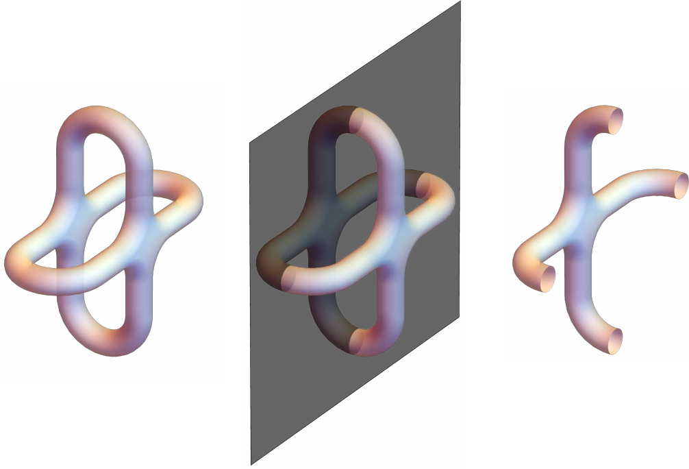
Figure 3.2: The Riemann surface \mathcal{S}_4 (right panel) is topologically a sphere with four boundaries. It is obtained by exploiting the reflection symmetry of \mathcal{M}_4 for two equal intervals (left panel) with respect to a plane (the black plane in the middle panel).
