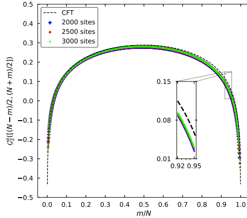
Figure 2.6: Plot of shifted Rényi entropy \mathcal{G}_2^f([(N-m)/2, (N+m)/2]) for the Ising chain with free BC, against the scaled interval size m/N . The deviations from the theoretical predictions are stronger as the interval is grown towards the boundaries.
