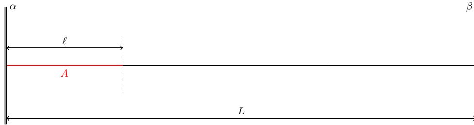
Figure 4.1: An interval of length \ell in a 1d critical chain with mixed BC ( \alpha\beta ) and length L .
