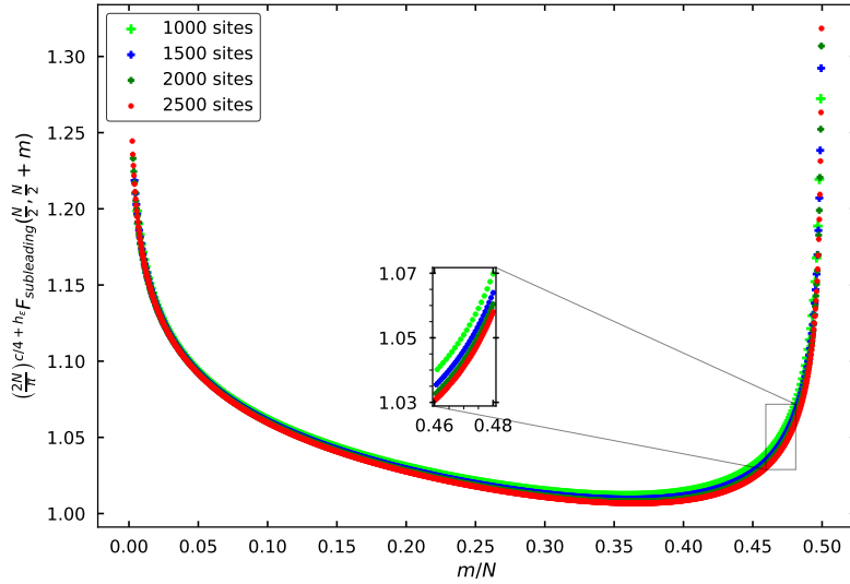
Figure 2.8: The rescaled subleading contribution (2N/\pi)^{c/4+h_\epsilon} F_{\text{subleading}} to the lattice two-point function of twist fields, for an interval starting in the middle of the chain and growing towards one boundary. The plot shows that even at large system sizes, the finite-size corrections are significant.
