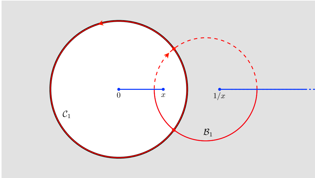
Figure 3.4: The cycles (red curves) employed in Sec. 3.2.1. Solid curves lie in the first sheet, while dashed lines stand for curves on the second sheet. The unit disk \mathbb{D} corresponds to the white region. The twist fields are located at the origin and x .
