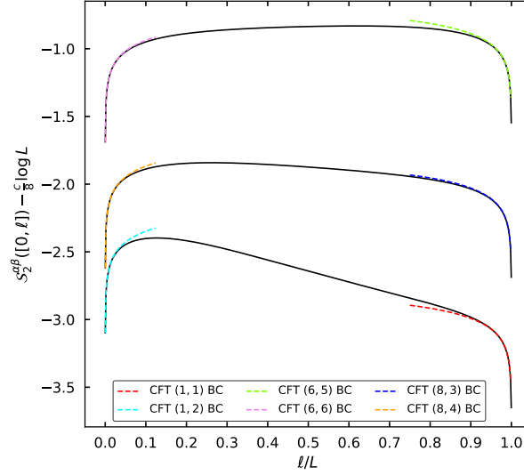
Figure 4.2: Shifted second Rényi entropies for the mixed BC setups ((1, 2), (1, 1)) , ((6, 6), (6, 5)) and ((8, 4), (8, 3)) for the BCFTs based on \mathcal{M}(10, 9) . The black curves denote the mixed BC prediction interpolating between the identical BC results in each case.
