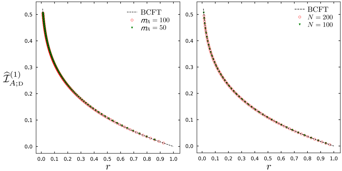
Figure 3.10: The UV finite quantity (3.102) for Dirichlet BC. The dashed curves correspond to the BCFT prediction (3.78). The results for the semi-infinite chains and the finite chains made by N sites are reported in the left and right panels respectively.
