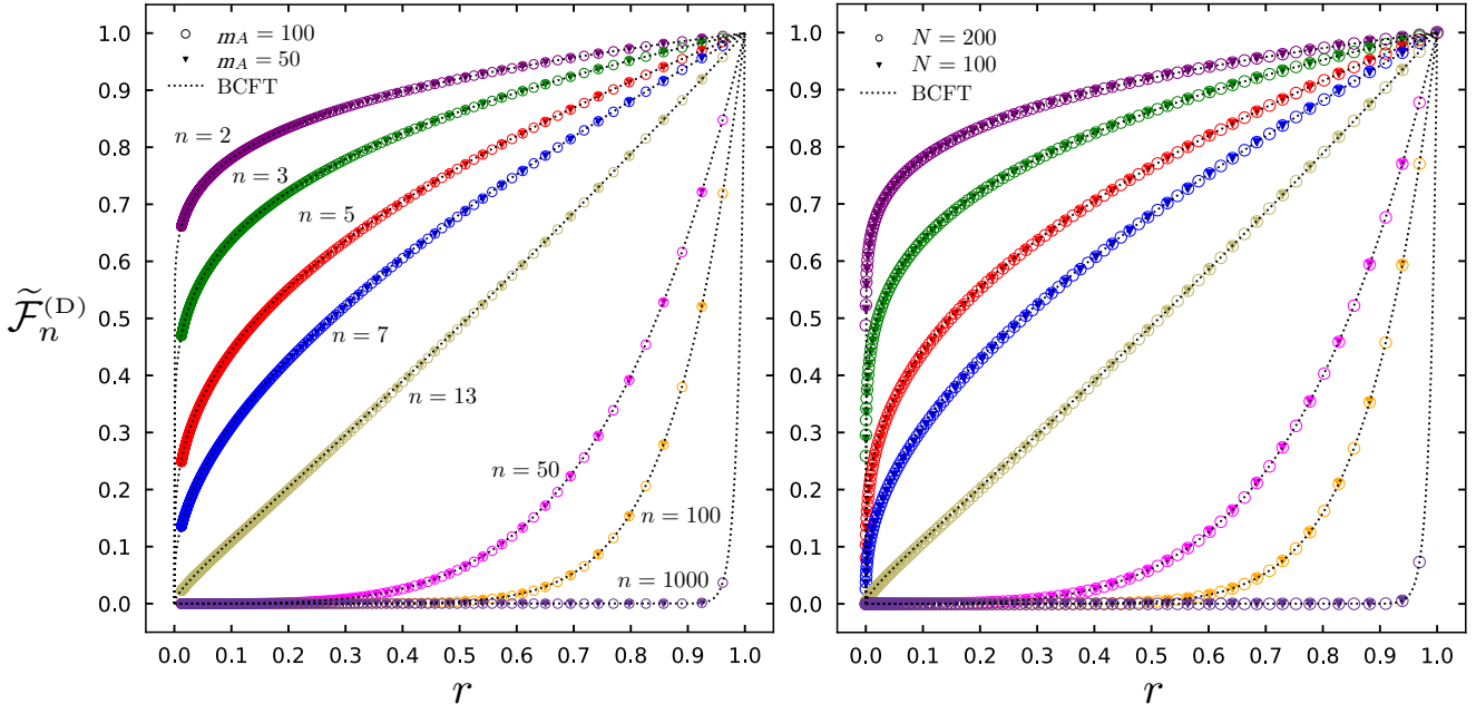
Figure 3.5: The function \tilde{\mathcal{F}}_n^{(D)} for the bipartitions in Figure 3.1 with Dirichlet boundary conditions. The black dotted lines correspond to the BCFT result given by the first expression in (3.28). The data points have been obtained for the block of m_A consecutive sites either in the semi-infinite chain (left panel) or on the finite chain made by N sites (right panel) with Dirichlet BC (see Sec. 3.3).
