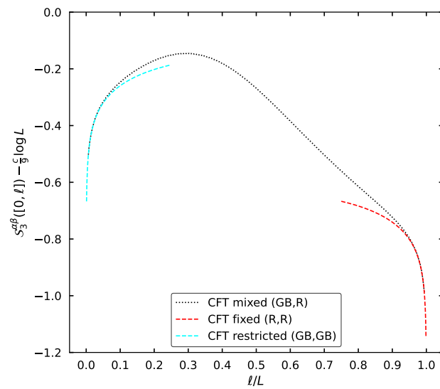
Figure 4.8: Comparison of shifted third Rényi entropies for (GB, R) , (R, R) and (GB, GB) BC. The mixed BC curve can be seen to interpolate between the identical BC results
