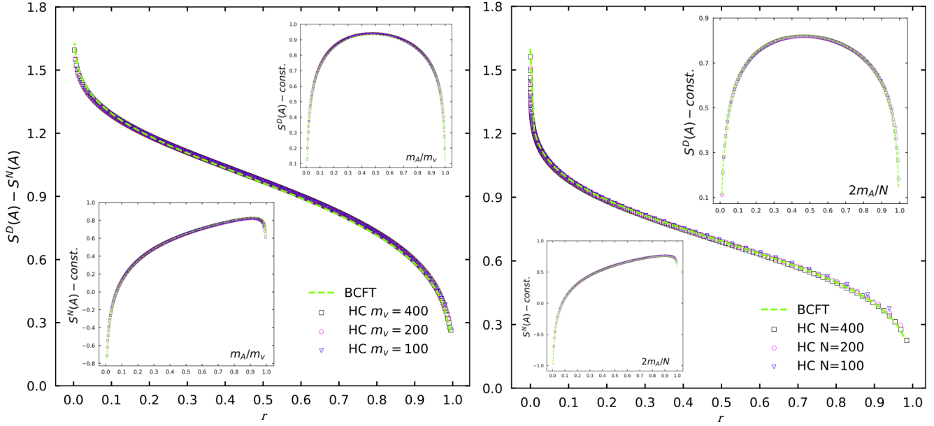
Figure 3.9: The difference between the entanglement entropy for Dirichlet BC and Neumann BC for the bipartitions of Figure 3.1, either in the semi-infinite chains (left panel) or in the finite chains (right panel). The insets show the entanglement entropy for the two different boundary conditions. The BCFT curves have been obtained from (3.76).
