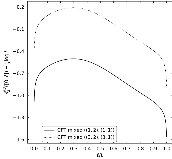
Figure 4.3: Shifted second Rényi entropies for the mixed BC setups ((1, 2), (1, 1)) and ((3, 2), (3, 1)) for the BCFTs based on \mathcal{M}(6, 5) . The difference between the two curves is constant with respect to the interval size, and thus fixed by their respective asymptotic behaviours around \ell \rightarrow 0 and \ell \rightarrow L
