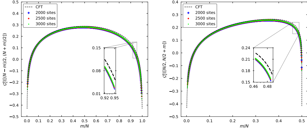
Figure 2.3: Plots of shifted Rényi entropy \mathcal{G}_2^f([m_u, m_v]) for the Ising chain with free BC, against the scaled interval size m/N . The deviations from the theoretical predictions are stronger as the interval is grown towards the boundaries
