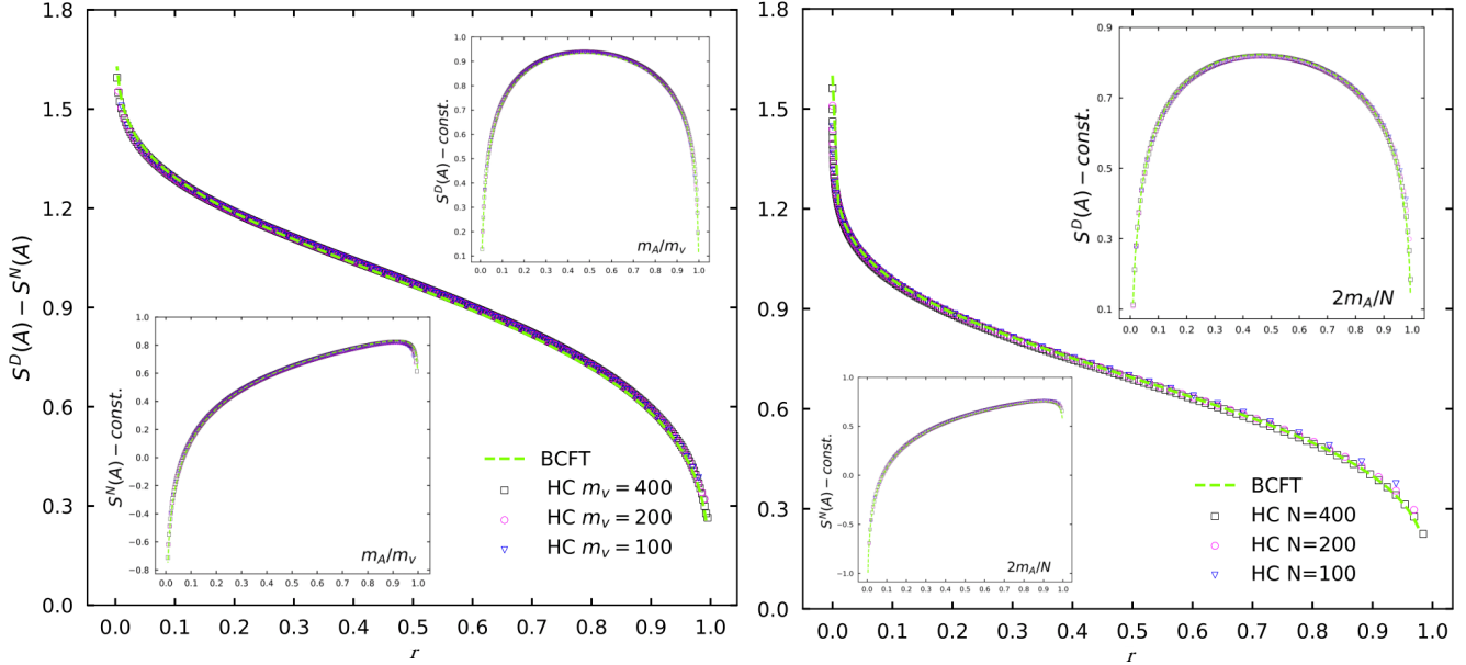
Figure 3.3: The difference between the entanglement entropy for Dirichlet BC and Neumann BC for the bipartitions of Figure 3.1, either in the semi-infinite chains (left panel) or in the finite chains (right panel). The insets show the entanglement entropy for the two different boundary conditions.
