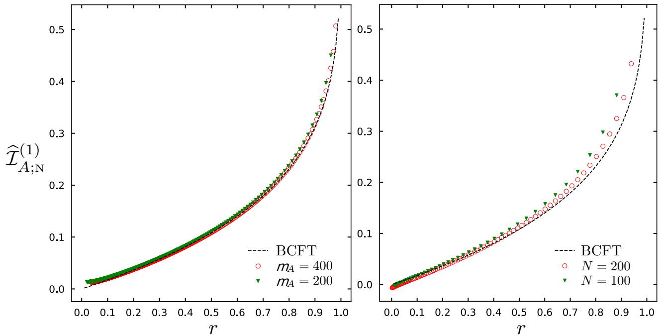
Figure 3.11: The UV finite quantity (3.102) for Neumann BC, with the same notation described in the caption of Figure 3.10.
