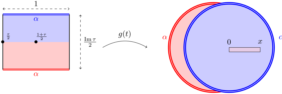
Figure 2.4: The annulus \mathbb{A}_\tau – fundamental domain pictured here – is mapped through g to the two-sheeted disk \mathbb{D}_{2,x} . The black edges are identified.
