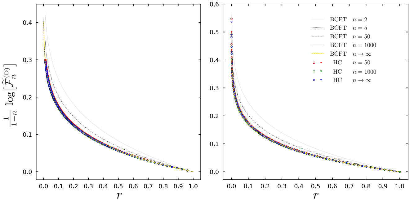
Figure 3.12: Single copy entanglement entropy for the bipartitions in Figure 3.1 (see (3.103)) when Dirichlet BC are imposed. The same harmonic chains of Figure 3.5 have been employed.
