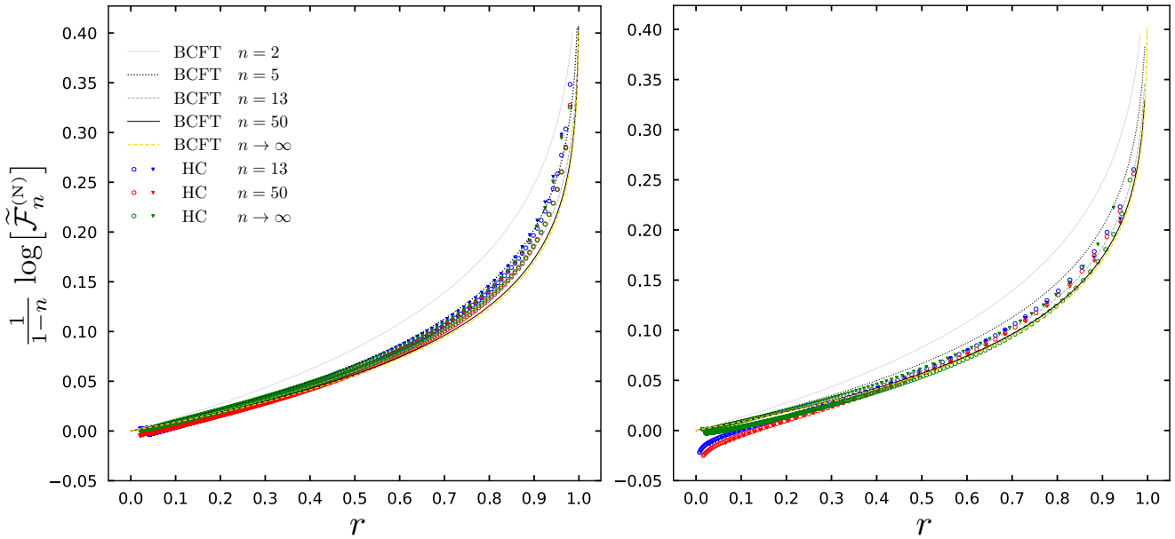
Figure 3.13: Single copy entanglement entropy for the bipartitions in Figure 3.1 (see (3.103)) when Neumann BC are imposed. The same harmonic chains of Figure 3.7 have been employed.
