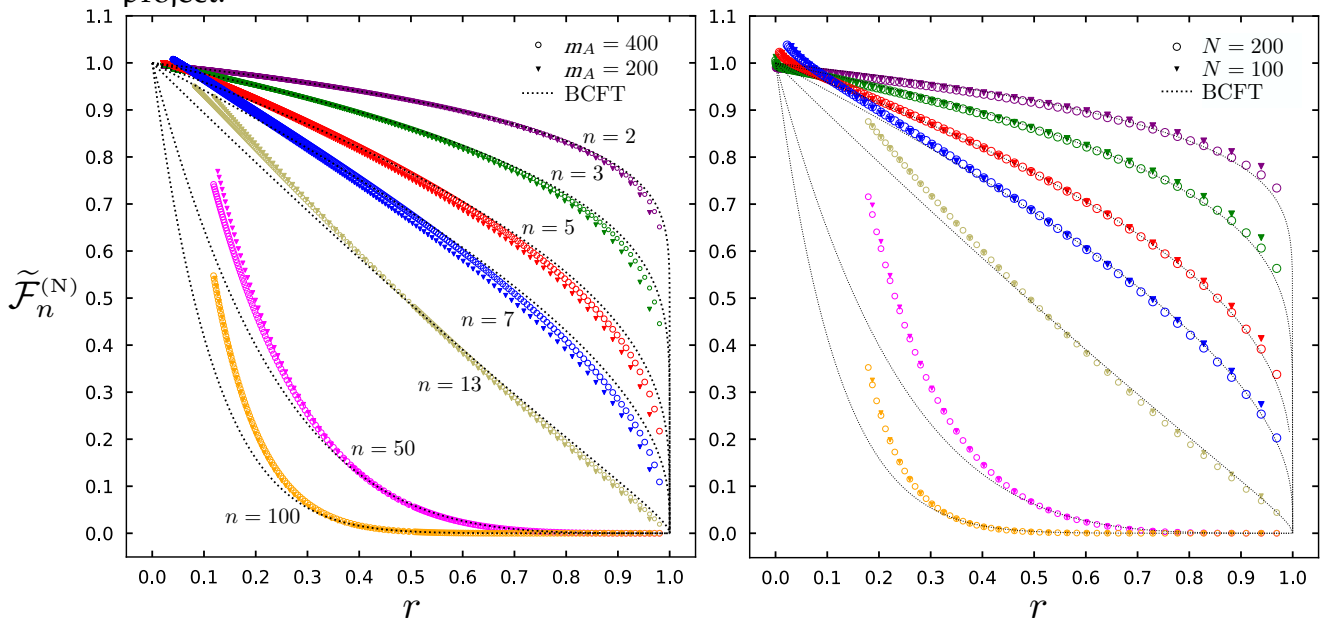
Figure 3.7: The function \tilde{\mathcal{F}}_n^{(N)} for the bipartitions in Figure 3.1 with Neumann boundary conditions. The black dotted lines correspond to the BCFT result given by the second expression in (3.28). The data points have been obtained for the block of m_A consecutive sites either in the semi-infinite chain (left panel) or on the finite chain made by N sites (right panel) with Neumann BC, as discussed in Sec. 3.3.
