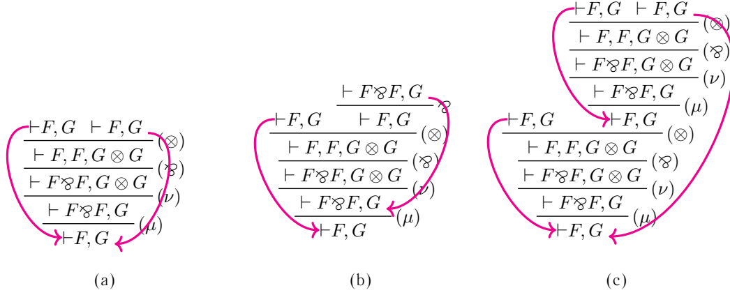
Figure 7.8: Different representations of the same circular proof of \vdash F, G where [F] = [G^\perp] = \mu x. x \otimes x_\alpha .
