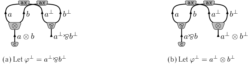
Figure 9.7: Instances of \mathcal{S} from Example 9.3.1
