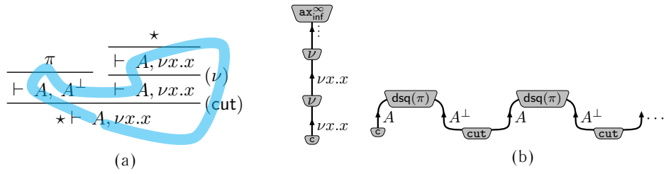
Figure 7.12: Exhibiting higher-order trips and visitable paths. Here \pi is the pre-proof in Figure 7.11a
