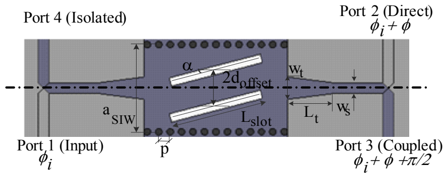
Fig. 4.5 The developed two-layer SIW coupler structure with microstrip to SIW transitions. a_{SIW} = 10.2 mm, L_{slot} = 10.7 mm, d_{offset} = 2.1 mm, \alpha = 15^\circ , slot width 1 mm, w_t = 2.6 mm, L_t = 4.9 mm and w_s = 1.29 mm.
