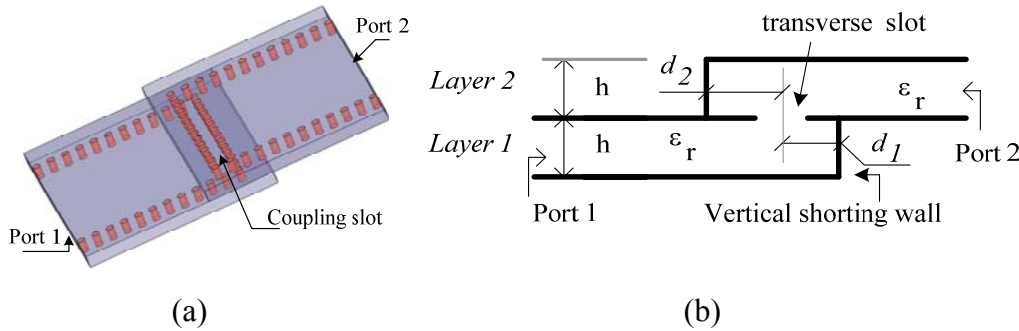
Fig. 2.7 Two layer transverse slot-coupled waveguide transition. (a) 3-D SIW structure. (b) Schematic longitudinal cross section.
