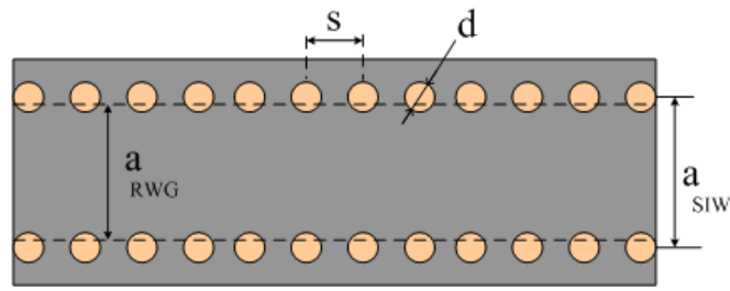
Fig. 1.1 Configuration of an SIW structure synthesized using metallic via-hole arrays.
