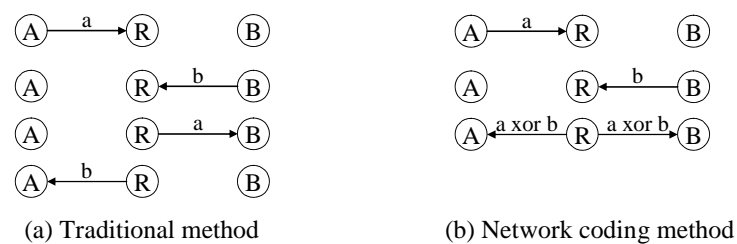
Figure 2.4.1: A simple network coding example.
