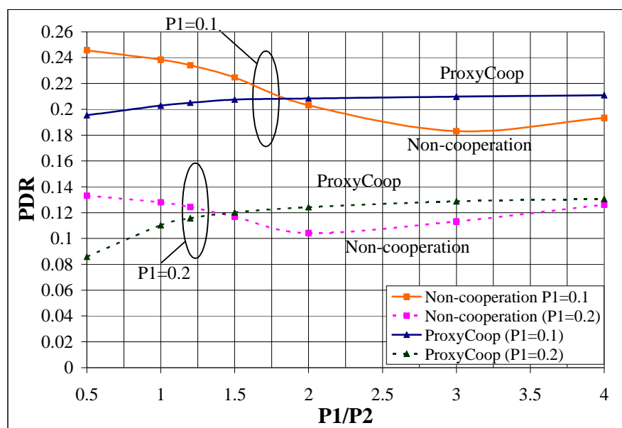
Figure 5.4.3.8: PDR of non-cooperative and ProxyCoop transmissions in the 9-terminal network.
