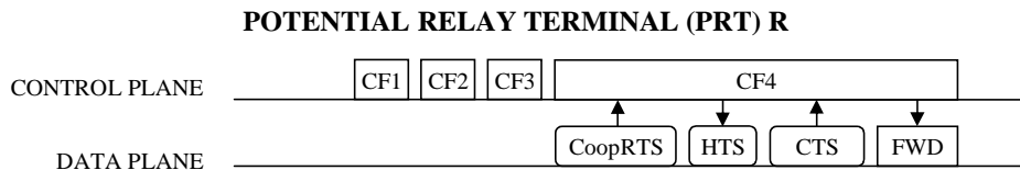
Figure 4.4.3.3: Data plane and control plane interactions of the CoopMAC protocol at a PRT R.
