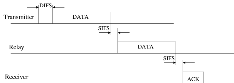
(a) Cooperative transmission in basic access method.
