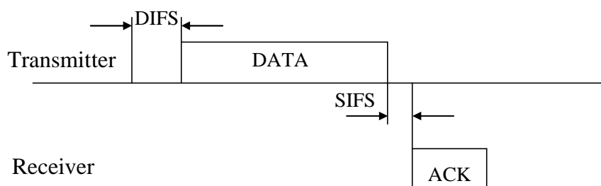
Figure 3.1.1.1: Basic access method of the IEEE 802.11 MAC standard.
