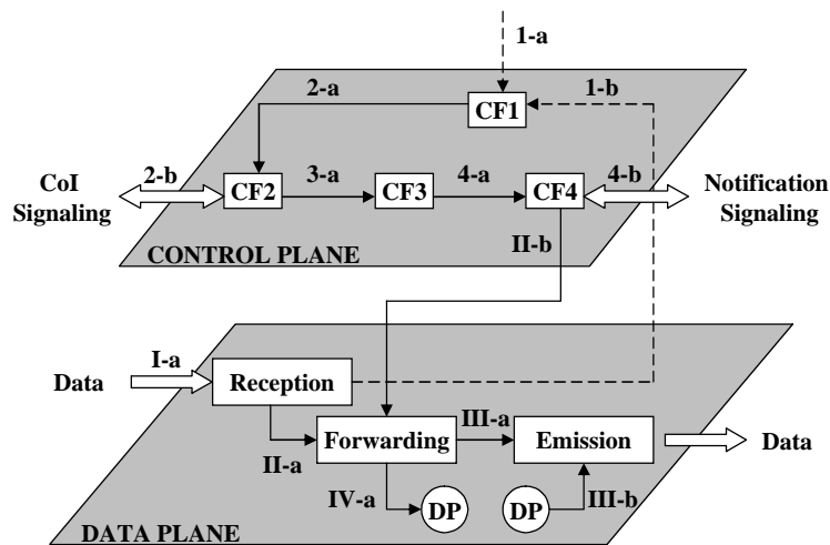
Figure 5.1.6: Cooperative Network Model.
