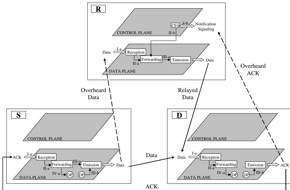
Figure 5.2.3: ProxyCoop transmission with basic access method of IEEE 802.11 MAC protocol on the cooperative network model.
