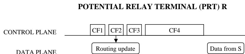
Figure 4.4.1.1: Data plane and control plane interactions of the ACR protocol at a potential relay terminal R.
