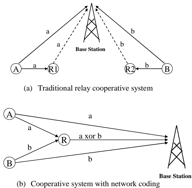
Figure 2.4.2: (a) Traditional relay cooperative system and (b) Cooperative system with network coding in a cellular network.
