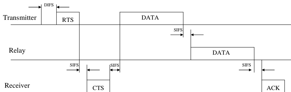
(b) Cooperative transmission in optional access method.
