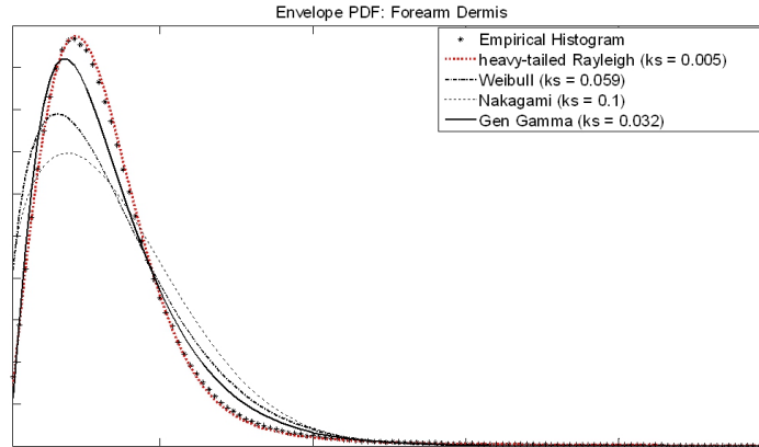
Figure 2.6: Comparison of the empirical envelope pdf obtained from forearm dermis, and the corresponding estimations using the heavy-tailed Rayleigh, Generalized Gamma, Weibull and Nakagami distribution.
