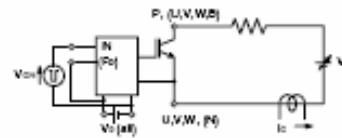
Fig. 5 OC and SC Test
