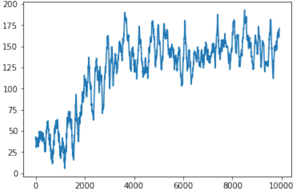
Figure 6.1: (Identical) rewards in the Power Unit Commitment game with our Fully Asynchronous FP procedure with \delta = 0.5
