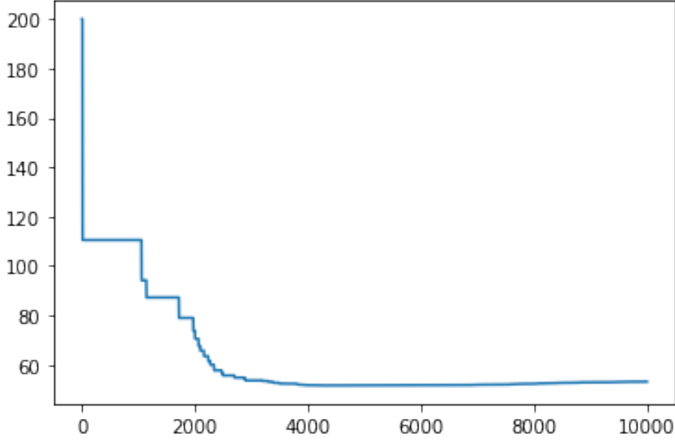
Figure 6.2: Continuation value of a random state in the Power Unit Commitment game with our Fully Asynchronous FP procedure with \delta = 0.5
