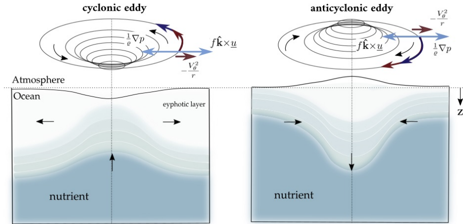
Figure 2.2: Schematic representation of the 3D structure of Cyclonic and Anticyclonic eddies. The surface trough and ridge owing to the (cyclo)geostrophic balance are schematically exaggerated. The corresponding shallowing and deepening of the mixed layer as well as the up/downwelling effects transferring nutrients from the deep to the euphotic layers are represented. Figure source: Ioannou, 2019
