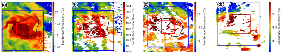
Figure I.3: Examples with different Cloud Coverage. Snapshots represent Sea Surface Temperature in degrees. Contours and squares are the same as Figure I.2. Snapshots of the same eddy (Ierapetra) on different days of December 2016 (a) 19/12 (b) 20/12 (c) 29/12 and (d) 30/12. Cloud coverage percentage is increasingly high. Examples (a) and (b) are retained while (c) and (d) are filtered
