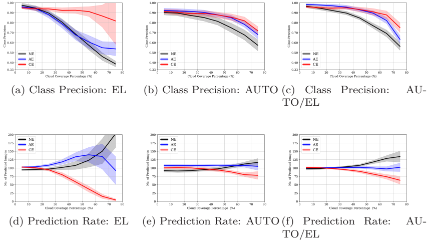
Figure III.7: Classifier performance the EDDIES-CLOUDY dataset. The y-axis of figures on the top line represents the Class Precision C_{i=j}^{pre} and on the bottom line the number of predicted images per class. Bold lines and envelopes represent respectively the mean and standard deviation of experiment runs (5-fold training and 10 test sets per CCP bin). Colours represent the performance over the three different classes (black for NE, blue for AE, red for CE). The x-axis represents the mean Cloud Coverage Percentage (CCP) range of the test set (0-10% to 70-80%). Figures in different columns show the performance of different classifiers.
