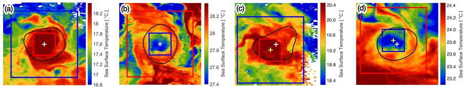
Figure I.2: Examples of the Eddy-Core Surface Temperature Anomaly computation and offset method. Snapshots represent Sea Surface Temperature in degrees. Black lines are superimposed altimetric detection contours. Small squares represent the core-mean and large ones the periphery-mean frames. Core-periphery are coloured red-blue or blue-red based on the sign of \delta T . Examples (a)-(d) illustrate the correction by offset: A white cross marks the center of the image. A yellow cross marks the center of the core-mean and periphery-mean frames, if it differs from the center of the image. Examples (a) and (b) are centered while (c) and (d) are offsetted.
