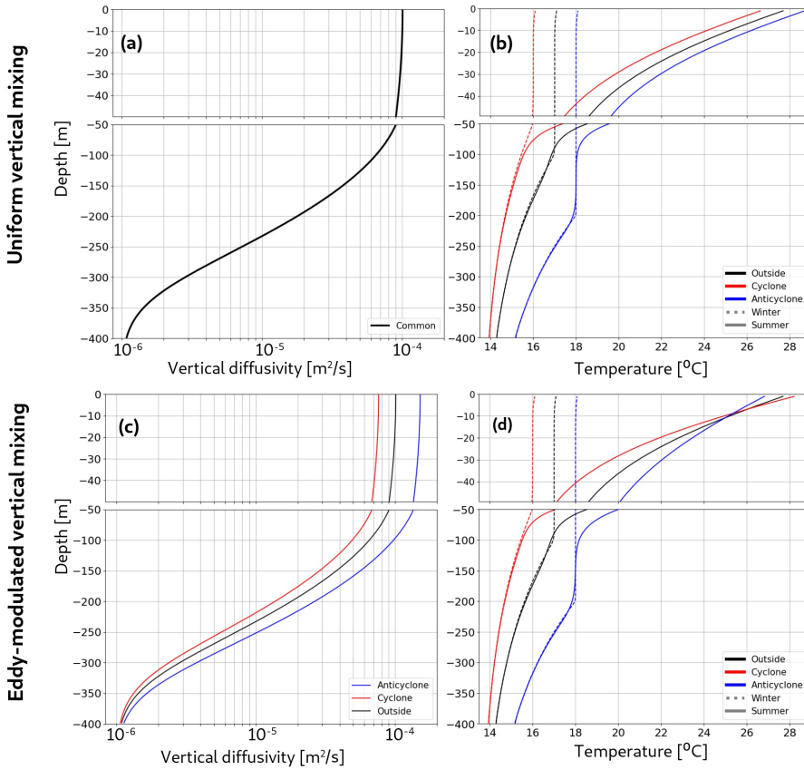
Figure I.10: 1D single column experiments : vertical structure. With a uniform vertical mixing : (a) vertical diffusivity A(z) from equation I.5, and (b) temperature profiles in winter (dashed line) and summer (continuous line), corresponding time of the year being reported on Fig.I.11b . Initial winter profiles are set in equation I.3. With eddy-modulated vertical mixing : (c) vertical diffusivity and (d) temperature profiles.
