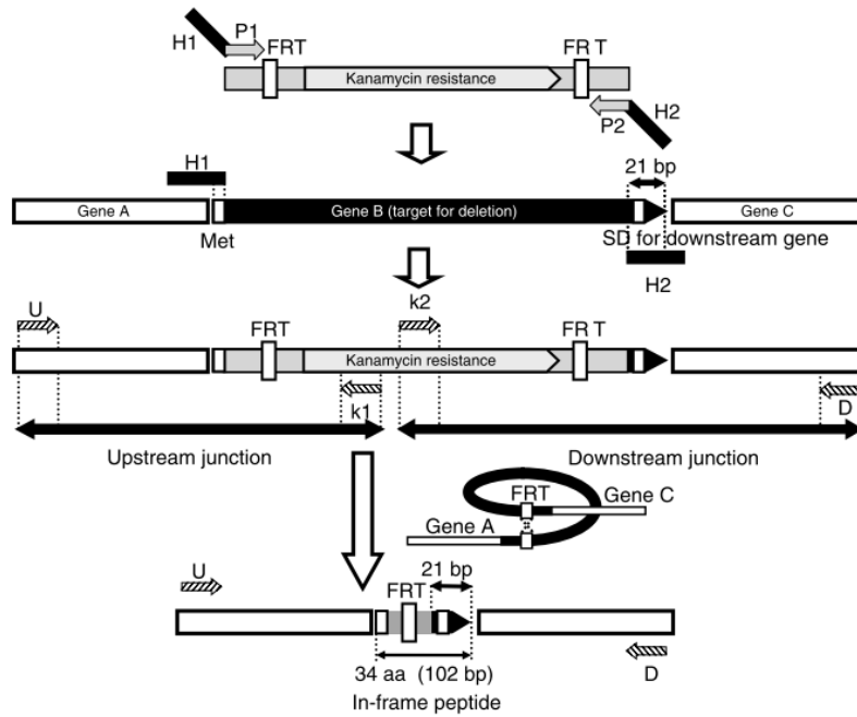
Figure 10: Figure from Baba et al. [72]. In the first step, the gene to be deleted is replaced with a kanamycin resistance gene flanked by two FRT sites. Novel junctions created between the resistance cassette and neighboring upstream (gene A) and downstream (gene C) sequences can be verified by PCR with kanamycin (k1 or k2) and locus-specific (U or D) primers. In a second step, the cassette can be removed using FLP recombinase. This leaves a 102 bp scar sequence.
