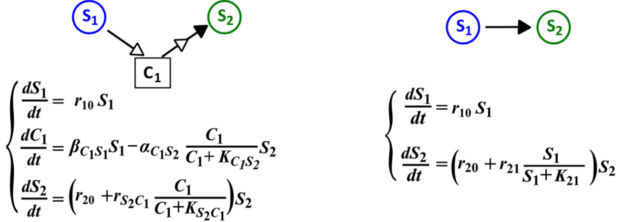
Figure 1: The difference between Lotka-Volterra models (right) and models with explicit resources (left). Adapted from [27]. Species S_1 releases chemical C_1 . C_1 is consumed by species S_2 and promotes S_2 's fitness. Both species have a basal growth rate ( r_{10} and r_{20} ). In the mechanistic model, the growth rate of S_2 is positively impacted by the chemical C_1 , whereas in the L-V model, S_2 is directly influenced by S_1 .
