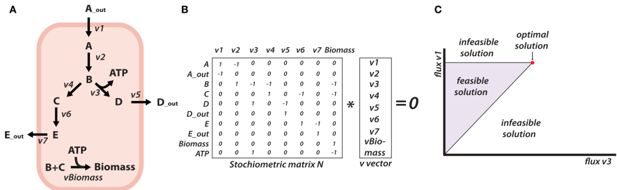
Figure 2: Taken from [36]. Constraint-based modeling of a micro-organism. (A) The microorganism takes up metabolite A and produces biomass, and products D and E. (B) The stoichiometric matrix N representing the network depicted in A, with rows corresponding to metabolites and columns to fluxes. The stoichiometric matrix multiplied with the flux vector is in steady-state. (C) The biomass flux is optimized to find the optimal flux distribution.
