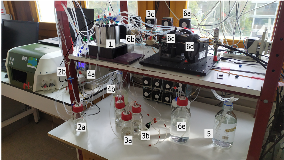
Figure 13: Picture of the mini-bioreactor platform. 1) Bioreactors 2a) KOH solution to sterilize the incoming air 2b) 0.22\ \mu\text{m} filter to sterilize the incoming air 3a) Medium storage bottle 3b) KOH to sterilize air entering the medium storage bottles 3c) Pumps transporting medium to the bioreactors 4a) Pump removing culture from the bioreactors 4b) Waste container 5) KOH sterilizing the air leaving the bioreactors 6a) Pumps transporting samples 6b) Selection valve selecting the chosen bioreactor to be sampled 6c) Measurement cuvette 6d) Filter wheel to select input and output wavelength for the fluorescence measurements 6e) Water container for water samples
