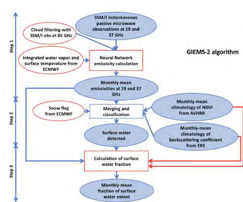
Figure 3-8. Schematic presentation of the GIEMS-2 algorithm. In red, the changes from GIEMS methodology (Prigent et al., 2020).
