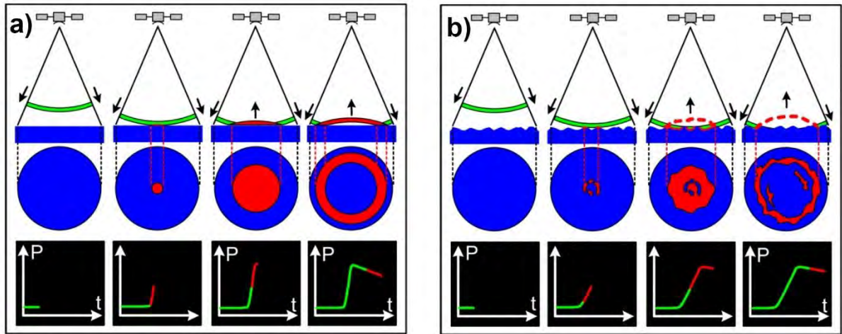
Figure 2-9. Representation of a reflected waveform of conventional altimetry echo. At the top, a representation of the satellite and emitted wave, with the reflected wave in red. In the middle, the behavior of the wave on a smooth surface (a) and rough surface (b). At the bottom, the waveform received by the altimeter (Calmant et al., 2008).
