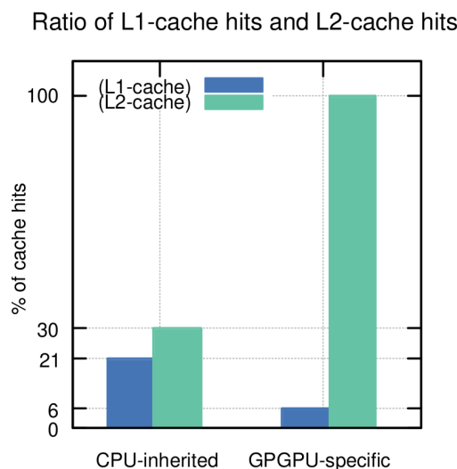
Figure 1.9. Relative amount of L1-cache and L2-cache hits for kernels running on the Tesla V100: The GPU parallel implementation is designed to maximize the L2-cache reuse.
