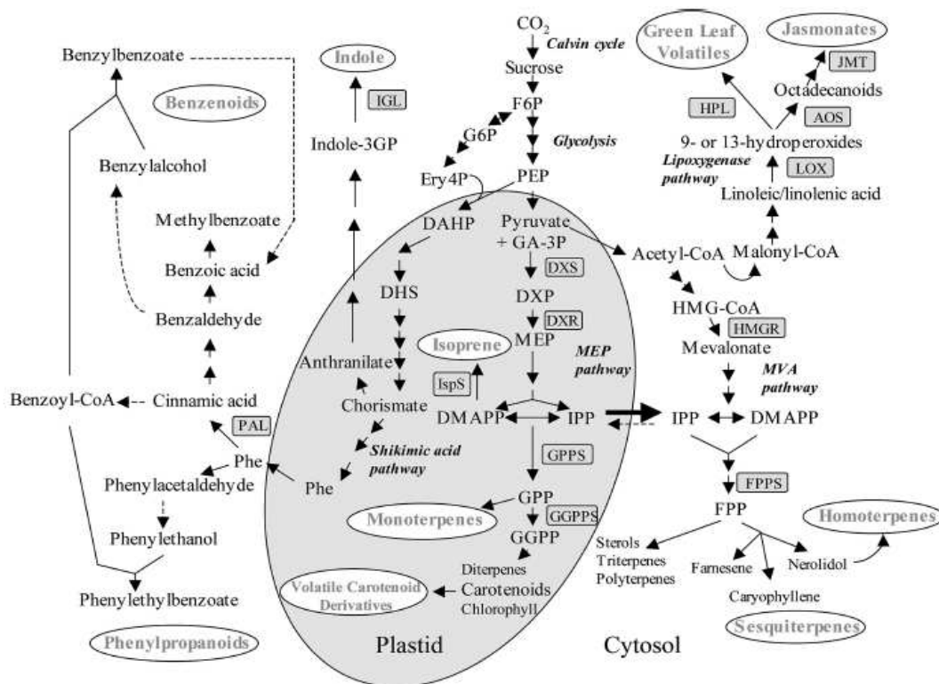
FIG. 2. Metabolic pathways leading to the biosynthesis of various volatile compounds in plants. Pathway names are italicized, volatile compounds are in bold and enzymes are boxed. Abbreviations: Acetyl-CoA, acetyl coenzyme-A; AOS, allene oxide synthase; DAHP, 3-deoxy-D-arabino-heptulosonate 7-phosphate; DHS, 3-dehydroshikimic acid; DMAPP, dimethylallyl diphosphate; DXP, 1-deoxy-D-xylulose 5-phosphate; DXR, DXP reductoisomerase; DXS, DXP synthase; Ery4P, erythrose 4-phosphate; F6P, fructose 6-phosphate; FPP, farnesyl diphosphate; FPPS, FPP synthase; GA-3P, glyceraldehyde-3-phosphate; G6P, glucose 6-phosphate; GGPP, geranylgeranyl diphosphate; GGPPS, GGPP synthase; GPP, geranyl diphosphate; GPPS, GPP synthase; HMG-CoA, 3-hydroxy-3-methylglutaryl-CoA; HMGR, 3-hydroxy-3-methylglutaryl-CoA reductase; HPL, fatty acid hydroperoxide lyase; IGL, indole-3-glycerol phosphate lyase; Indole-3GP, indole 3-glycerol phosphate; IPP, isopentenyl diphosphate; JMT, jasmonic acid carboxyl methyl transferase; LOX, lipoxygenase; MEP, 2-C-methyl-D-erythritol 4-phosphate; MVA, mevalonate; PAL, phenylalanine ammonia lyase; PEP, phosphoenolpyruvate; Phe, phenylalanine.
