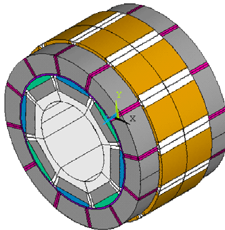
figure IV.3 : structure globale Aximag
