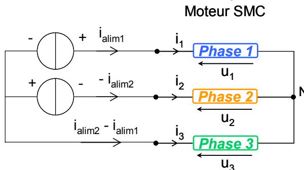
Circuit 2
