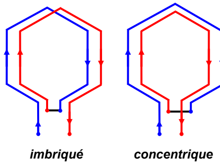
figure II.4 : dispositions possibles des spires.
