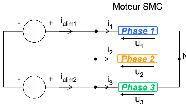
Circuit 1
