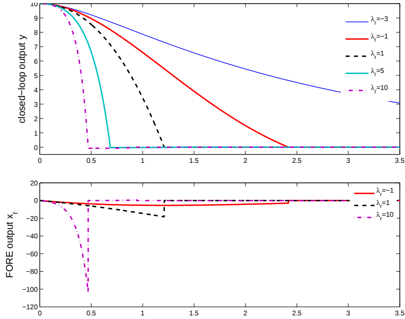
Figure 2.8: Top: Output of the closed-loop system. Down: Output of the FORE for different values of \lambda_r .
