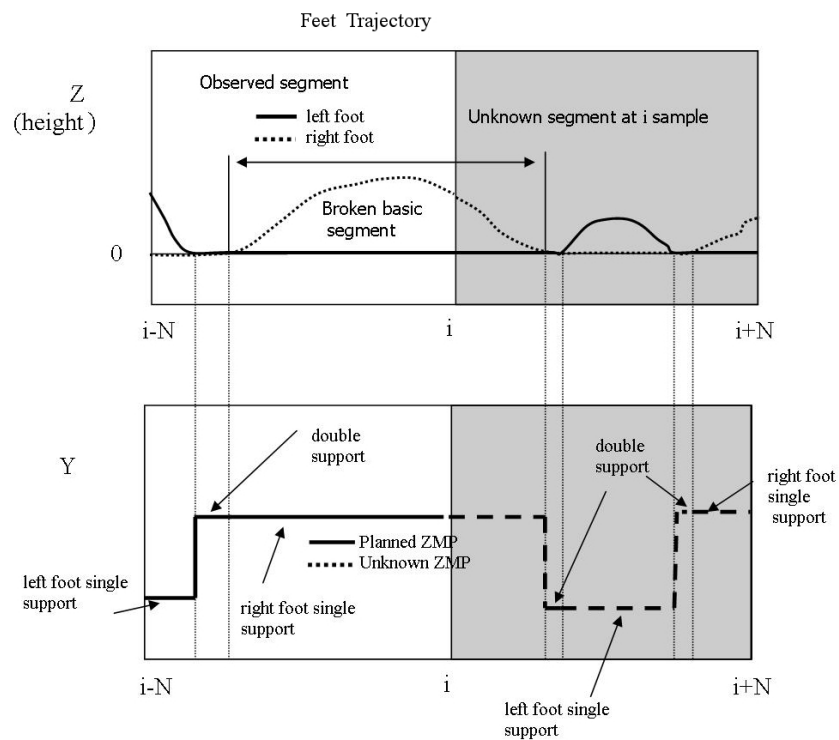
Figure 5.12: Planning the ZMP trajectory from the feet positions. To plan the ZMP it is only required the the position of the last landing foot. Attention must be made on the feet height, they determines when the ZMP must be changed.
