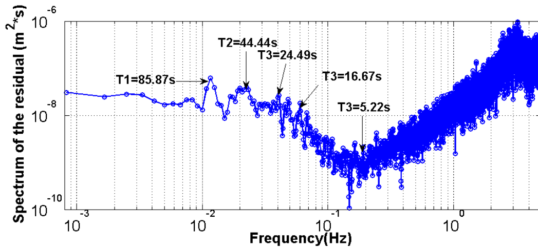
Fig. 10-50 Fourier spectrum function with the respect to the frequency of the residual of H_6(t) with differential filtering
