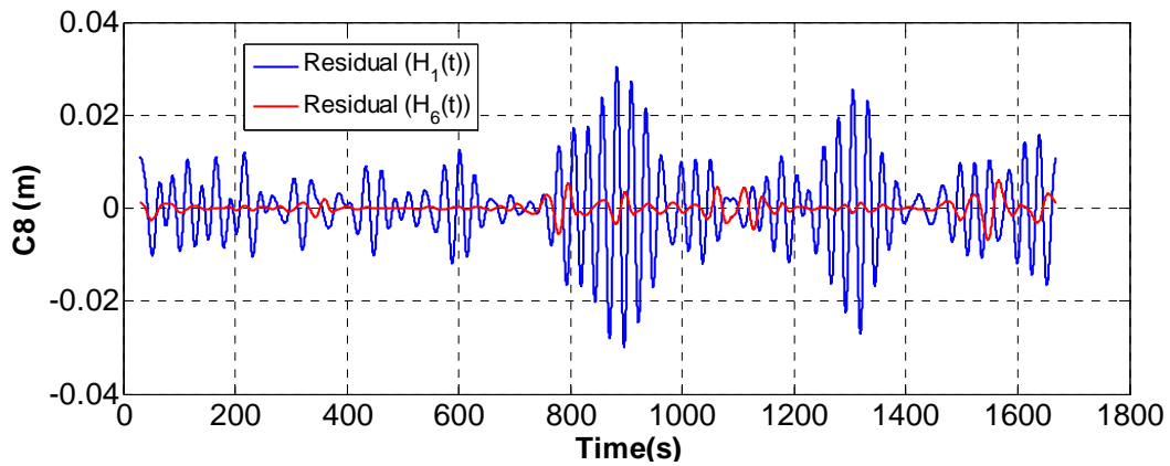
Fig. 10-83 Evolution of the dyadic wavelet component C_8 of the residuals of H_1(t) and H_6(t) with moving average filtering ( wt_1=5s et wt_6=30s , t=0-1800s )
