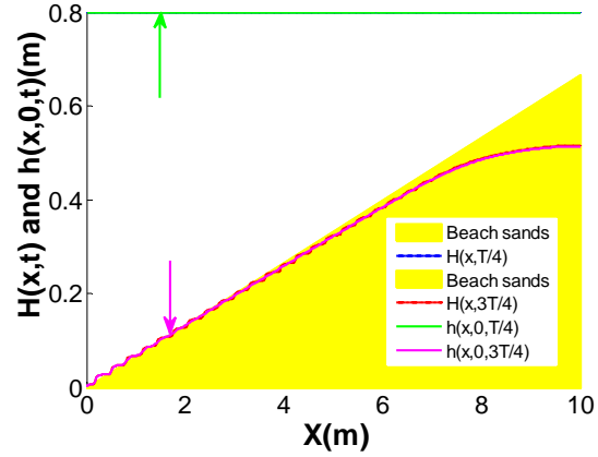
Fig. 11-18 Comparison of the pressure head h(x,0,t) and the free surface h(x,z,t)=0.0 at t=T/4 and t=3T/4
