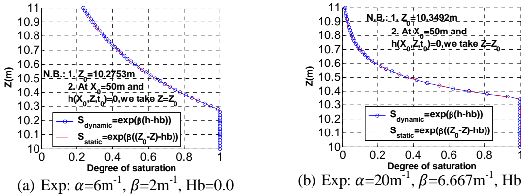
Fig. 3-46 Comparison of the instantaneous static curve and the computed dynamic curve of the degree of saturation at t=10 hours at X_0=50\text{m} with partially saturated Richards model in the case of the exponential model parameters: (a) \alpha=6\text{m}^{-1} , \beta=2\text{m}^{-1} , H_b=0.0 ; (b) \alpha=20\text{m}^{-1} , \beta=6.667\text{m}^{-1} , H_b=0.0 .
