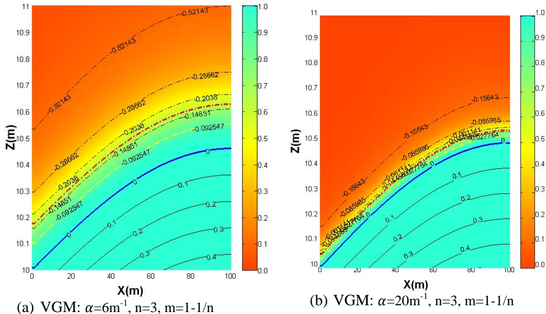
Fig. 3-47 Vertical profile of the instantaneous distributions of the pressure head h(x, z, t_0) and the degree of saturation S(x, z, t_0) at t=10 hours with partial saturated Richards model in the case of VGM parameters: (a) \alpha=6\text{m}^{-1} , n=3 , m=1-1/n ; (b) \alpha=20\text{m}^{-1} , n=3 , m=1-1/n Note: 1. in the figure (a), the red curve ( h=-0.17\text{m} ) corresponds to S=0.63 and the yellow curve ( h=-0.09\text{m} ) corresponds to S=0.9 ; 2. in the figure (b), the red curve ( h=-0.05\text{m} )
