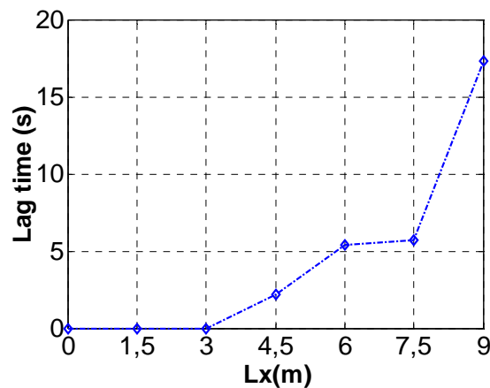
Fig. 12-19 Lag time corresponding to the maximum cross-correlation between H_1(t) and H_i(t) ( i = 2, \dots, 7 ) with respect to the horizontal distance of the sensor position from the sensor No.1 ( Original signal )
