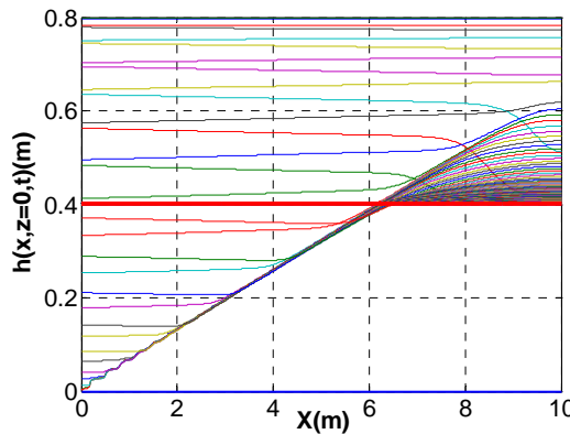
Fig. 11-19 Profile of the evolution of the horizontal line pressure head at z=0 h(x,z=0,t) or the water level fluctuations H(x,t) (time interval= 10 dt=1.0s )
