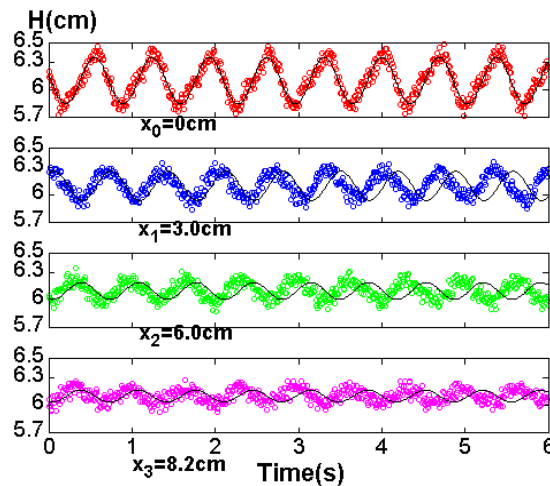
Fig. 4-5 Time evolution of measured water levels H(x,t) (symbols) and the corresponding theoretical values (solid curves) at different locations in the sandbox: x_0=0.0 , x_1=3.0 , x_2=6.0\text{cm} , x_3=8.2\text{cm} (period T=0.6896\text{s} , amplitude A_0 = 0.2521 \text{ cm} ).
