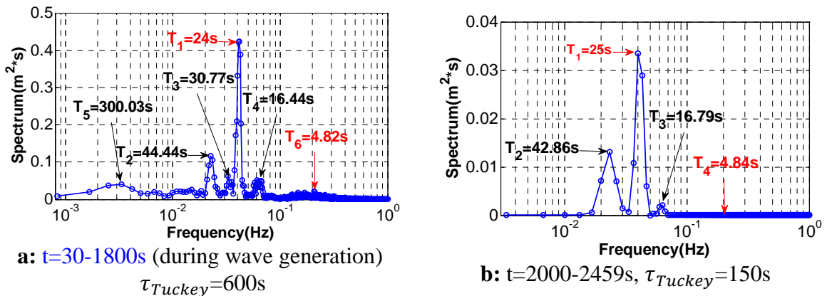
Fig. 6-4 Fourier frequency spectrum of the water level fluctuations H_1(t) for two different time windows (during and after wave generation).
