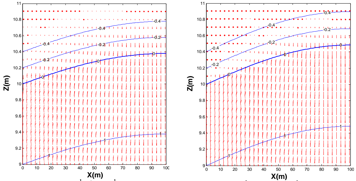
Fig. 3-50 Vertical profile of the instantaneous flux field q(x, z, t_0) and pressure head h(x, z, t_0) contours at t=10 hours with partial saturated Richards model in the case of exponential model parameters: (a) \alpha=6\text{m}^{-1} , \beta=2\text{m}^{-1} , H_b=0.0 ; (b) \alpha=20\text{m}^{-1} , \beta=6.667\text{m}^{-1} , H_b=0.0 . Note: \beta = \alpha / 3 and \text{Scale}_{\text{flux}}=0.7 .
