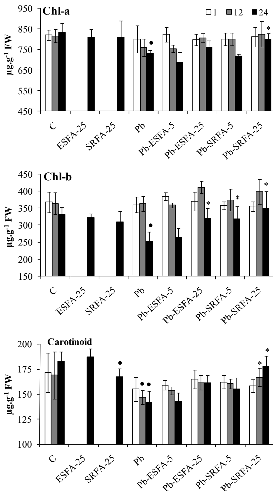
Fig-3. Effect of SRFA and ESFA on Pb-induced reduction of pigment contents ( \mu\text{g.g}^{-1} FW) in V. faba leaves. Values are means of two separate experiments each replicated six times. An asterisk (*) indicates significant differences at P < 0.05 for Pb-FA treatments compare
