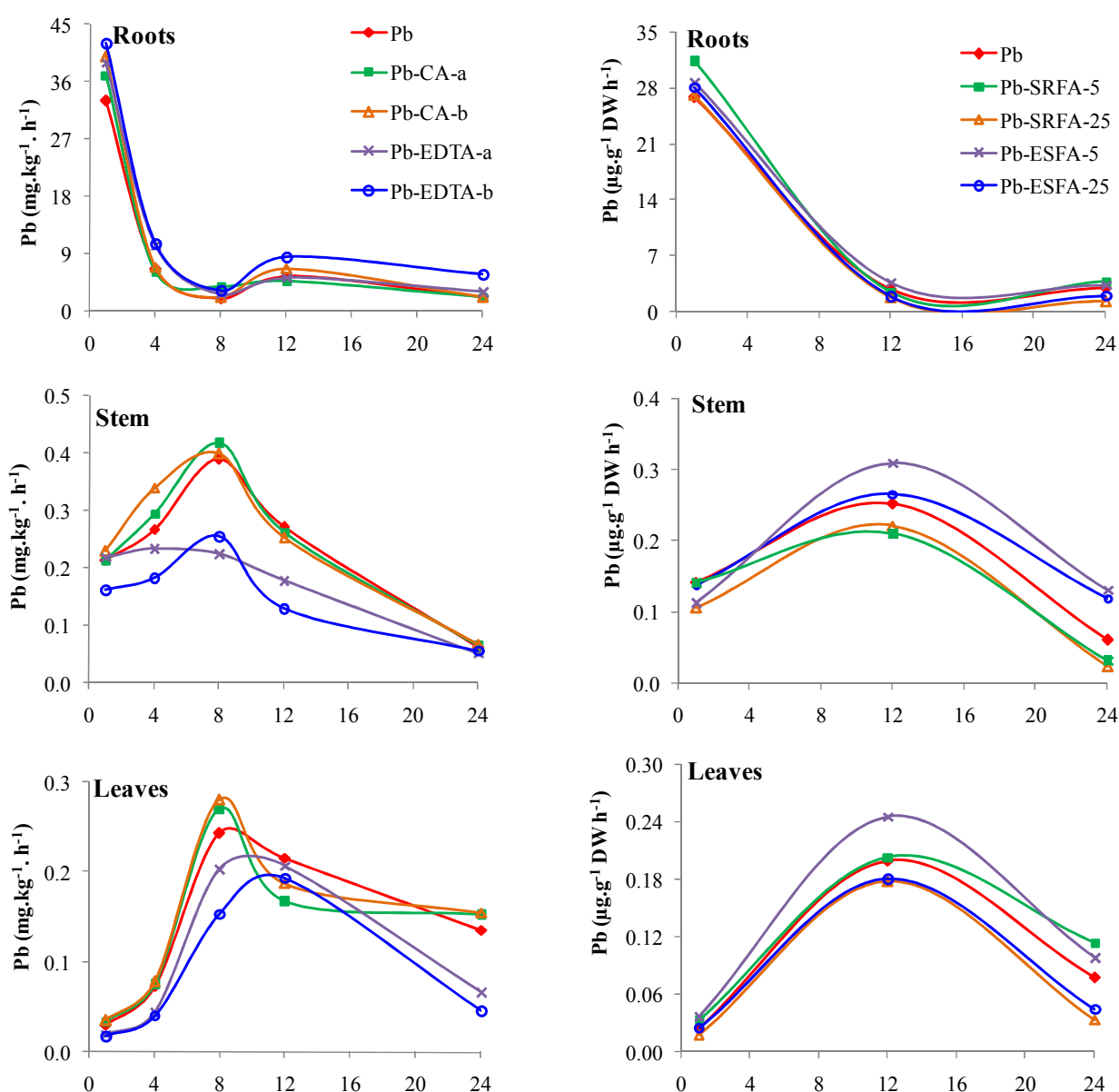
Fig-1. Effect of organic ligands on Pb kinetic uptake and translocation by Vicia faba .
