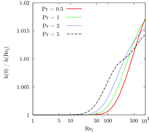
Figure II.9: Evolution of the ratio h(0) in the pure diffusive case over h(Re_\ell)
