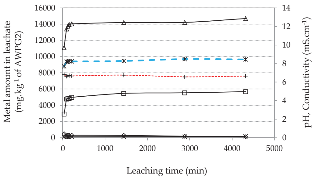
Figure 77 : Leachability of calcium, phosphorus, sulfur and strontium from AWPG2 formulation ( -\diamond- Phosphorus, -\square- Calcium, -\Delta- Sulfur, -\times- Strontium, -\text{+}- pH and -\text{*}- conductivity ( \text{mS.cm}^{-1} ))
