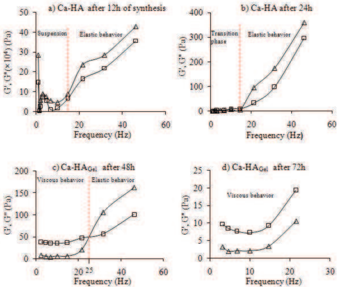
Figure 50: Frequency-sweep curves of Ca-HA as a function of synthesis time ( \text{---}\Delta\text{---} , storage modulus G' , \text{---}\square\text{---} loss modulus G'' ). The description of the behavior of Ca-HA Gel is based on two conditions if G' > G'' , elastic behavior, and if G' < G'' , the behavior is viscous.
