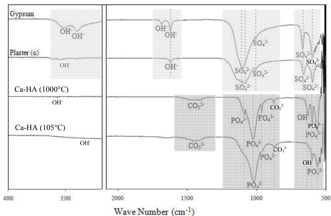
Figure 33: FTIR of gypsum, plaster, Ca-HA dried at 105°C (24h) and Ca-HA calcined at 1000°C
