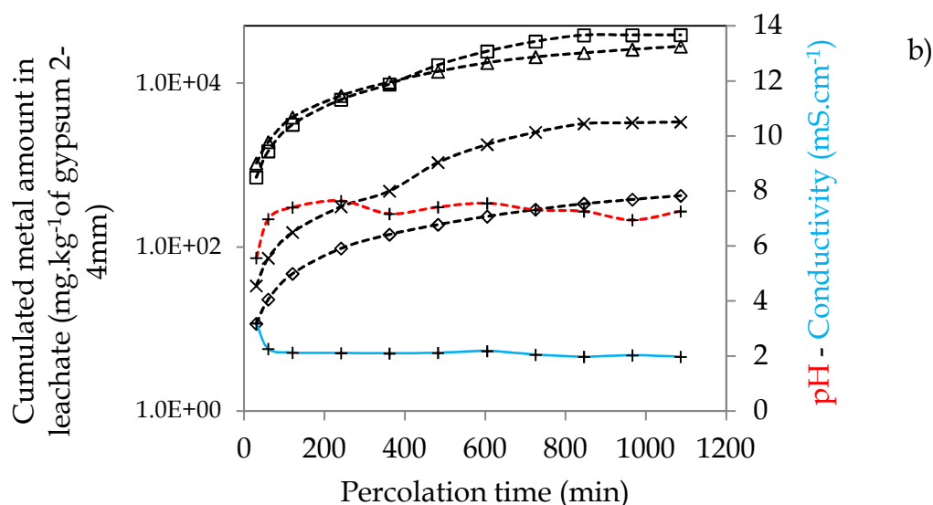
Figure 89: Leached amount of calcium (---□---), phosphorus (---◇---), sulfur (---Δ---) and strontium (---×---) from column percolation test of gypsum (1-2mm) (a) and gypsum (2-4mm) (b) in function of leaching time, pH (---+---) and conductivity (---+---)
