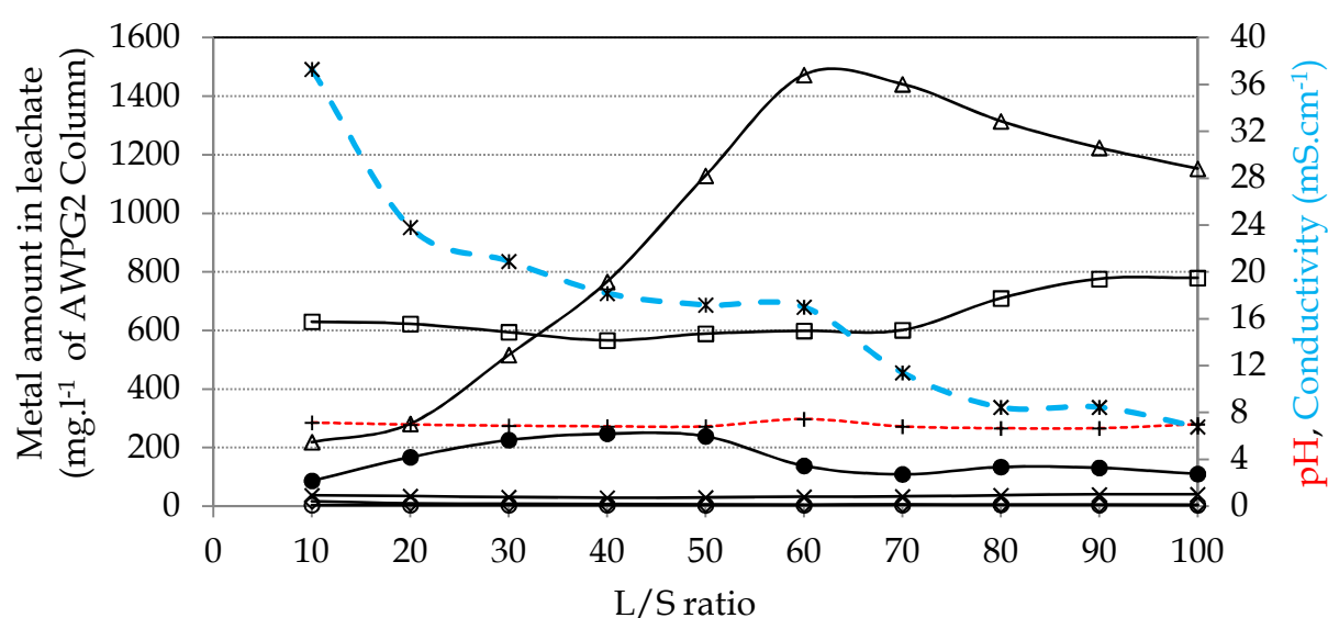
Figure 97 : Concentration of calcium (—□—), phosphorus (—◇—), sulfur (—Δ—), strontium (—×—), lead (—○—) and cadmium (—●—) in the filtrate at different L/S mass ratio (pH (—+—) and conductivity (—+—))
