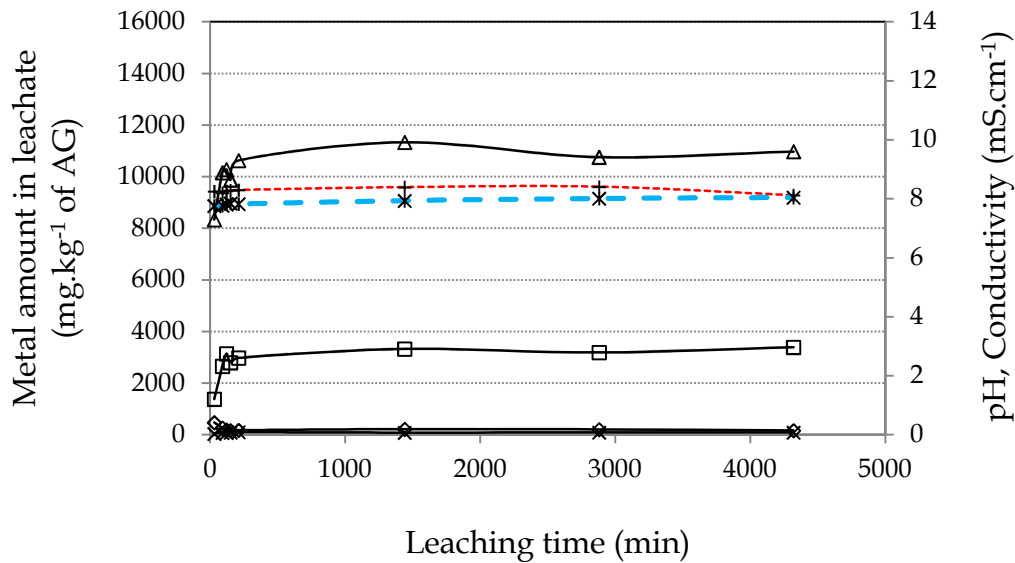
Figure 75 : Leachability of calcium, phosphorus, sulfur and strontium from AG formulation (—◇— Phosphorus, —□— Calcium, —△— Sulfur, —×— Strontium, --+-- pH and --*-- conductivity (mS.cm -1 ))
