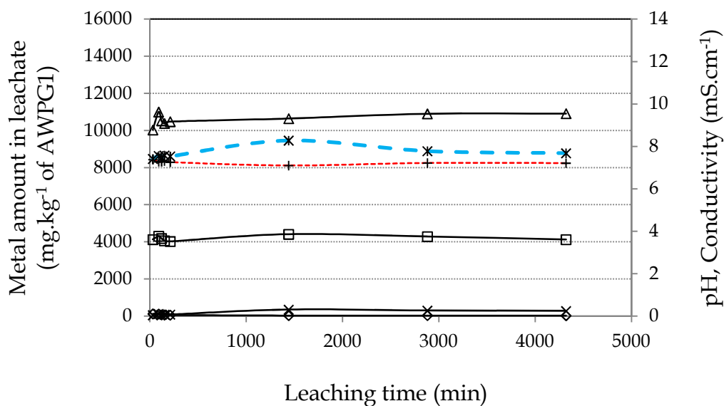
Figure 76 : Leachability of calcium, phosphorus, sulfur and strontium from AWPG1 formulation (—◇— Phosphorus, —□— Calcium, —△— Sulfur, —×— Strontium, -+--- pH and -*--- conductivity ( \text{mS.cm}^{-1} ))
