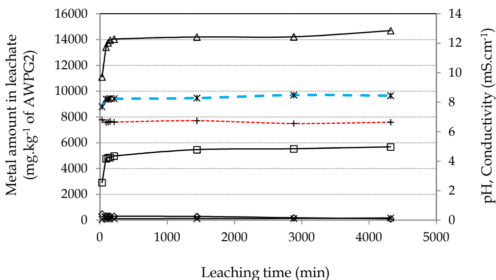
Figure 77 : Leachability of calcium, phosphorus, sulfur and strontium from AWPG2 formulation (—◇— Phosphorus, —□— Calcium, —△— Sulfur, —×— Strontium, -+--- pH and -*--- conductivity ( \text{mS.cm}^{-1} ))
