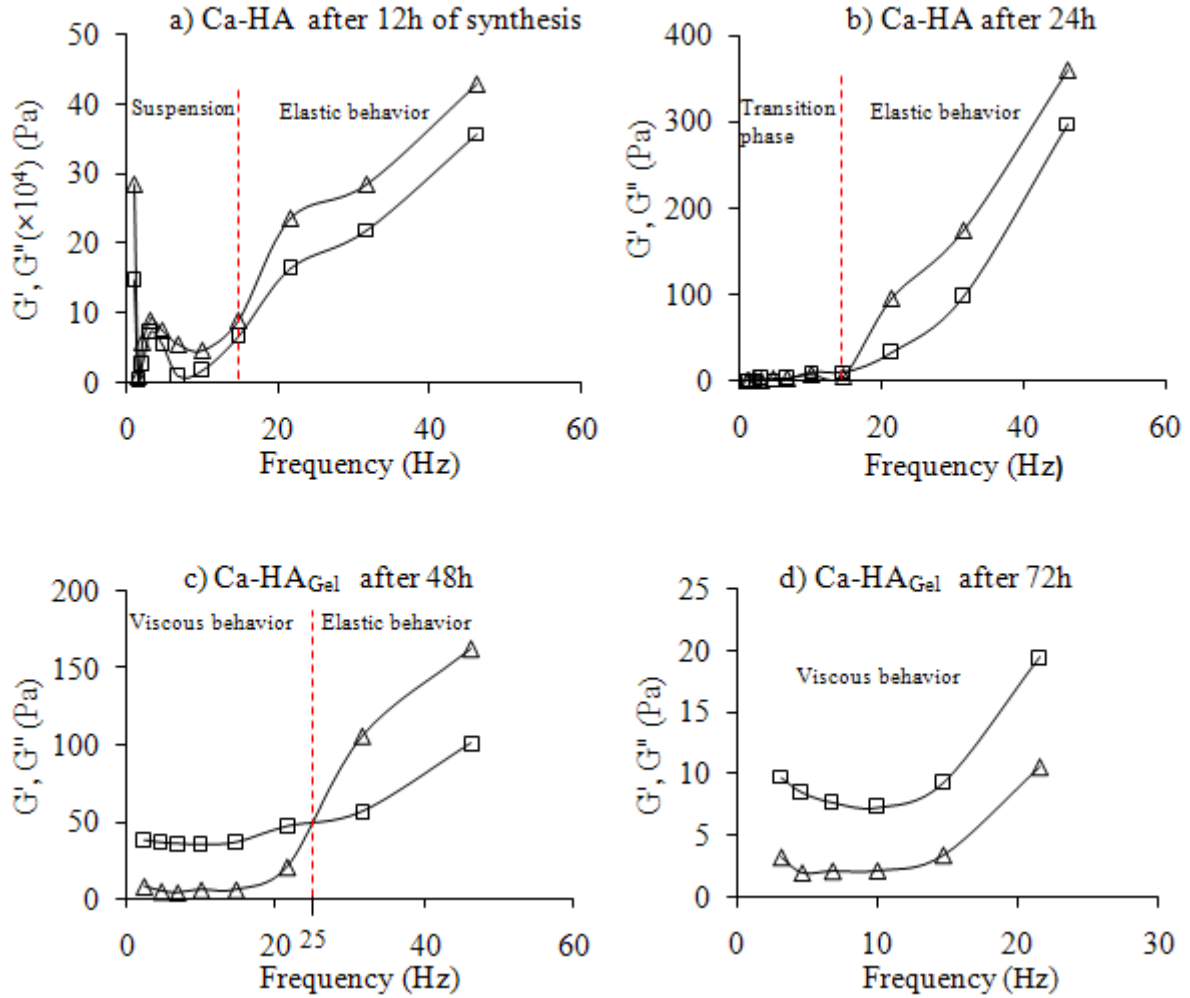
Figure 50: Frequency-sweep curves of Ca-HA as a function of synthesis time ( \triangle , storage modulus G' , \square loss modulus G'' ). The description of the behavior of Ca-HA Gel is based on two conditions if G' > G'' , elastic behavior, and if G' < G'' , the behavior is viscous.
