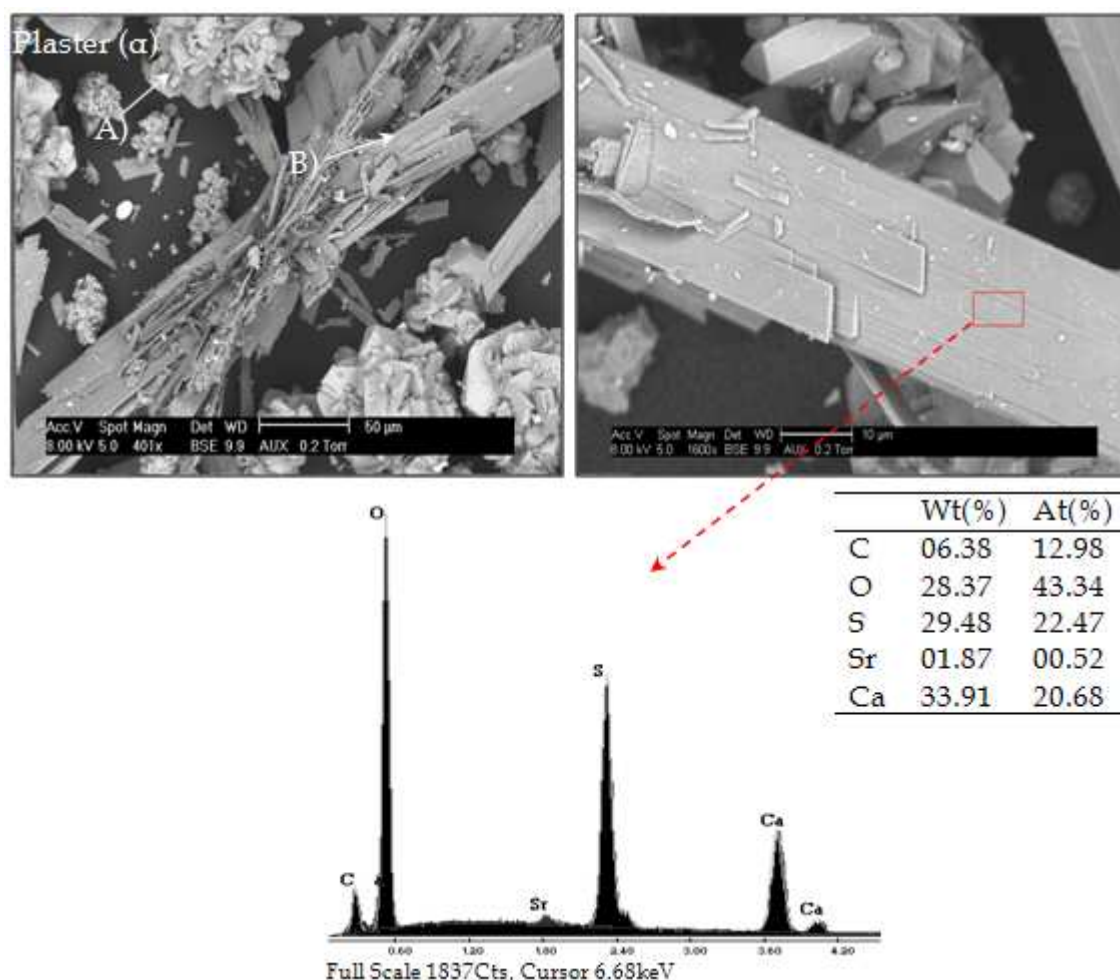
Figure 18 : SEM pictures of plaster ( \alpha ) (10-50 \mu m)
