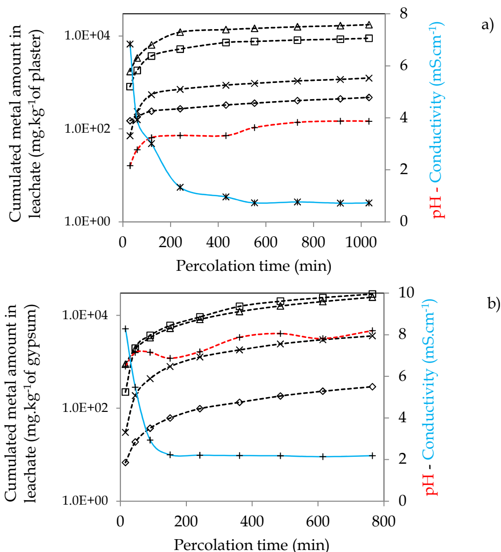
Figure 88: Leached amount of calcium (---□---), phosphorus (---◇---), sulfur (---△---) and strontium (---×---) from column percolation test of plaster (a) and gypsum (<1mm) (b) in function of leaching time, pH (---+---) and conductivity (---+---)
