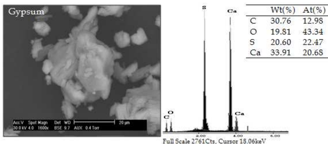
Figure 19 : SEM picture and EDS analysis corresponding to gypsum (<1mm) (20µm)
