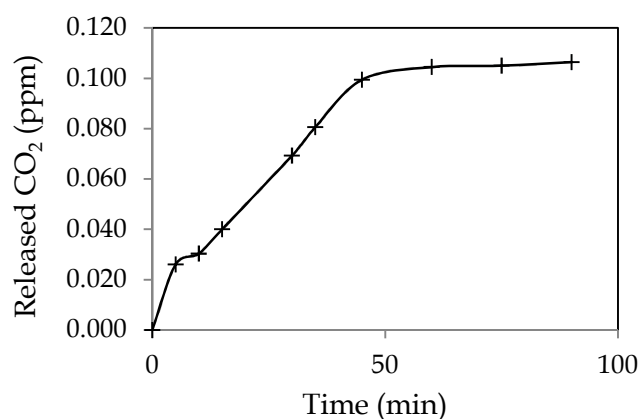
Figure 48 : Amount of released \text{CO}_2 as a function of time
