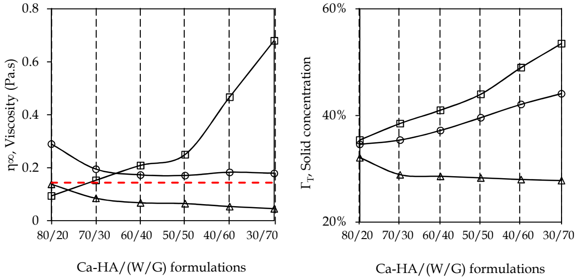
Figure 55: Variation of viscosity of Ca-HA/(W/G) mixtures at different mass ratios (— \text{Ca-HA}_{\text{Gel}} (0.144Pa.s), —□— \text{Ca-HA}/(\text{W/G}=0.2) , —○— \text{Ca-HA}/(\text{W/G}=0.4) , —Δ— \text{Ca-HA}/(\text{W/G}=0.6) )
