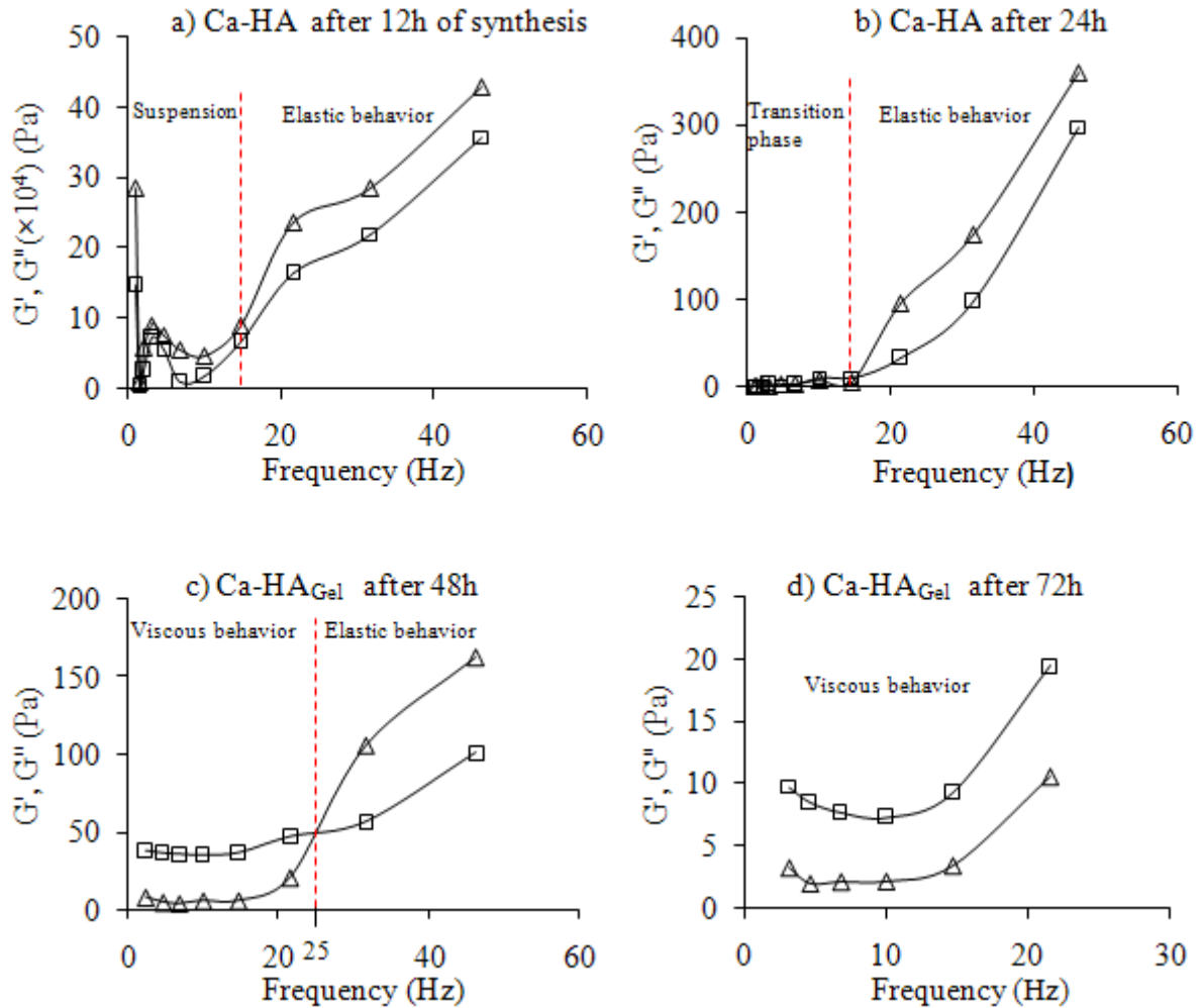
Figure 50: Frequency-sweep curves of Ca-HA as a function of synthesis time ( \triangle , storage modulus G' , \square loss modulus G'' ). The description of the behavior of \text{Ca-HA}_{\text{Gel}} is based on two conditions if G' > G'' , elastic behavior, and if G' < G'' , the behavior is viscous.
