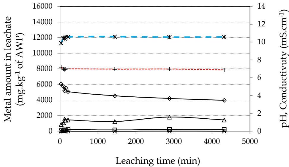
Figure 74: Leachability of calcium, phosphorus, sulfur and strontium from AWP formulation ( -\diamond- Phosphorus, -\square- Calcium, -\Delta- Sulfur, -\times- Strontium, -\text{+}- pH and -\text{*}- conductivity ( \text{mS.cm}^{-1} ))
