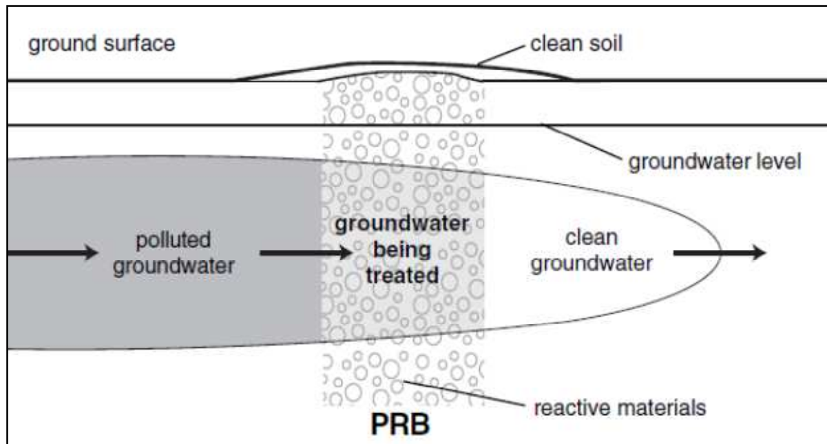
Figure 1: PRB general concept [8]
