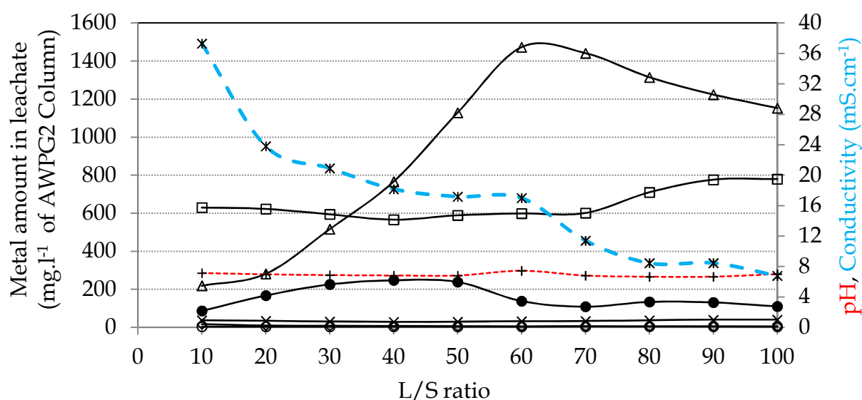
Figure 97 : Concentration of calcium (—□—), phosphorus (—◇—), sulfur (—△—), strontium (—×—), lead (—○—) and cadmium (—●—) in the filtrate at different L/S mass ratio (pH (—+—) and conductivity (—+—))
