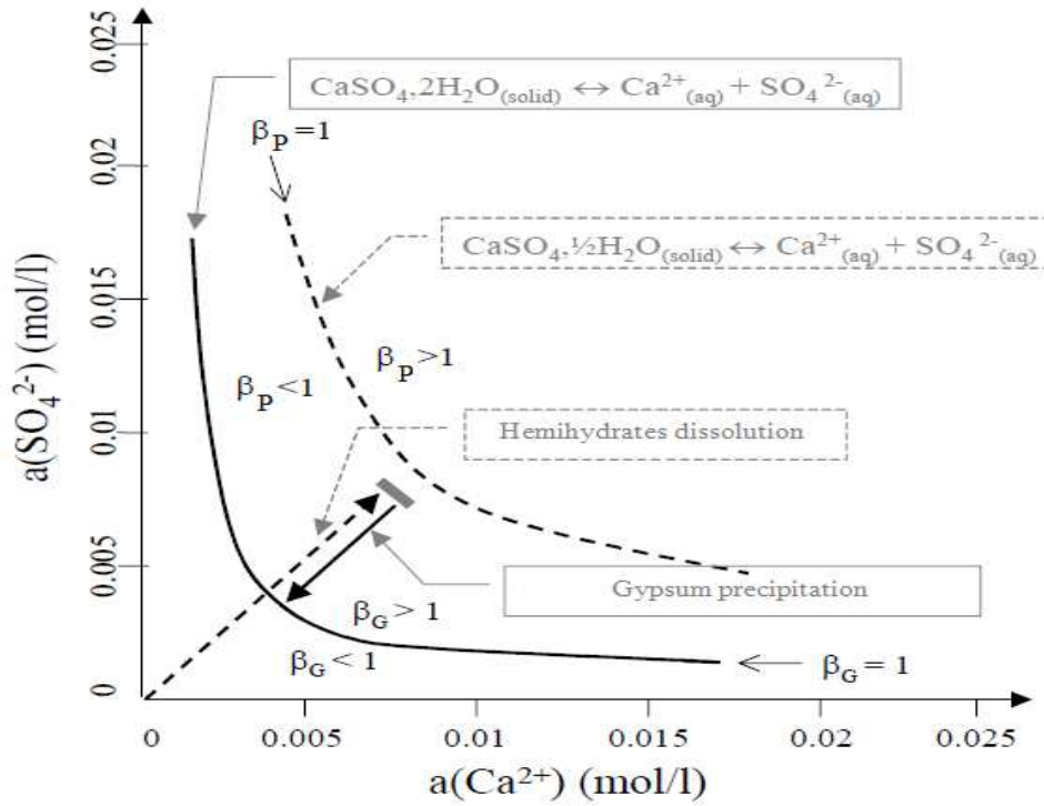
Figure 34: Diagram of calcium sulfate solubility [1]
