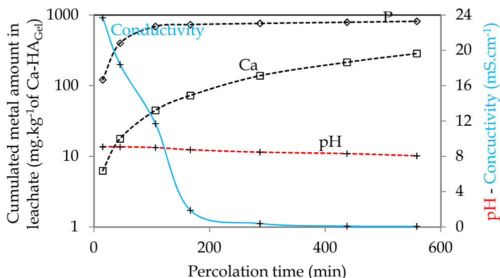
Figure 87: Leached amount of calcium and phosphorus from Ca-HA as a function of leaching time, pH and conductivity (—◇— Phosphorus, —□— Calcium, ---+--- pH and ---+--- conductivity ( \text{mS.cm}^{-1} ))
