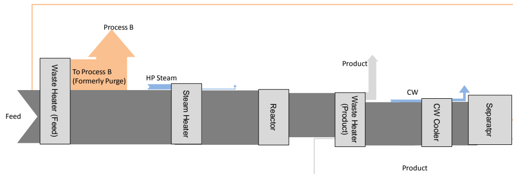
Figure 3.23. Grassmann diagram (integrated case)
