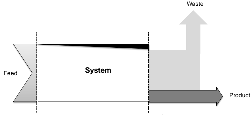
Figure 3.28. Grassmann diagram for the splitter
