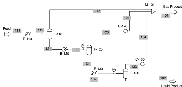
Figure 4.7. Natural gas stabilization (Montelongo-Luna et al., 2007)
