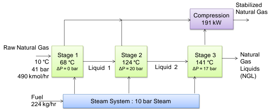
Figure 5.1. Block diagram of the NGL recovery process
