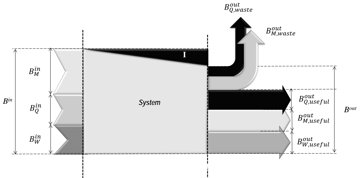
Figure 3.1. A General Grassmann representation of a process or system
