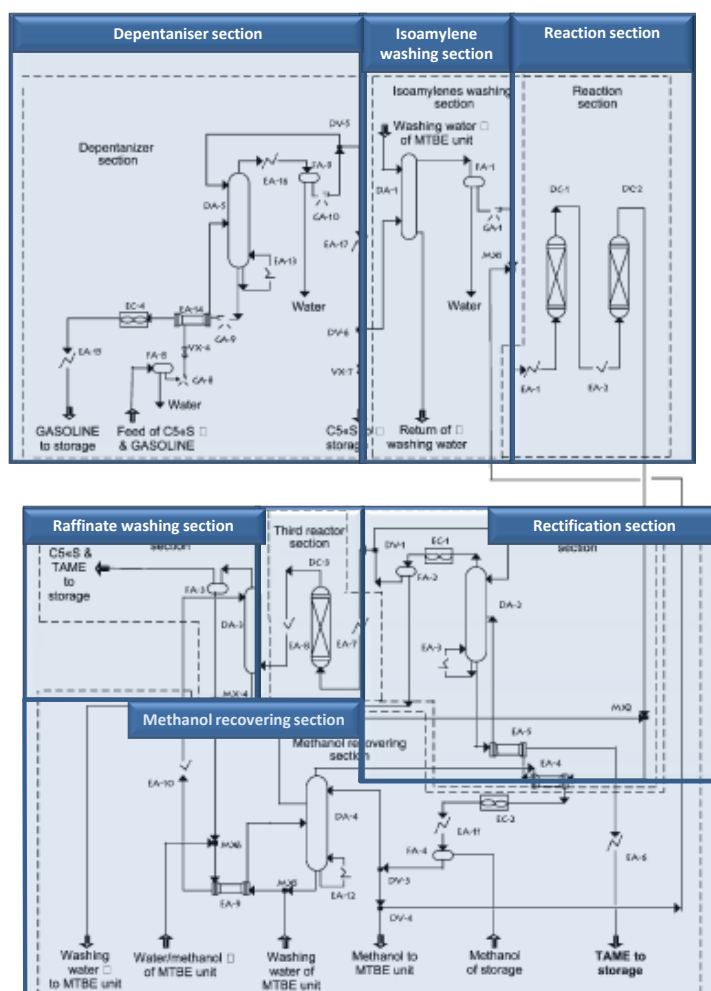
Figure 3.42. Decomposition of the process into functional zones
