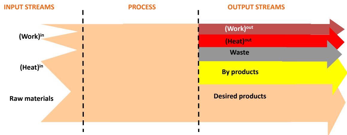
Figure 2.2. Energy balance
