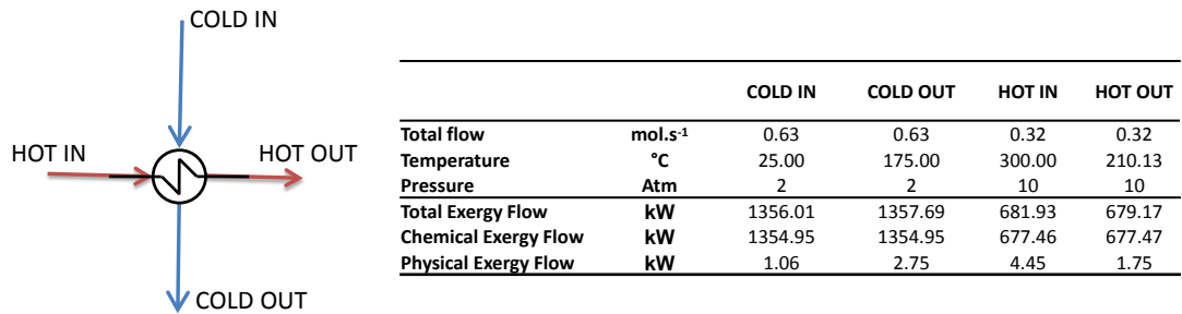
Figure 3.32. Two-stream heat exchanger
