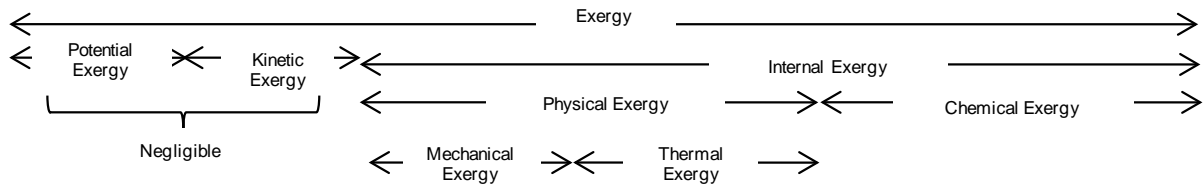
Figure 2.5. Exergy components
