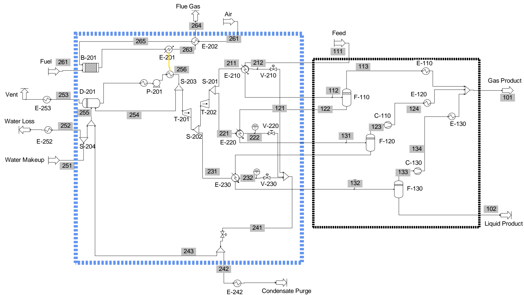
Figure 5.11. Improved process & utility flowsheet
