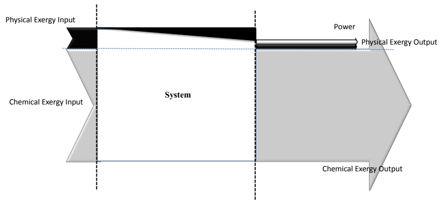
Figure 3.31. Grassmann diagram for expansion of propane
