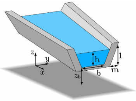
Fig. 3: Venturi flume parameters.
