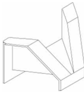
Figure 1.6: H flume
