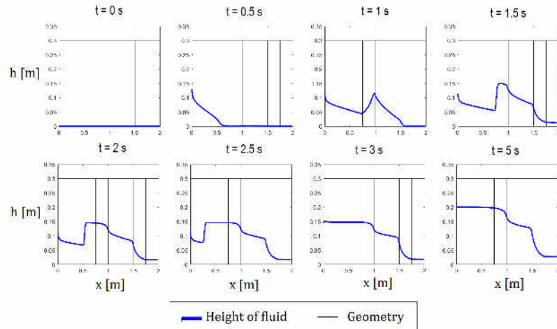
Figure 4.8: Capture at different time of a water flow along the trapezoidal Venturi flume for Q = 500\text{L/min} with the 1D transient model
