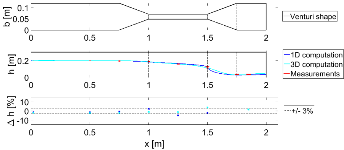
Figure 6.13: Exp. vs. 3D vs. 1D for a glycerin flow with \mu = 0.205 Pa.s , \rho = 1237.5 Kg/m^3 and Q = 244.5 L/min
