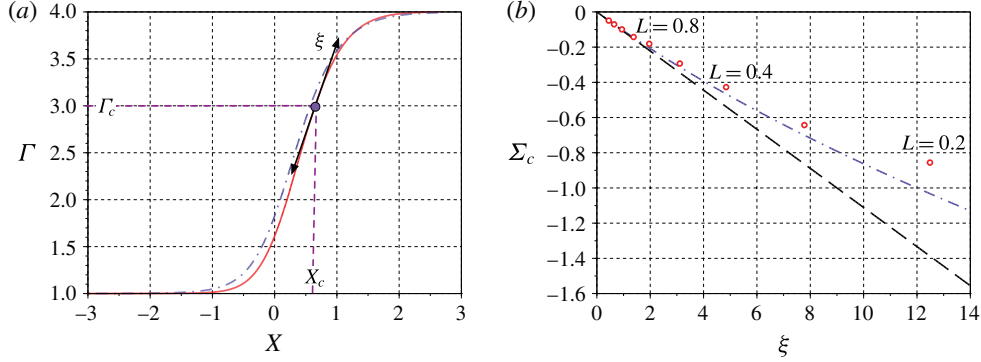
FIGURE 7. Slope \Gamma(X) such that h(X) = \bar{h} + \Delta h \tanh(X/L) is the critical backwater curve in the cases \Gamma_1=1 and \Gamma_2=4 . (a) Comparison between the TLM (plain red) and the STL (dash-dotted blue) for L=0.8 . (b) Critical surface slope \Sigma_c = h'(X_c) as a function of the bottom curvature \xi = \Gamma'(X_c) for L = 2^{k/2}/10 and k = 2, 3, \dots, 11 . Comparison with the theoretical functions for the STL (dash-dotted blue) and the NOR (dashed black) models.
