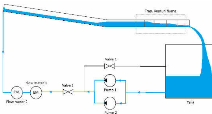
Figure 2.10: Flow loop with high flow rate, the valve 1 is closed and the 2 pumps are turned on
