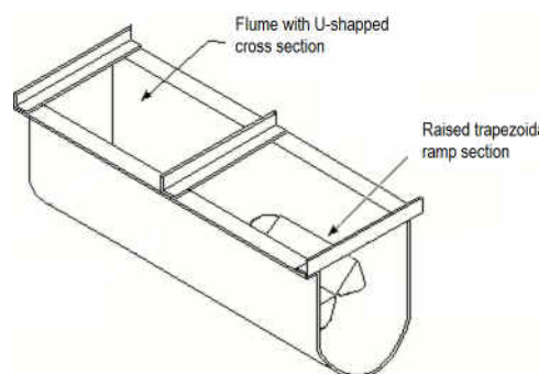
Figure 1.5: Palmer-Bowlus flume
