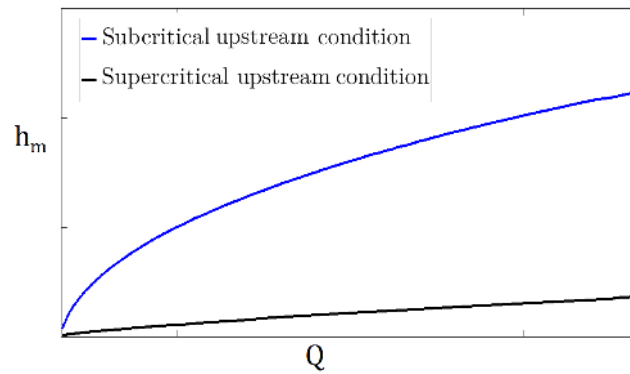
Figure 4.3: Qualitative relation between h_m and Q for subcritical and supercritical upstream condition for a trapezoidal Venturi flume
