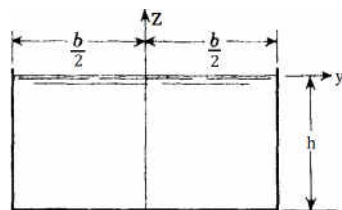
Figure 5.10: Rectangular channel
