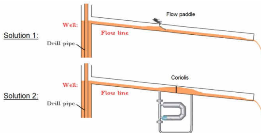
Figure 1.12: Flow paddle (solution 1) and Coriolis (solution 2) sensors installed in return lines
