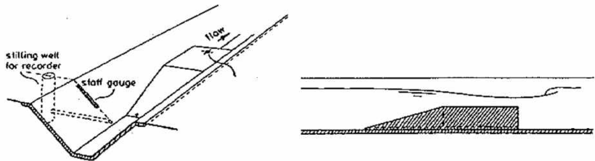
Figure 1.10: RBC flume
