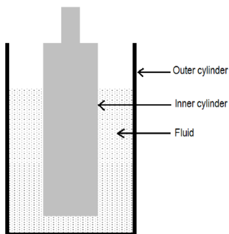
Figure 2.2: Couette geometry of the rheometer RheolabQC
