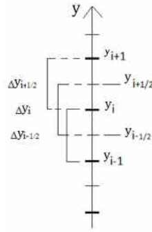
Figure 5.6: Vertical mesh and associated space steps
