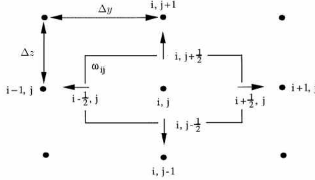
Figure 5.9: Control volume
