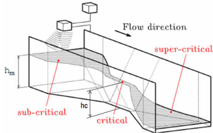
Figure 1.1: Venturi flume
