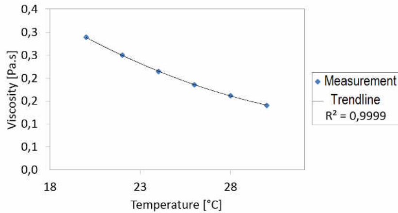
Figure 2.4: Trendline of the viscosity and temperature of the mixture with 90% of glycerin
