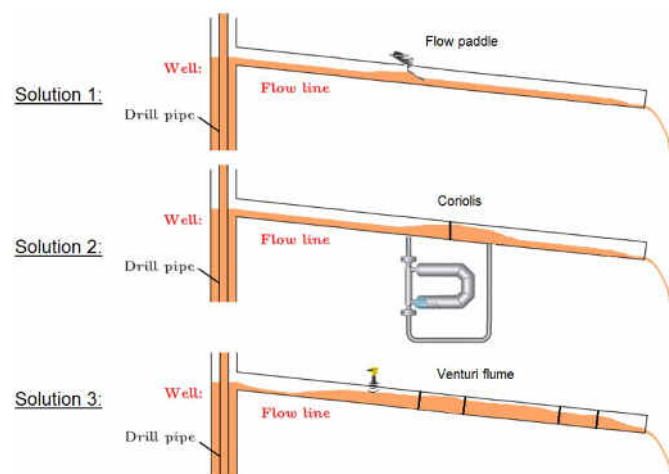
Fig. 1: Solution to measure the flow out the well.
