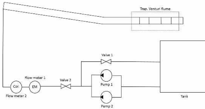
Figure 2.8: Empty flow loop
