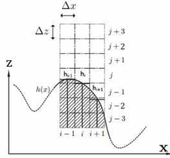
Figure 6.6: Illustration of the HF method to compute the height of the free surface
