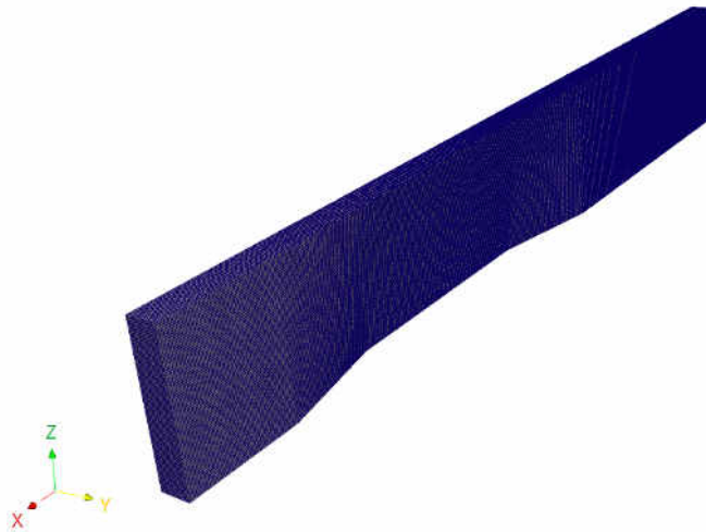
Figure 3.2: Mesh for the Trapezoidal Venturi flume modeling
