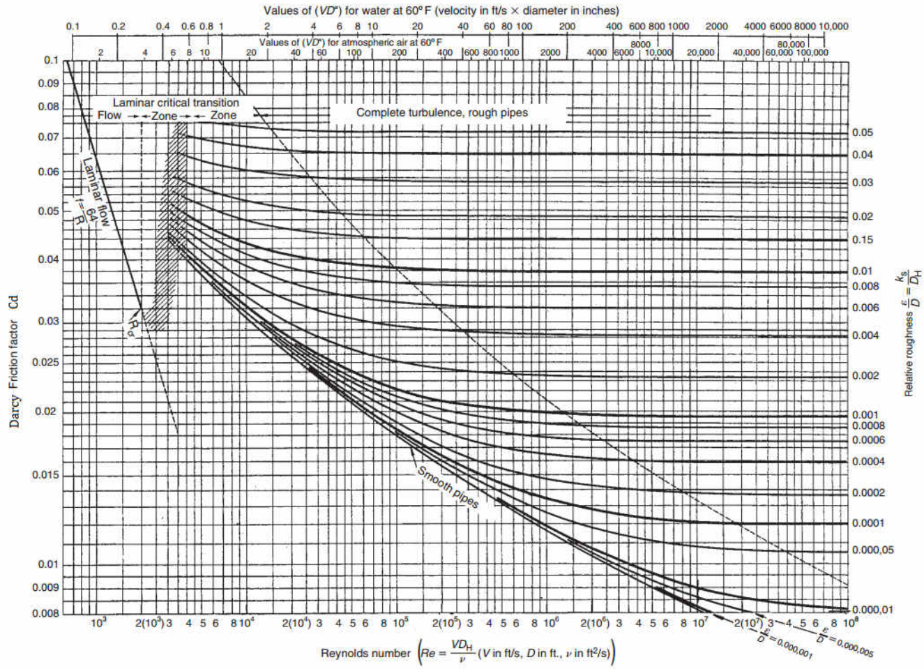
Figure 4.4: Moody diagram (after Moody, 1944, with permission of the American Society of Mechanical Engineers)
