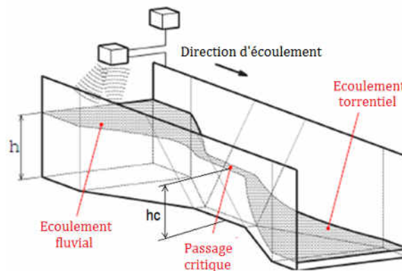
Figure 1.17: Canal Venturi
