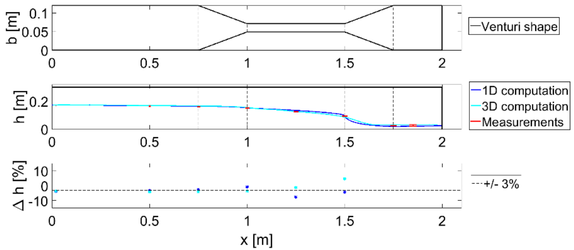
Figure 6.14: Exp. vs. 3D vs. 1D for a Carbopol flow with \tau_y = 1.6 Pa.s , k = 0.81 Pa.s^n , n = 0.53 , \rho = 1000 Kg/m^3 and Q = 161.3 L/min
