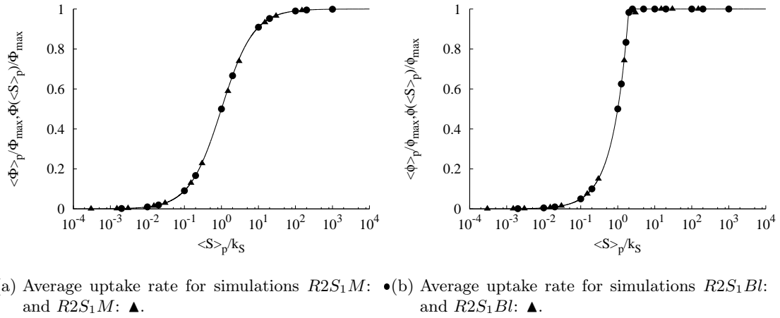
Figure 4.2: Non-dimensionalised average uptake rate \langle \Phi \rangle_p for Monod (left) and Blackman (right) assimilation models with respect to the dimensionless ratio \langle S \rangle_p / k_S for the dynamic flow R2 . Symbols refer to mean concentrations S_0 = 1 \text{ kg}_S \cdot \text{m}^{-3} : \bullet and S_0 = 0.15 \text{ kg}_S \cdot \text{m}^{-3} : \blacktriangle . (—) represents the non-dimensionalised uptake rate based on the average substrate concentration \Phi(\langle S \rangle_p) .
