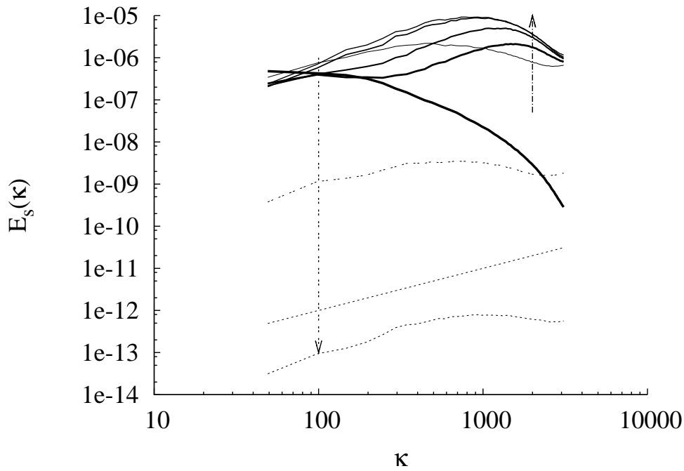
Figure 5.32: Substrate energy spectra for different times of the substrate decay. The bolder line correspond to the initial state. The thicker the line, the bigger the time. The arrow \dashleftarrow shows the initial evolution whereas the \dashrightarrow arrow presents the second phase evolution.
