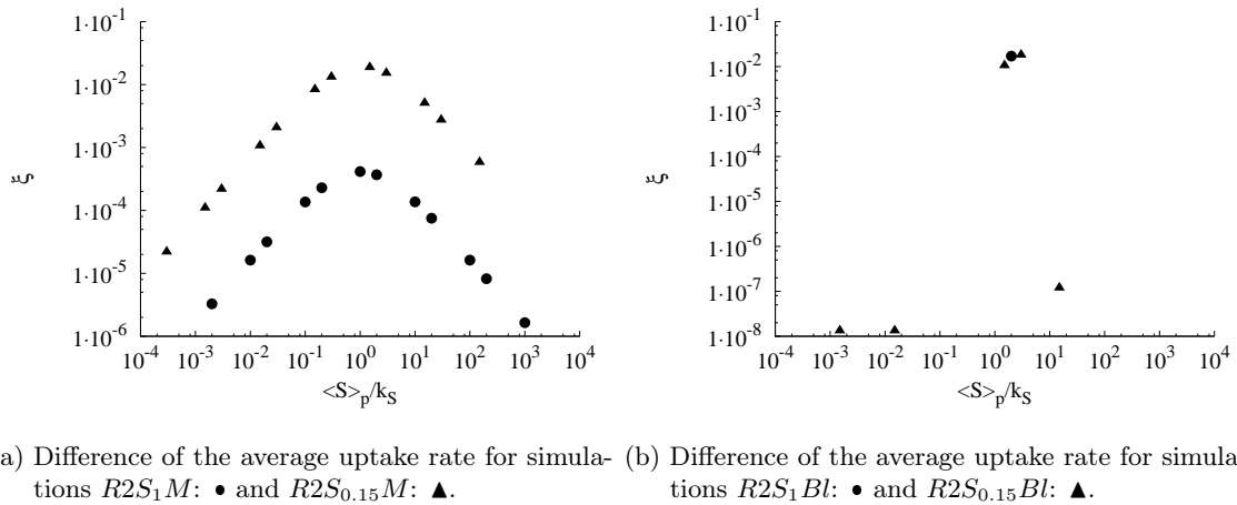
Figure 4.3: Deviation from the average uptake rate \langle \Phi \rangle_p to the uptake rate based on average substrate concentration for Monod (left) and Blackman (right) assimilation models with respect to the dimensionless ratio \langle S \rangle_p / k_S for the dynamic flow R2 . Symbols refer to mean concentrations S_0 = 1 \text{ kg}_S \cdot \text{m}^{-3} : \bullet and S_0 = 0.15 \text{ kg}_S \cdot \text{m}^{-3} : \blacktriangle .
