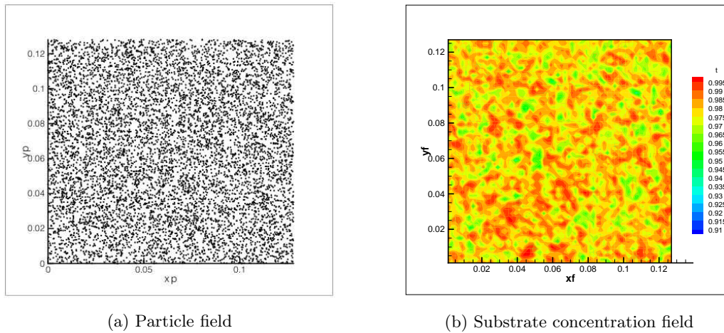
Figure 5.22: 2D view of particle (a) and substrate concentration field (b) for Blackman assimilation model with S_0 = 1 , k_S = 10^3 (in [\text{kg}_S \cdot \text{m}^{-3}] ) at t = 2.5 \cdot 10^{-2} s.
