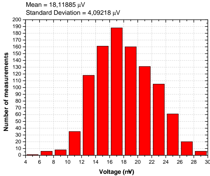
Figure 68: Histogram of the produced voltage for 1000 points of measurements at angle = 0^\circ , the applied power is 20 dBm and the frequency is 30.75 GHz.
