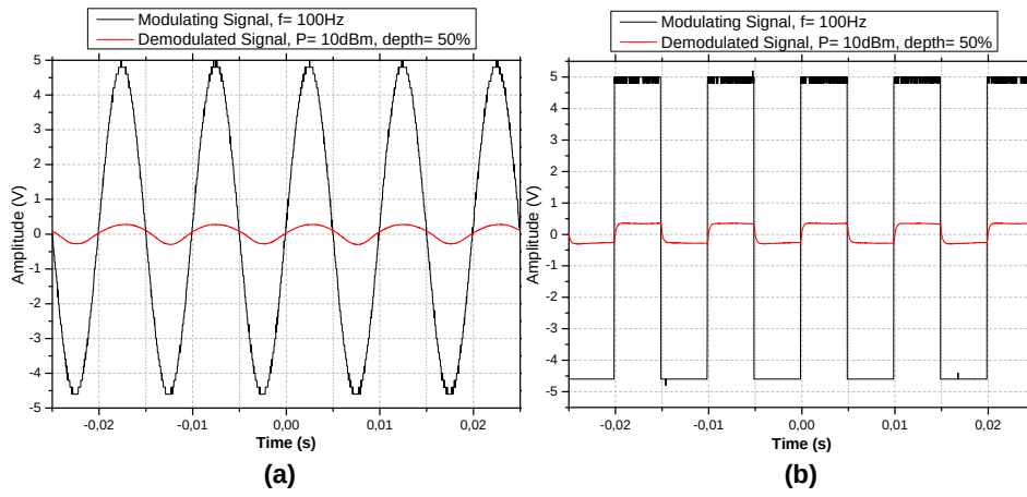
Figure 46: Virgin sample response to the applied amplitude modulated RF signal for an output power of 10 dBm and a modulation depth of 50 %. (a) Sine wave modulating signal, (b) pulse wave modulating signal, with f = 100 Hz and a carrier signal of f = 36.71 GHz.
