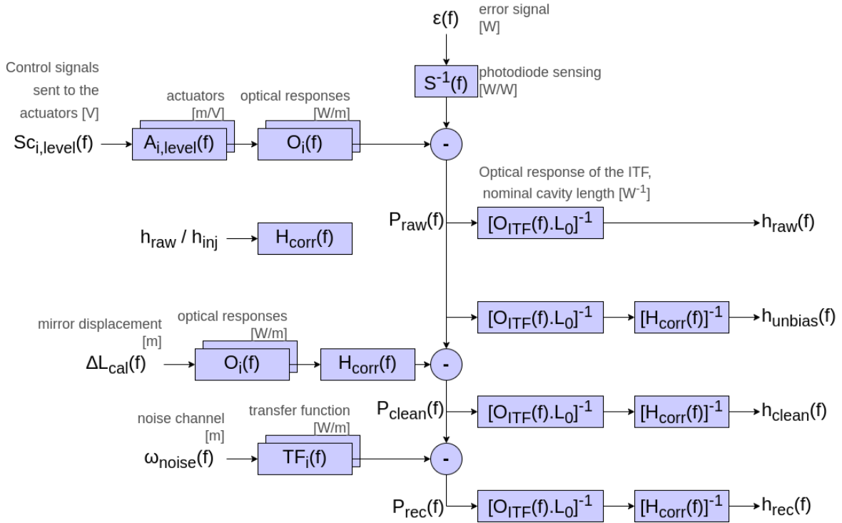
Figure 4.2: Simplified block diagram of the total reconstruction pipeline.
