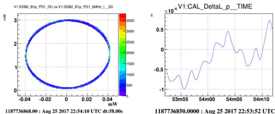
Figure 3.11: Left: P_{AC} as function of P_{DC} while a signal is injected on the mirror command. Right: Reconstructed \Delta L signal
