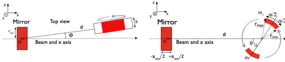
Figure 3.8: Scheme of the NCal principle. The NCal makes the mirror move along the x axis which is the laser axis. The z axis is the vertical axis.
