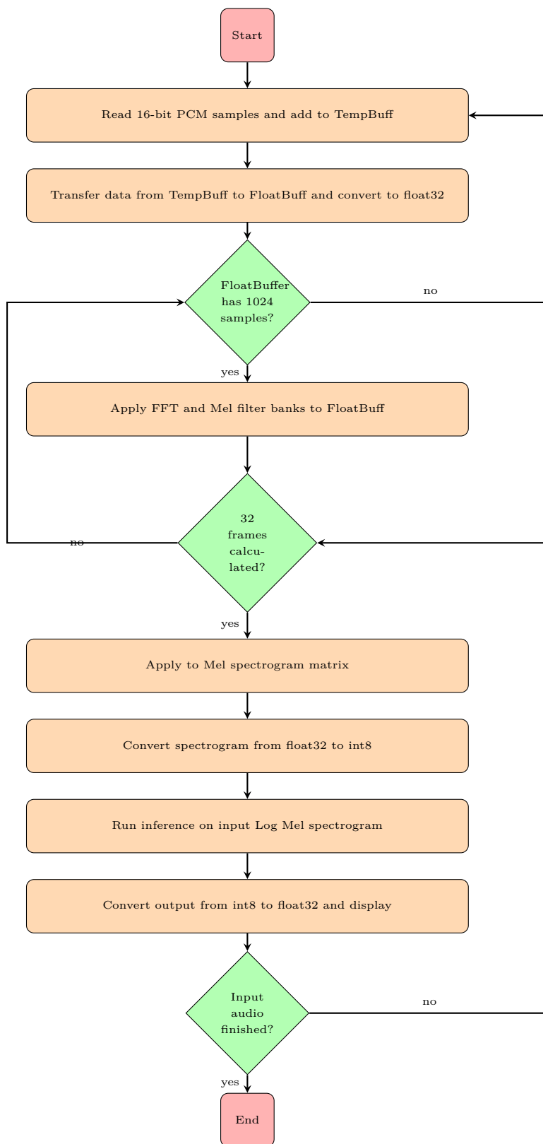
Figure 4.5 – Processing chain for inference on STM32 SensorTile.
