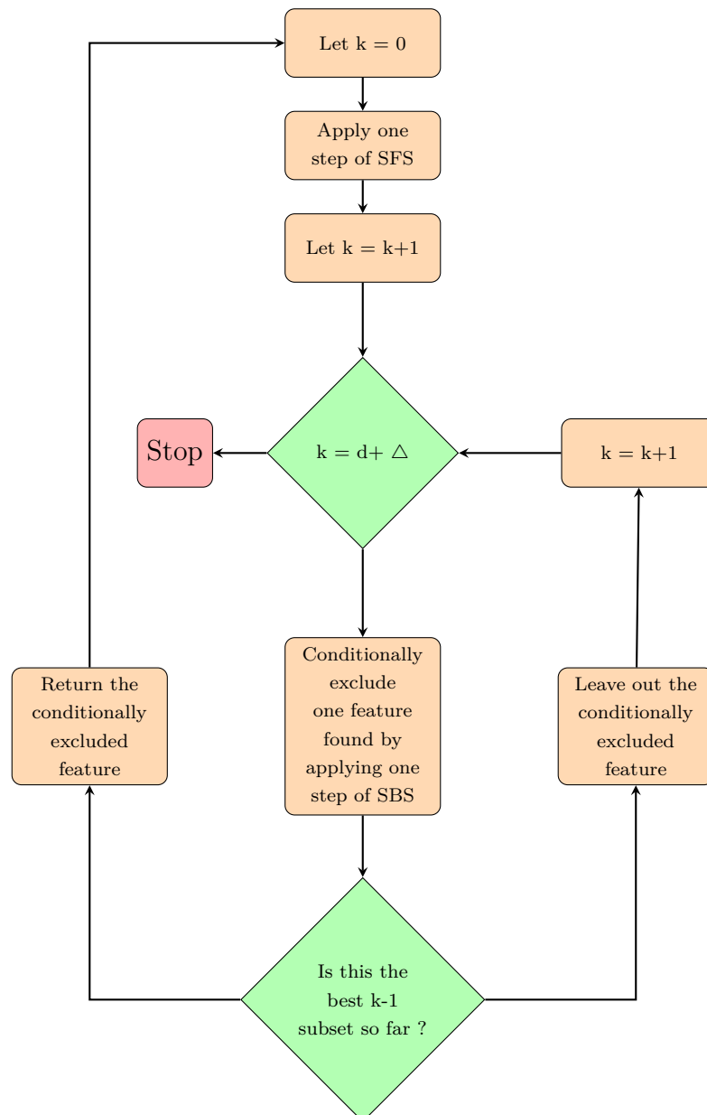
Figure 3.1 – Sequential Forward Floating Selection (SFFS) Algorithm.
