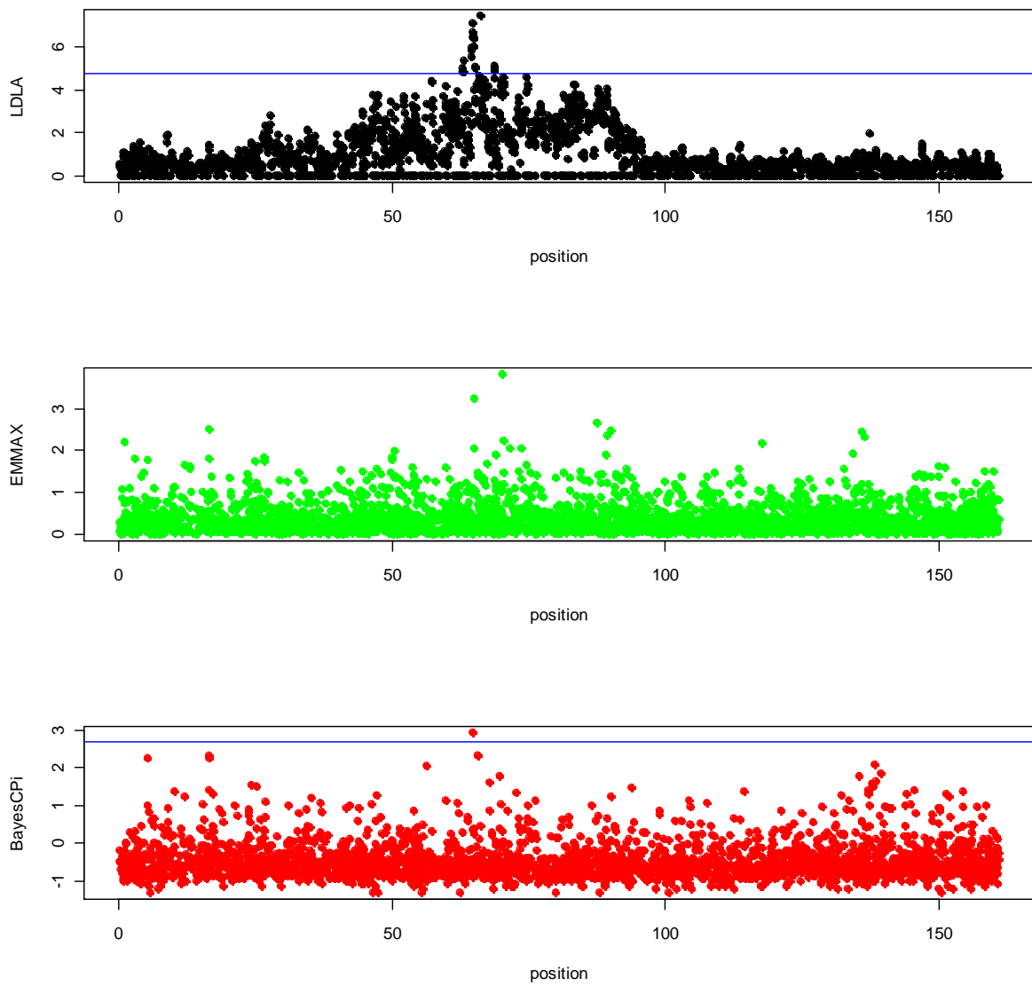
244 Figure 1. Scan of chromosome 1 in dairy cattle. Y-axis: \log_{10}(1/p\text{-value}) for LDLA and 245 EMMAX; \log_{10}(\text{Bayes Factor}) for BayesCPI. X-axis: position along the chromosome (in 246 cM). The blue line (if any) is the rejection threshold.
