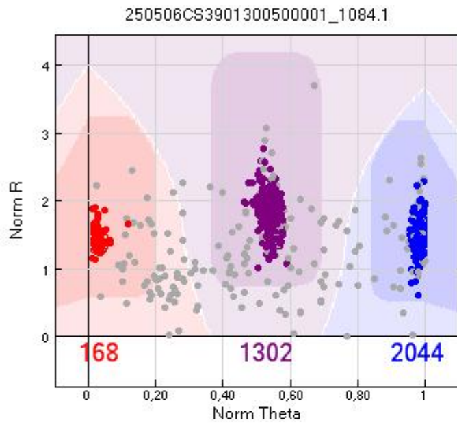
Figure 5.8: Fluorescence cluster
