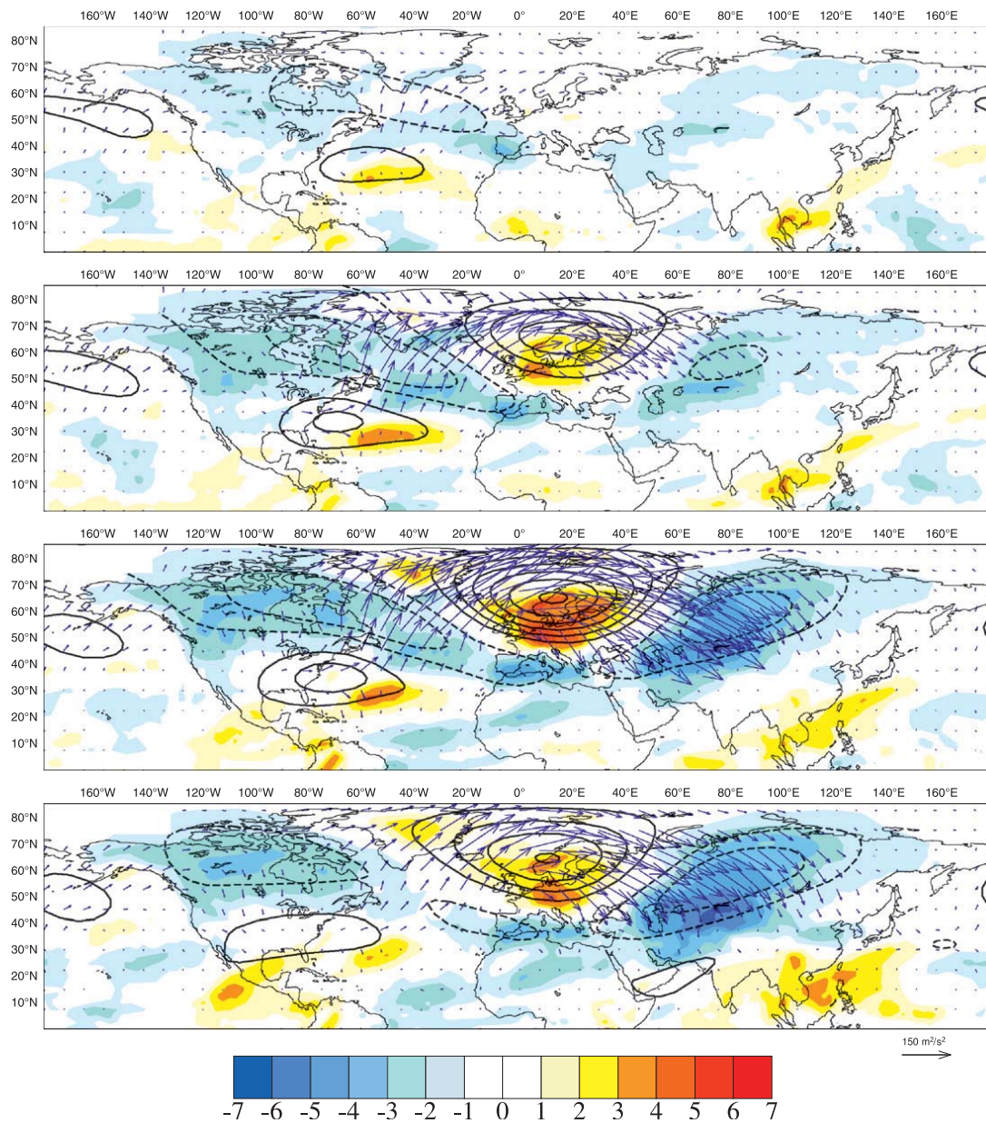
FIG. 15. Regression of the low-frequency streamfunction (black contours; solid and dashed lines correspond respectively to positive and negative values; first contour and interval are 2 \times 10^6 \text{ m}^2 \text{ s}^{-1} ), of \mathbf{W}_H multiplied by 10 (only one arrow over three is plotted) at 200 hPa and of the low-frequency OLR (shaded; first contour and interval are 1 \text{ W m}^{-2} ) on the blocking index for the period 1974–2001 for lag (a) –8, (b) –4, (c) 0, and (d) +4 days.
