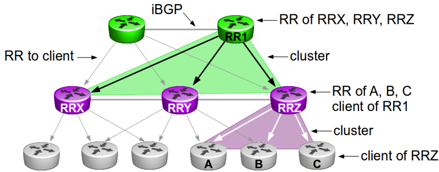
Figure 2.14 – Examples of route reflection
