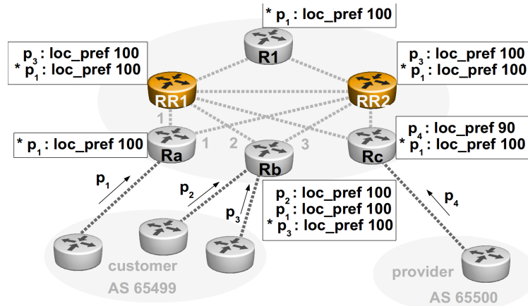
Figure 3.10 – Diversity loss within an ISP's network
