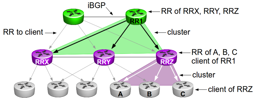
Figure 2.14 – Examples of route reflection
