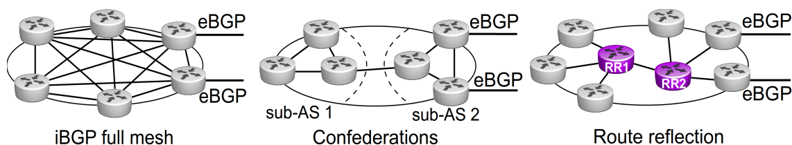
Figure 9.1 – Examples of a full mesh of iBGP sessions, confederations, route reflection
