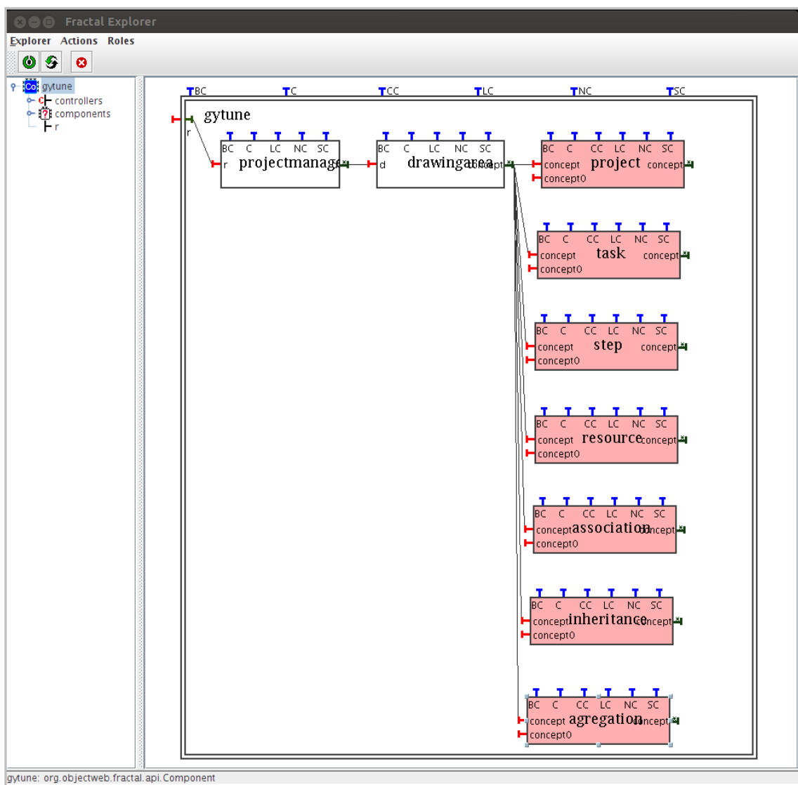
FIGURE 9.7 – Syntaxe abstraite
