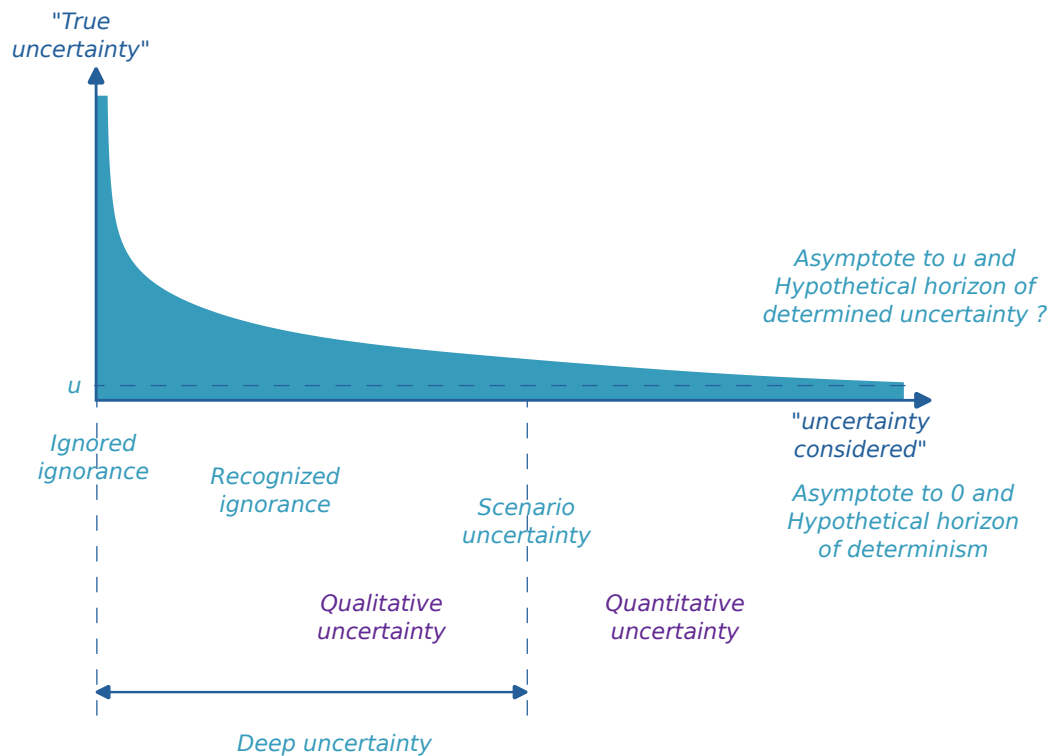
Figure 1.1: Conceptual view of the different types of uncertainties. It starts from ignored uncertainty which represents the maximum of uncertainty and converge asymptotically to the hypothetical horizon of determined uncertainty. The region of deep and qualitative uncertainty is displayed.
