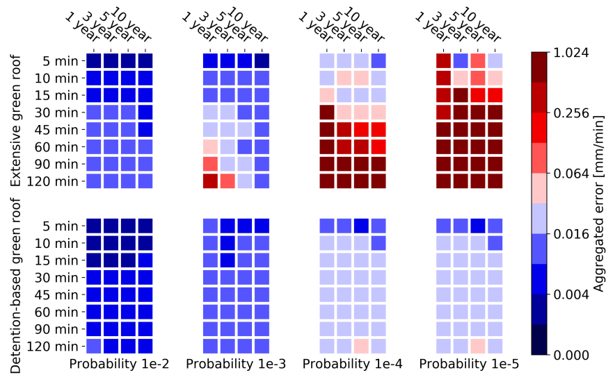
Figure 3.2: Aggregated error of the survival discharge for different log-probability level depending on resolution (y-axis) and amount of input data (x-axis).
