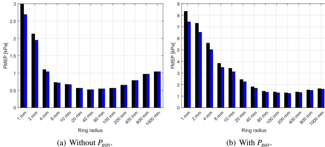
Figure 5.16: Predicted FMEP aver a full engine cycle as a function of the ring radius.
