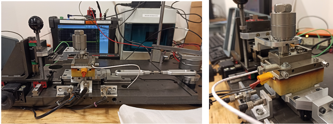
Figure 3.3: ARTEMIS test-rig.
