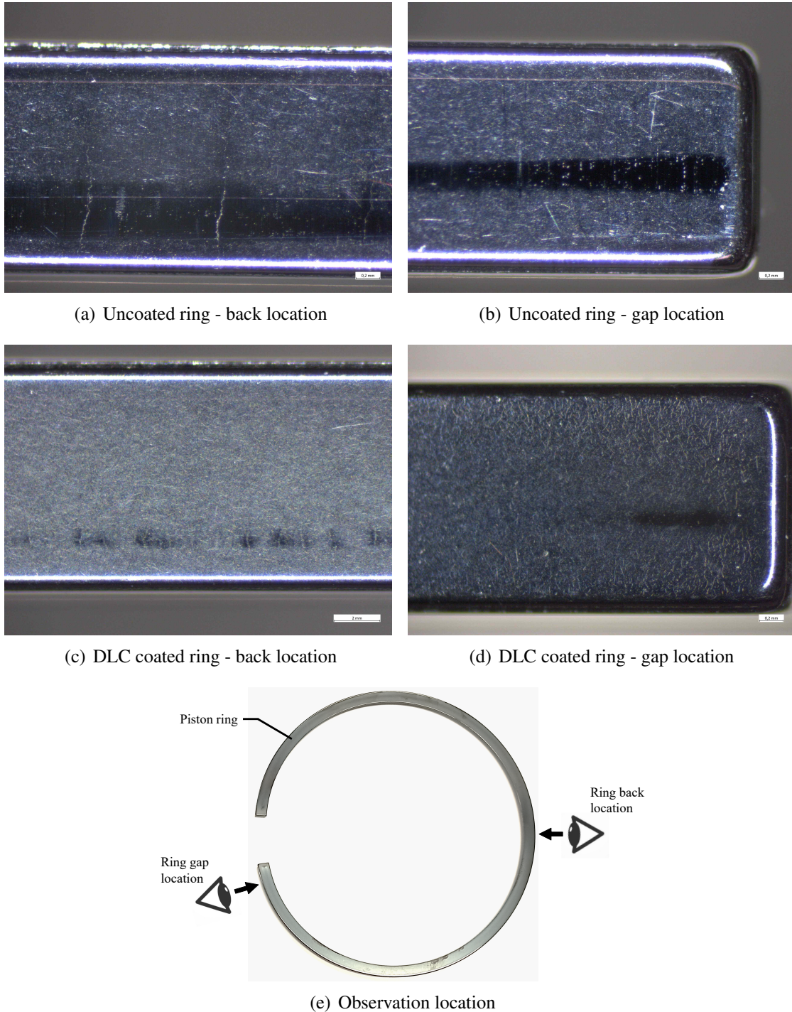
Figure 5.8: Microscope pictures of both tested compression rings, the dark zones highlight the wear scars.
