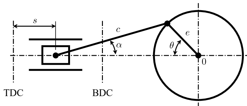
Figure 2.5: Piston / con-rod / crankshaft mechanism.
