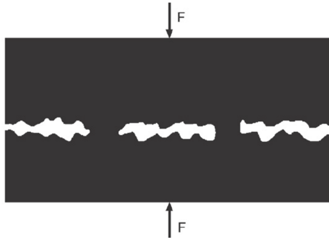
Figure 2.2: Schematic of the contact mechanics problem: how large is the real area of contact when two solids with rough surfaces are pushed into contact ? [8]
