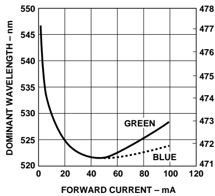
Figure 7. Color vs. forward current.
