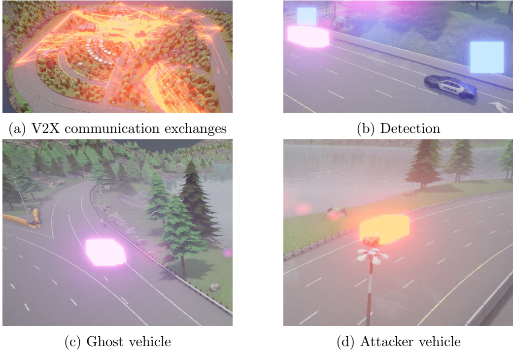
Figure 6.2: Plotting module visualization examples.
