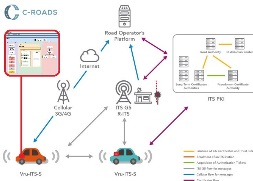
Figure 4.2: CAV-MBDA as part of C-Roads project architecture [7]
