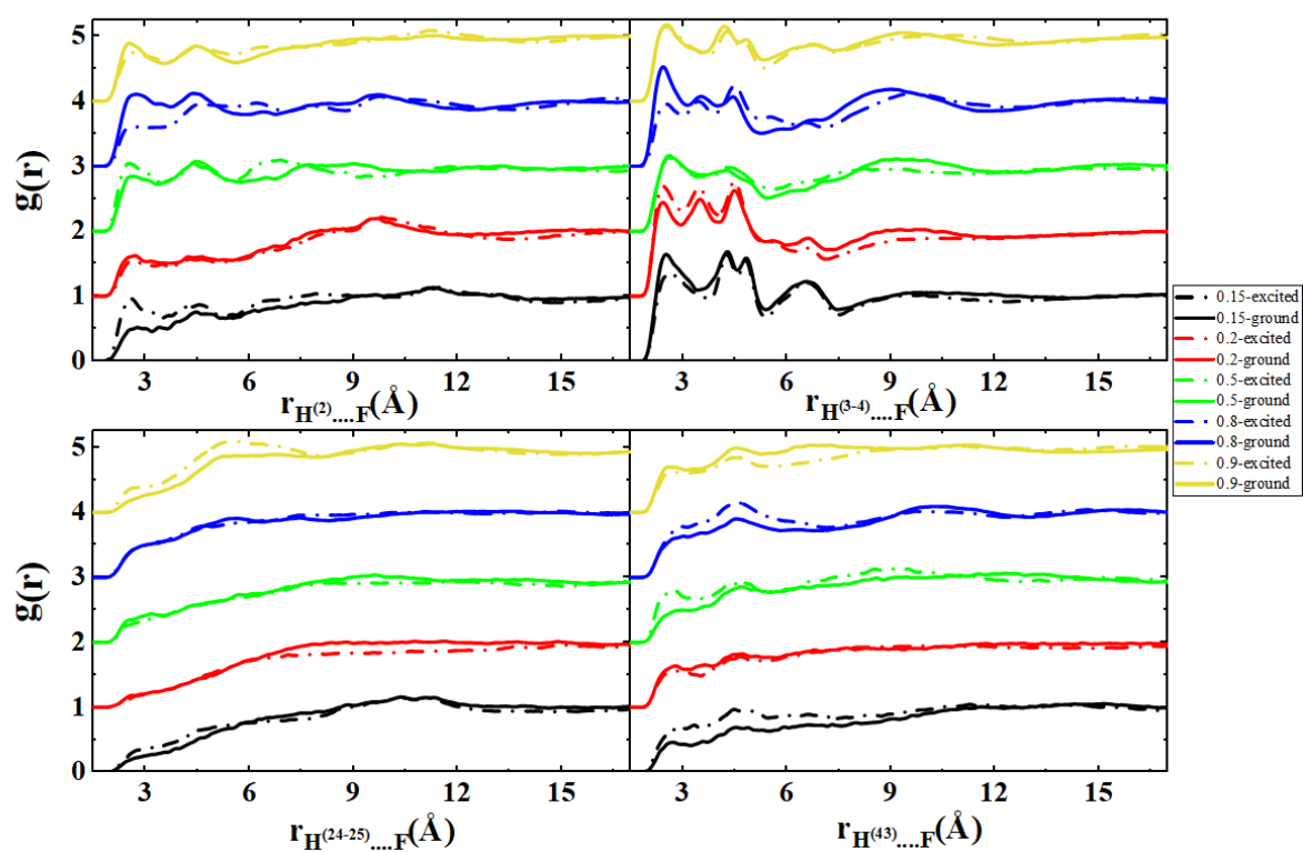
Figure 2.22. The ionic liquid mole fraction dependence of the radial distribution function of the F atom of the anion \text{BF}_4^- around hydrogen atoms chosen in the donor \text{H}^{(43)} , bridge \text{H}^{(2)} , the acceptor \text{H}^{(3-4)} and butyl chain \text{H}^{(24-25)} parts of the dye D205 dye. These functions were calculated in the ground and excited states.
