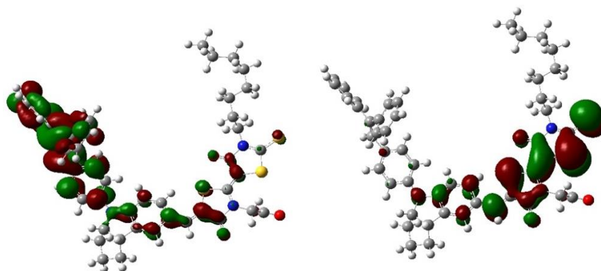
Figure 2.4. HOMO (left) and LUMO (right) spectrum of D205 dye
