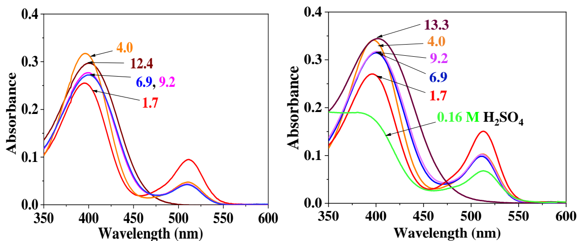
Figure 3.11: Steady-state absorption spectra of 2,4,5,7,4'- and 2,4,5,7,5'-pentanitrofluorescein in water with 1 vol % DMSO; the numbers denote the pH values; dye concentrations: 1.01 \times 10^{-5} and 1.57 \times 10^{-5} M, respectively.
