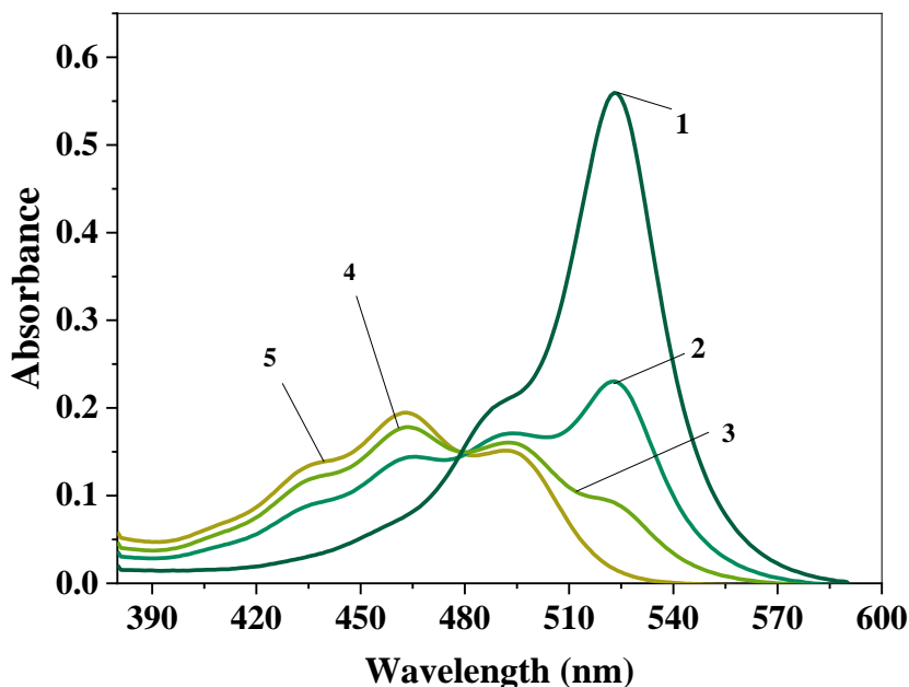
Figure 4.6: Steady-state absorption of 4'-Nitrofluorescein methyl ester in benzoate and salicylate buffer solutions in DMSO with 20 vol % water: 0.005M KBenz (1), 0.005M HBenz +0.005M KBenz (2), 0.0075 M HBenz +0.005M KBenz (3), 0.020 M HBenz +0.005M KBenz (4), 0.001 M H2Sal +0.005M NaHSal (5).
