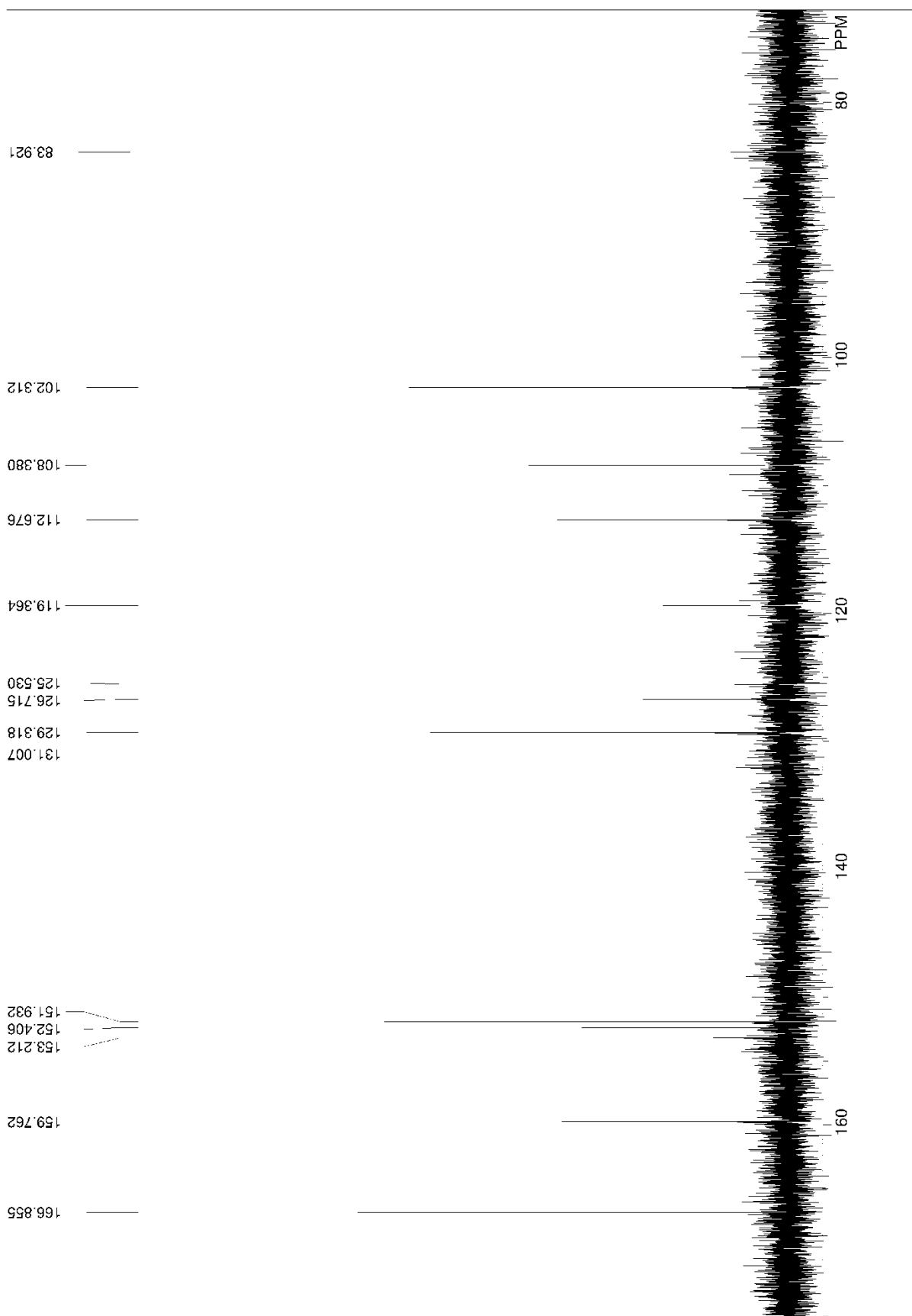
Figure A4: ^{13}\text{C} NMR spectrum of 5'-nitrofluorescein (101 MHz, DMSO- d_6 ).
