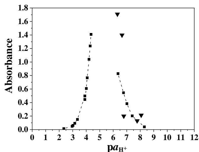
Figure 3.15: Absorption of 2,4,5,7-tetranitrofluorescein ( 4.2 \times 10^{-5} M) at 522 nm vs. p_aH^* . Picric acid solutions (left-hand side) and salicylate buffers (right-hand side); 2,6-dinitrophenolate buffer solutions are shown with a triangle.
