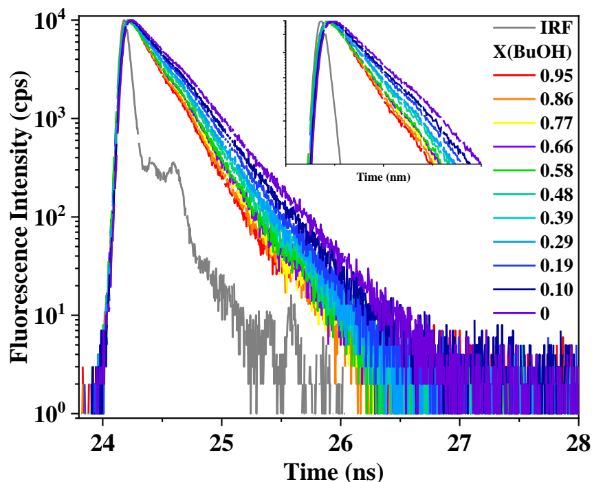
Figure 6.8: The fluorescence intensity decays of BDP2 in acetonitrile butanol mixtures, ( \lambda_{em}=513 nm). The instrument response function (IRF in grey) was recorded at 470 nm (FWHM = 80ps). The fluorescence intensity decays at the maximum are presented closer (inset).
