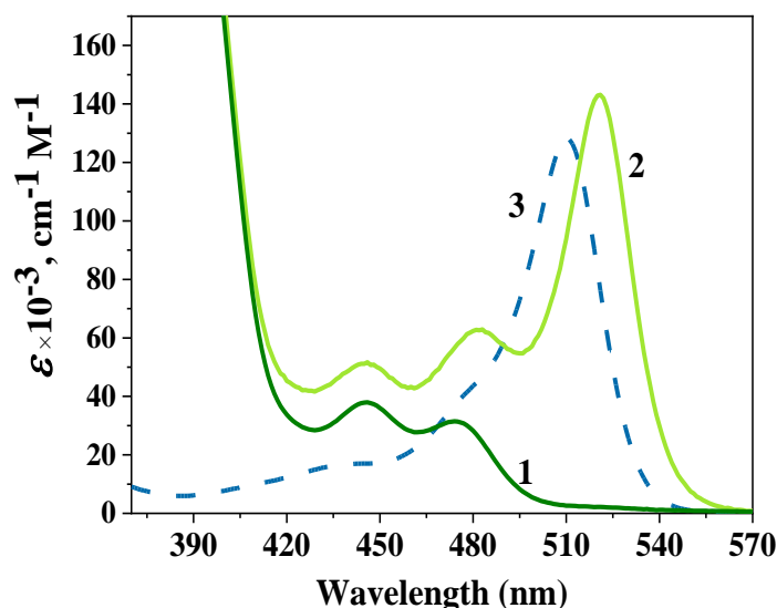
Figure 3.5: The molar extinction coefficient of 4,5-dinitrofluorescein: 1 – neutral form \text{H}_2\text{R} in the presence of 0.05 M p -toluenesulfonic acid; 2 – the spectrum in the presence of 0.001 M of p -toluenesulfonic acid; 3 – absorption of the \text{R}^{2-} dianion in the presence of 0.02 M DBU (in this case, the E values were divided by 650). The spectra 1 and 2 were obtained at dye concentrations of 3.7 \times 10^{-3} and 7.5 \times 10^{-4} M.
