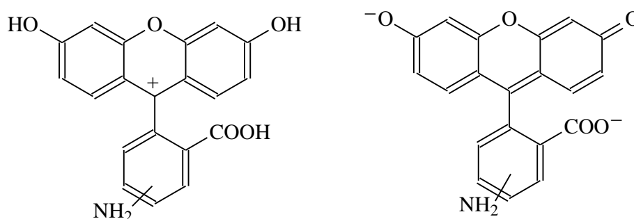
Figure 1.9: The structure of 4'- and 5'-aminofluoresceins in their cation and dianion forms.
