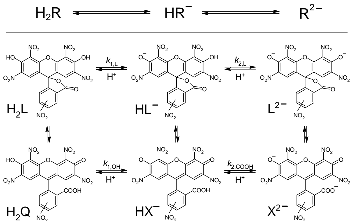
Figure 3.28: Detailed scheme of protolytic equilibrium of the nitro derivatives of fluorescein.
