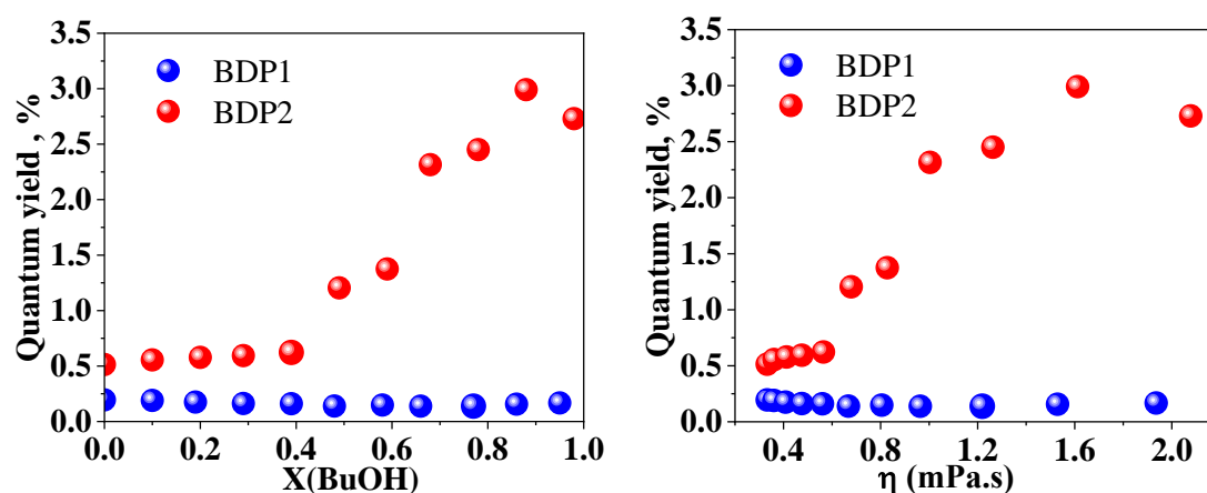
Figure 6.6: Fluorescence quantum yields of BDP1 (blue circle) and BDP2 (red circle) excited at 470 nm for various molar fractions of BuOH and viscosity. The reference used to measure the fluorescence quantum yields was rhodamine 6G in ethanol (excited at the same wavelength).
