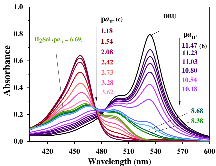
Figure C3: Steady-state absorption spectra of ethyl ester of 4'-nitrofluorescein in DMSO at different pK_{a_{H^+}} values in salicylate (a) and benzoate (b) buffer solutions and in p -toluenesulfonic acid solutions (c).
