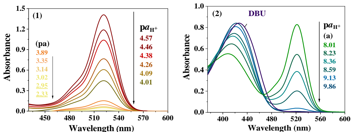
Figure 3.14: Steady-state absorption spectra of 2,4,5,7-tetranitrofluorescein ( 4.2 \times 10^{-5} M) in diluted picric acid (pa) (1) and in the salicylate buffer solutions (a) (2). The R^{2-} spectrum was obtained in 0.02 M DBU solution.
