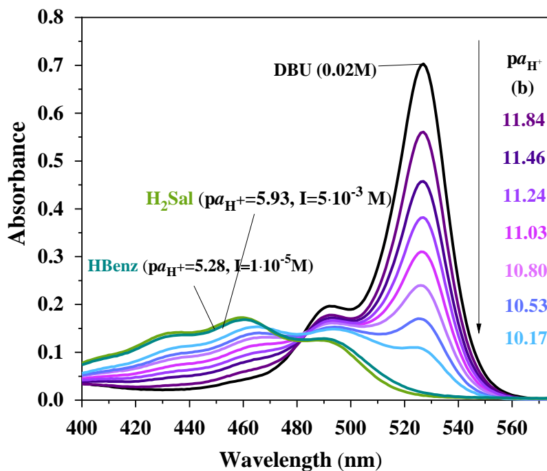
Figure 4.1: Steady-state absorption spectra of ethyl ester of 4'-aminofluorescein in DMSO at different pH values where H_2Sal – salicylic acid, HBenz – benzoic acid, salicylate (a) and benzoate (b) buffer solutions and in p -toluenesulfonic acid solutions (c).
