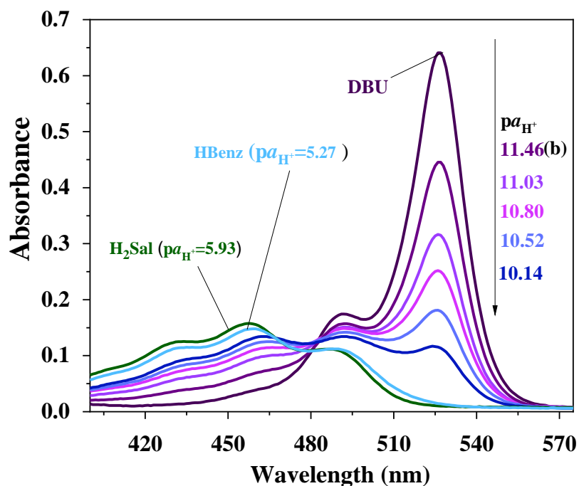
Figure C4: Steady-state absorption spectra of ethyl ester of 5'-aminofluorescein in DMSO at different pK_{a_{H^+}} values in salicylate (a) and benzoate (b) buffer solutions and in p -toluenesulfonic acid solutions (c).
