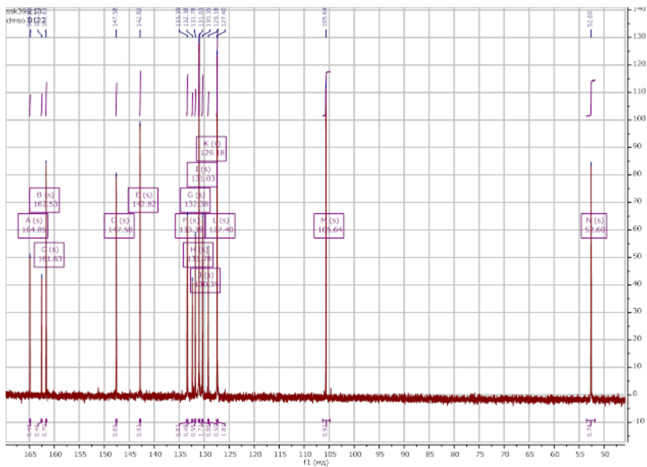
Figure A22: ^{13}\text{C} NMR spectrum of 2,4,5,7-tetranitrofluorescein methyl ester (methyl 2-(3,6-dihydroxy-2,4,5,7-tetranitro-9H-xanthen-9-yl)benzoate): (101 MHz, \text{DMSO-}d_6 ) \delta 164.85, 162.53, 161.63, 147.58, 142.82, 133.39, 132.38, 131.78, 131.03, 130.35, 129.18, 127.40, 105.64, 52.60 ppm.
