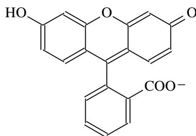
Figure 1.4: Fluorescein monoanion, HQ - .
