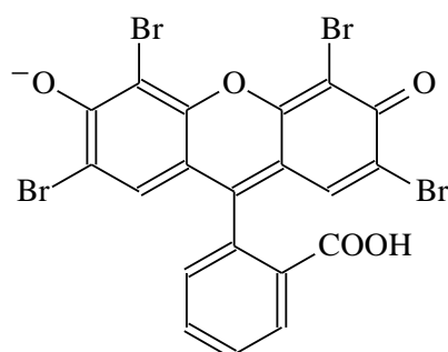
Figure 1.6: The molecular structure of the eosin monoanion, HX^- .
