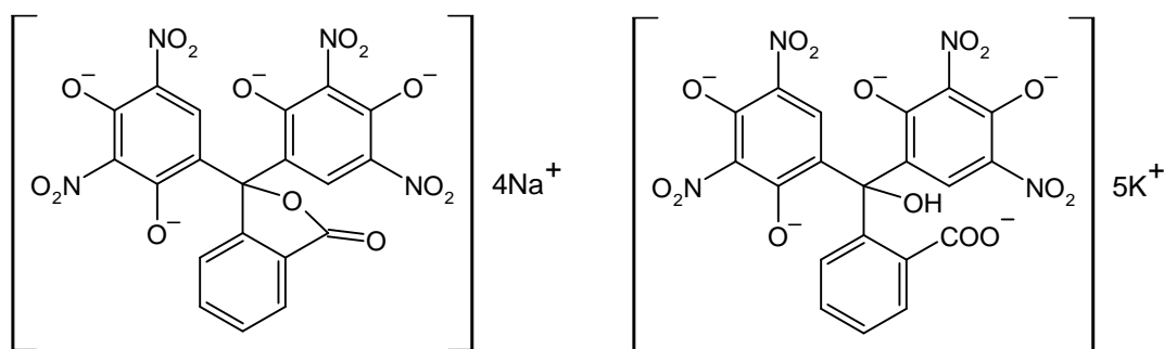
Figure 3.9: Highly charged anions of 2,4,5,7-tetranitrofluorescein with ruptured pyran ring identified using electrospray spectroscopy (left) and X-ray analysis of crystals (right) [6].
