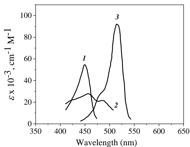
Figure 1.5: Spectra of fluorescein ionic forms in 91 mass % aqueous dimethyl sulfoxide (DMSO): H 3 R + (1); HR - (2); R 2- (3) [20].
