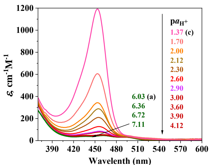
Figure 3.24: Absorption spectra of 5'-nitrofluorescein in DMSO in the acidic region ( p -toluenesulfonic acid solutions (c) and in salicylate (a) buffer solutions).
