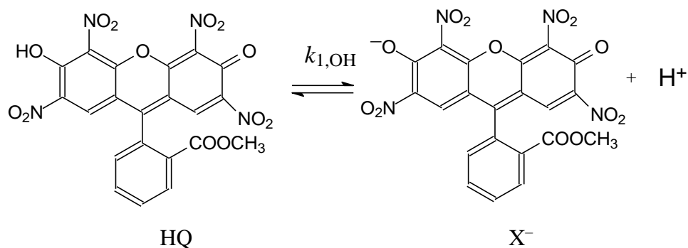
Figure 3.12: Dissociation equilibrium of 2,4,5,7-tetranitrofluorescein methyl ester
