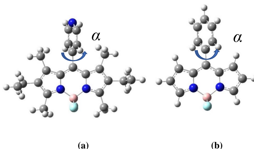
Figure 6.11: Structure of Molecular structures of BODIPYs under study: BDP1 (left) and BDP2 (right). \alpha is the dihedral angle that defines the rotation of the phenyl group with respect to the pyridine BODIPY core.
