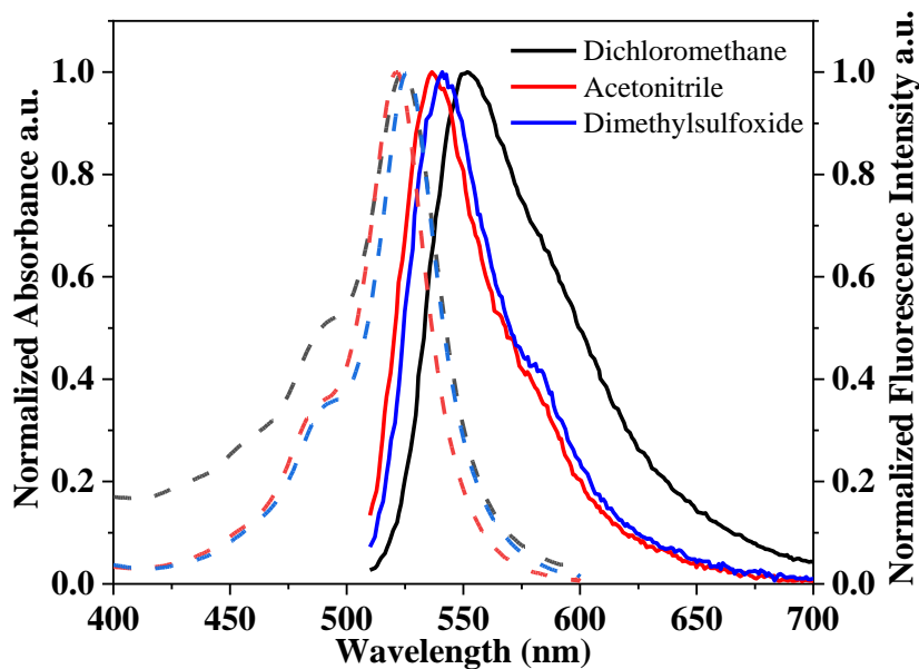
Figure 5.2: Normalized absorption (dash line) and fluorescence spectra of 4'-nitrofluorescein in dichloromethane (1; -----), acetonitrile (2; - - - - -), and dimethylsulfoxide (3; - - - - -); 0.02 M DBU in all solutions ensure complete conversion of the dye into the R^{2-} ion.
