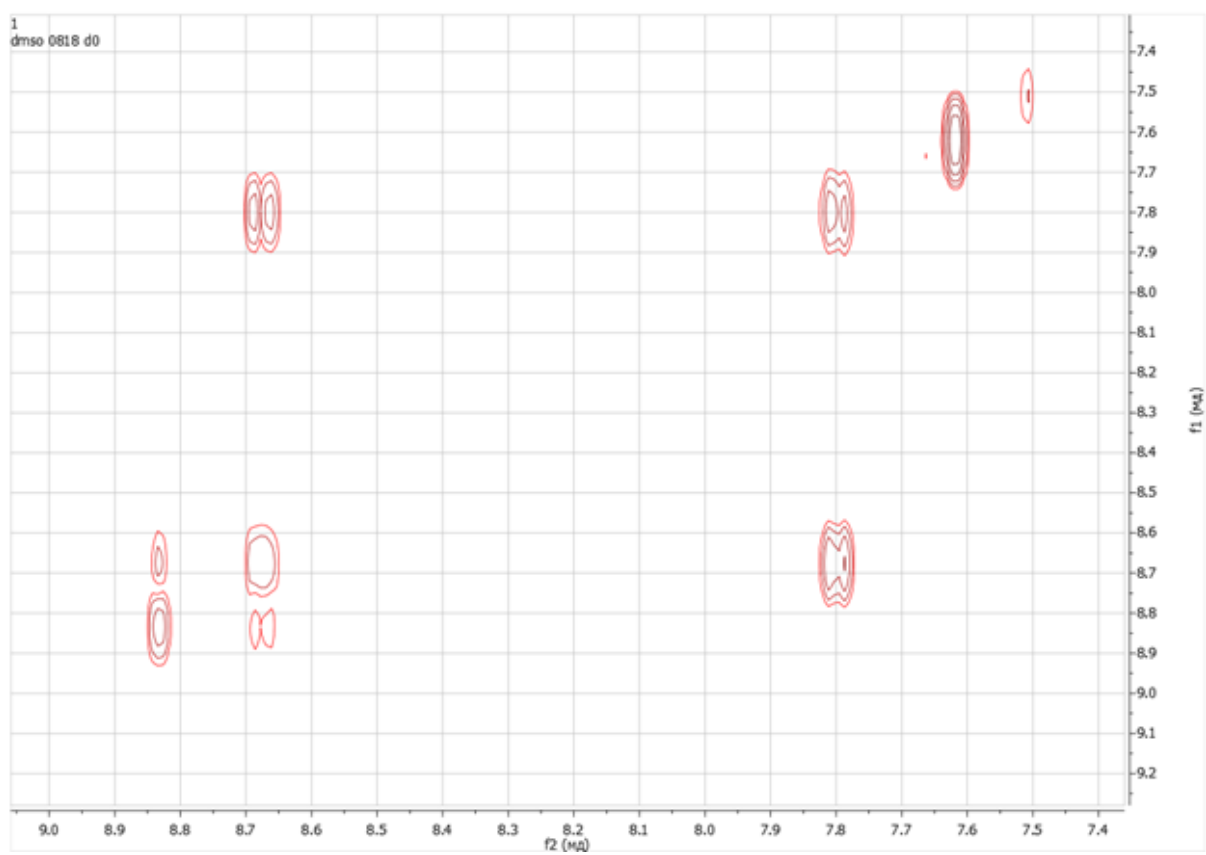
Figure A14: ^1\text{H} - ^1\text{H} COSY NMR spectrum of 2,4,5,7,4'-pentanitrofluorescein (400 MHz, DMSO- d_6 ).
