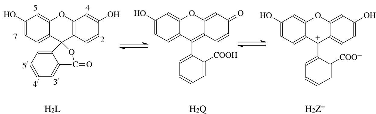
Figure 1.3: Molecular structures of the neutral form of fluorescein.
