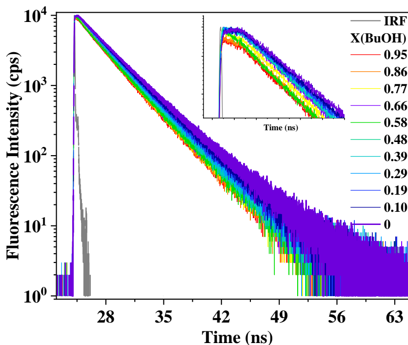
Figure 6.7: The fluorescence intensity decays of BDP1 in acetonitrile/butanol mixtures, pure ACN ( \lambda_{em}=538 nm), X (BuOH) = 0.1 and 0.19 ( \lambda_{em}=539 nm), X (BuOH) = 0.29 and 0.39 ( \lambda_{em}=540 nm), X (BuOH) = from 0.48 to 0.95 ( \lambda_{em}=541 nm). The instrument response function (IRF in grey) was recorded at 470 nm (FWHM = 80ps). The fluorescence intensity decays at the maximum are presented closer (inset).
