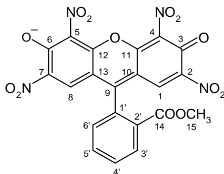
Figure 2.6: Anion of the methyl ester of 2,4,5,7-tetranitrofluorescein.
