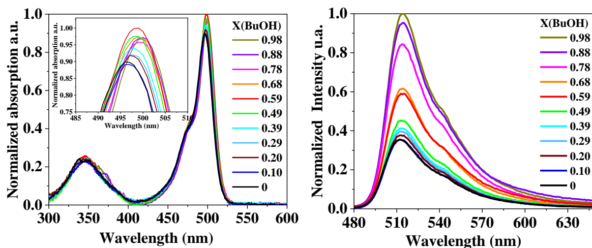
Figure 6.4: Normalized steady-state absorption (left) and emission (right) spectra of BDP2 in whole mixture composition of AN and BuOH ( \lambda_{\text{excitation}}=470 nm). The absorption spectra at the maximum are shown in the inset.
