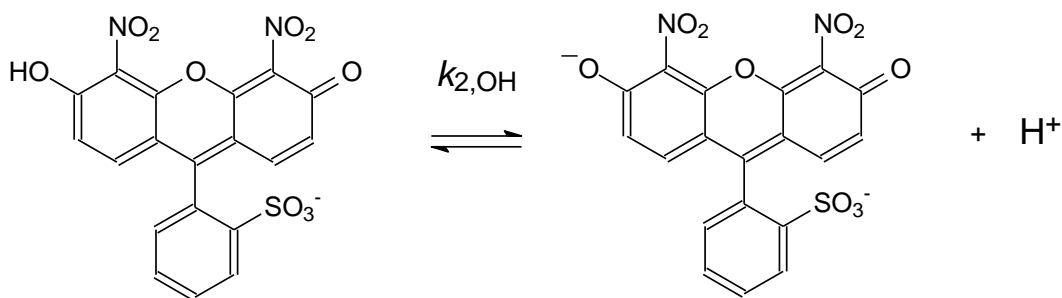
Figure 3.26: The dissociation of methyl ester of 4,5-dinitrofluorescein (top panel) and 4,5-dinitrosulfofluorescein (bottom panel).
