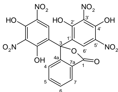
Figure 2.4: 2,4,5,7-Tetranitrofluorescein with the cleaved pyran ring in lactonic form.
