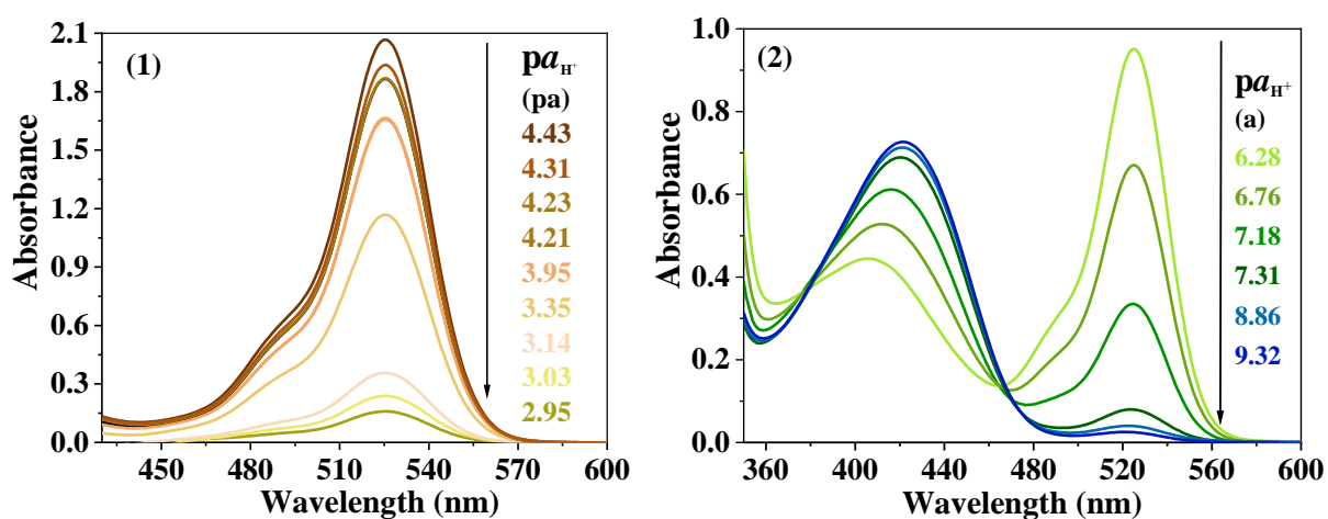
Figure 3.17: Steady-state absorption spectra of 2,4,5,7,5'-pentanitrofluorescein ( 4.4 \times 10^{-5} M) in diluted solutions of the picric acid (pa) (1) and in the salicylate buffer solutions (a) (2). The R^{2-} spectrum was obtained in 0.02 M DBU solution.
