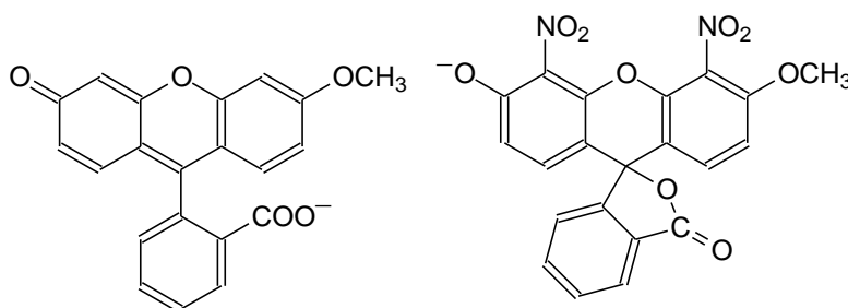
Figure 3.27: The structures of the single-charged anions of methyl ethers of fluorescein (left) and 4,5-dinitrofluorescein (right).
