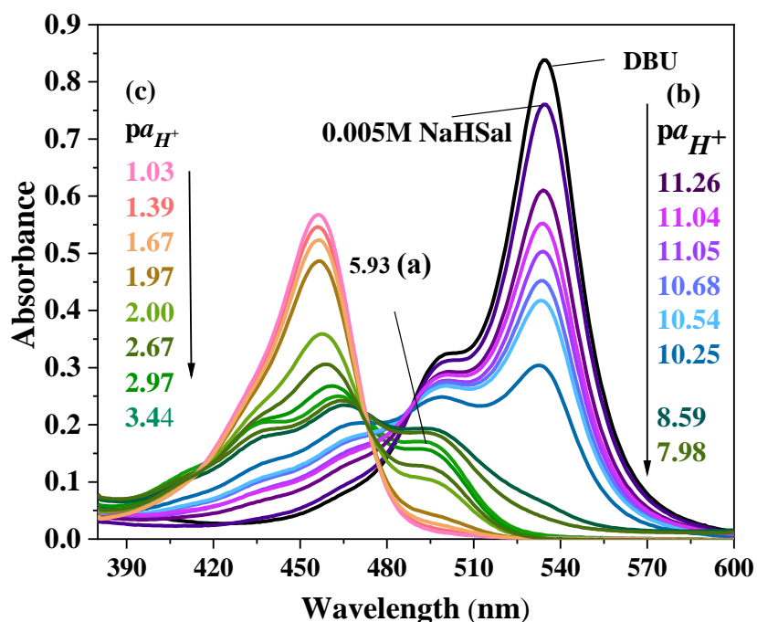
Figure 4.2: Steady-state absorption spectra of ethyl ester of 5'-nitrofluorescein in DMSO at different pH values where salicylate (a) and benzoate (b) buffer solutions and in p -toluenesulfonic acid solutions (c).
