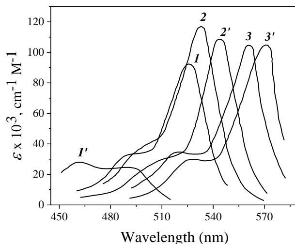
Figure 1.7: Absorption spectra of R^{2-} (1–3) and HR^{-} (1'–3') of 3',4',5',6'-tetrachlorofluorescein (1, 1'), 2,4,5,7-tetraiodofluorescein (erythrosin) (2, 2'), and 2,4,5,7-tetraiodo-3',4',5',6'-tetrachlorofluorescein (rose Bengal B) (3, 3') in 90 mass % aqueous acetone [34].
