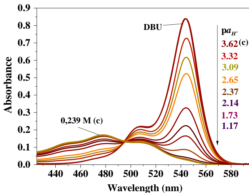
Figure 4.4: Steady-state absorption spectra of methyl ester of eosin in DMSO at different concentrations of p -toluenesulfonic acid (c); pa_{H^+}^* = -\log c_{H^+} - \log f_1 . The values below pa_{H^+}^* should be considered conventional ones because of relatively high ionic strength. The spectra in 0.239 M acid and 0.02 M DBU correspond to the neutral form, HR, and the anion, R^- , respectively.
