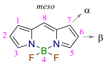
Figure 6.1: Structure of 4,4-difluoro-4-bora-3a,4a-diaza-s-indacene, BODIPY “core”.
