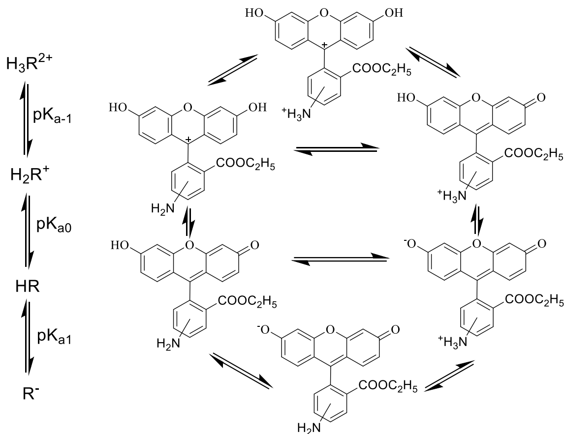
Scheme 4.2: Scheme of equilibria of amino-substituted fluorescein esters.
