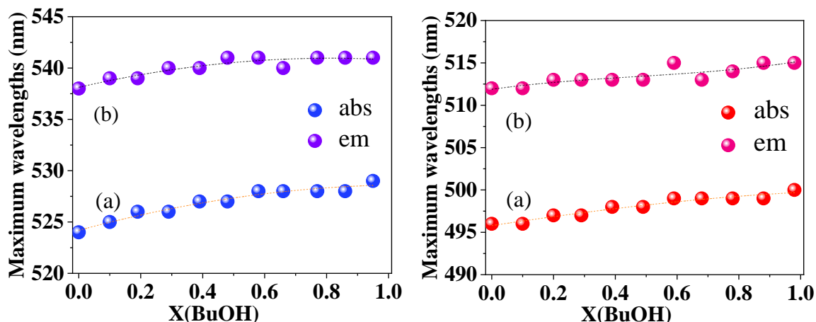
Figure 6.5: Maximum absorption (a) and emission (b) wavelengths for S_0 \rightarrow S_1 transition for BDP1(left) and BDP2 (right) as a function of the molar fraction of the BuOH.
