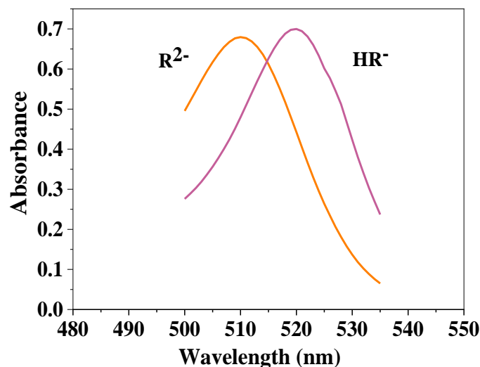
Figure 3.4: Steady-state absorption spectra of the anions of 4,5-dinitrofluorescein in DMSO at ionic strength of 0.005 M; the \text{HR}^- spectrum was singled out using the calculated \text{p}K_a values.
