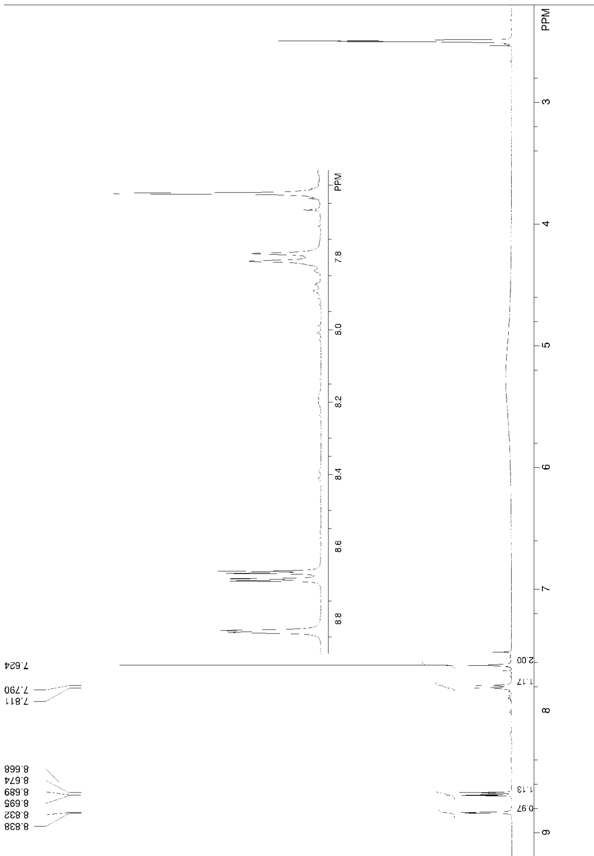
Figure A13: ^1\text{H} NMR spectrum of 2,4,5,7,4'-pentanitrofluorescein (400 MHz, \text{DMSO-}d_6 ).
