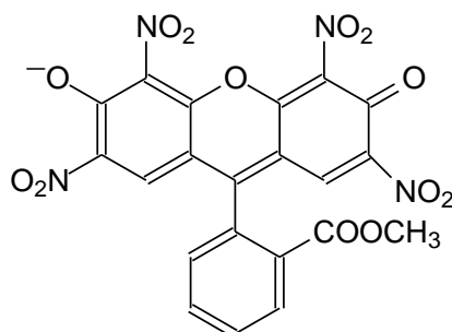
Figure 5.7: The methyl ester of the 2,4,5,7-tetranitrofluorescein anion R^- .
