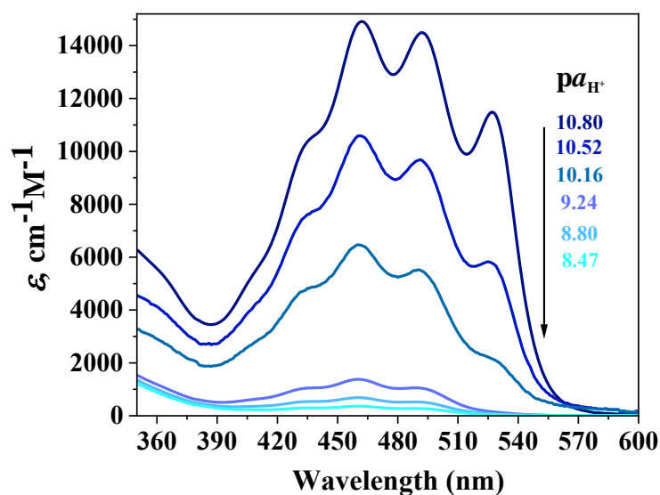
Figure 3.21: Absorption of 5'-nitrofluorescein in the acidic range of the benzoate buffer solutions in DMSO.
