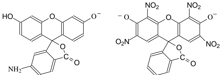
Figure 1.10: Examples of anions with lactonic structure: HL^- of 5'-aminofluorescein and L^{2-} of 2,4,5,7-tetranitrofluorescein.
