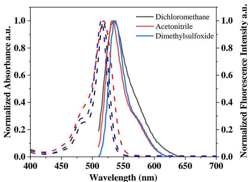
Figure 5.3: Normalized absorption (dash line) and fluorescence spectra of 4'-aminofluorescein in dichloromethane (1; -----), acetonitrile (2; - - - - -), and dimethylsulfoxide (3; - - - - -); 0.02 M DBU in all solutions ensure complete conversion of the dye into the R^{2-} ion.
