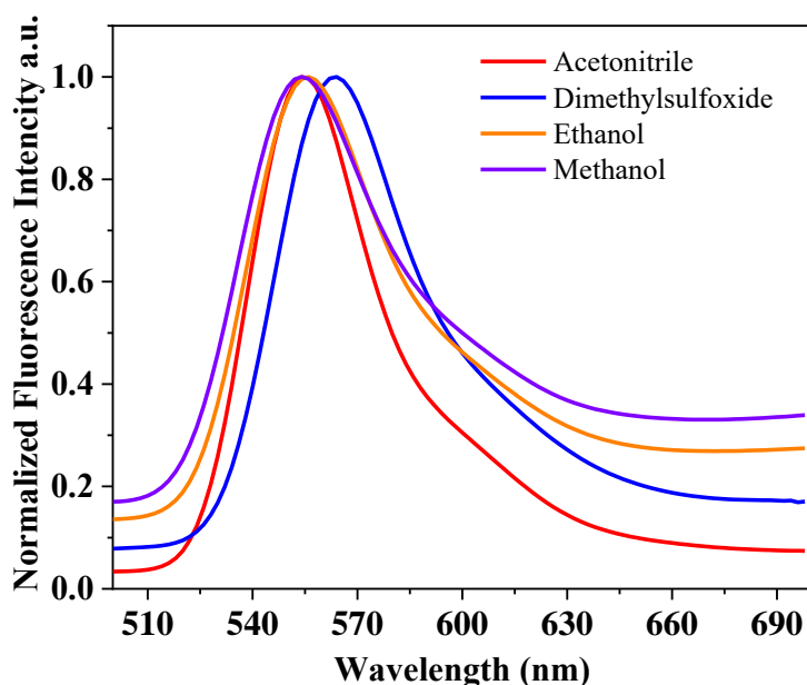
Figure 5.8: Normalized fluorescence spectra of the methyl ester of the 2,4,5,7-tetranitrofluorescein in methanol (-----), ethanol (-----) acetonitrile (2; -----), and dimethylsulfoxide (3; -----); 0,01 M NaOH and 0.02 M DBU in solutions ensure complete conversion of the dye into the R^- ion.
