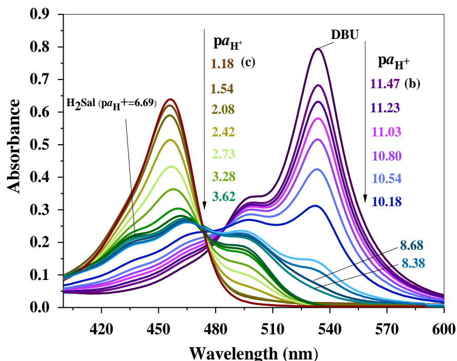
Figure 4.3: Steady-state absorption spectra of ethyl ester of 4'-nitrofluorescein in DMSO at different pa^*_{H^+} values where H_2Sal – salicylic acid, salicylate (a) and benzoate (b) buffer solutions and in p -toluenesulfonic acid solutions (c).
