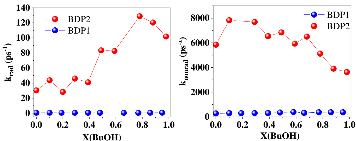
Figure 6.10: Evolution of fluorescence radiative and nonradiative rate constants of BDP1 and BDP2 in acetonitrile/butanol mixtures as a function of the molar fraction of the solvent.
