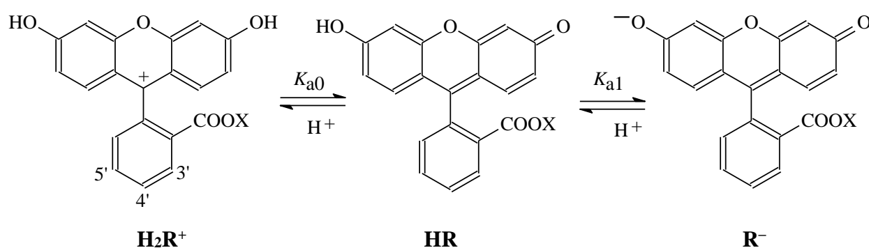
Scheme 4.3: Stepwise dissociation of the esters of nitro and amino fluoresceins; X = CH 3 or C 2 H 5 . The NO 2 or NH 2 groups occupy positions 3', 4', or 5'.
