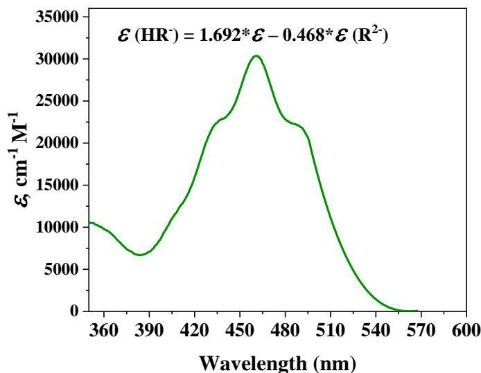
Figure 3.23: The spectrum of the single-charged anion of 5'-nitrofluorescein, \text{HR}^- , in DMSO.
