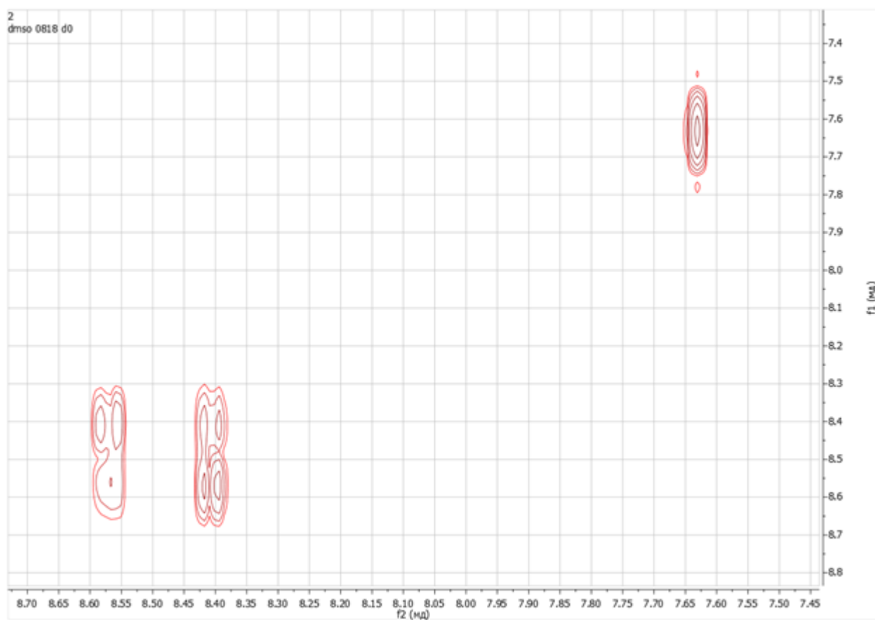
Figure A17: ^1\text{H} - ^1\text{H} COSY NMR spectrum of 2,4,5,7,5'-pentanitrofluorescein (400 MHz, \text{DMSO-}d_6 ).
