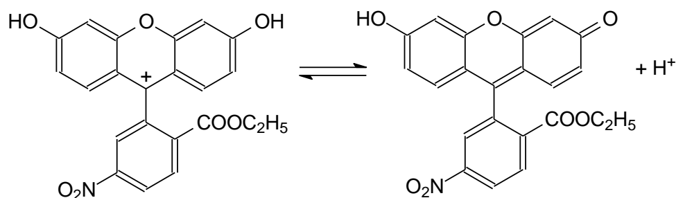
Figure 3.30: The dissociation scheme of the 5'-nitrofluorescein cation.
