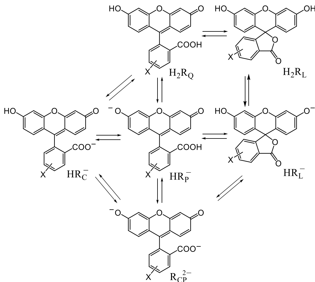
Scheme 5.1: The detailed equilibrium of fluorescein and aminofluoresceins; X = H: fluorescein; X = 4'-NH 2 : 4'-aminofluorescein; X = 5'-NH 2 : 5'-aminofluorescein.
