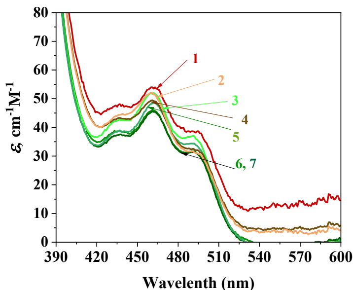
Figure 3.22: Absorption of 5'-nitrofluorescein around the spectra of the neutral form, H 2 R. The values in the activity scale pa_{\text{H}^+}^* are as follows: 4.12 (1); 3.60 (2); 7.11 (3); 3.90 (4); 6.72 (5); 6.36 (6); 6.03 (7); p -TSA and salicylic buffer solution were used.
