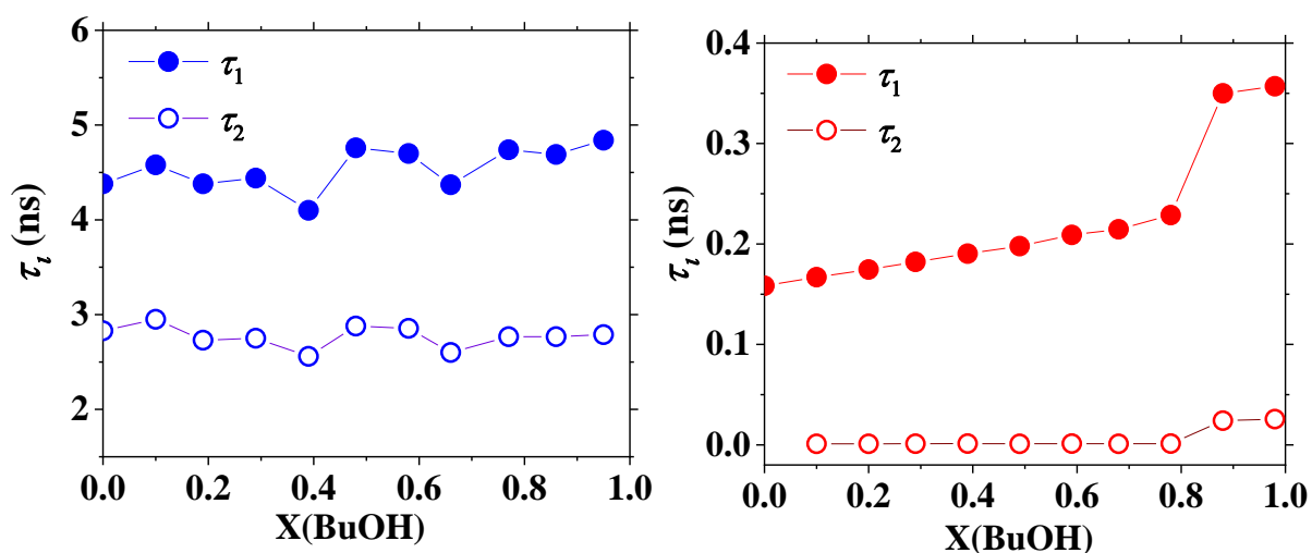
Figure 6.9: Evolution of the time components of BDP1(left) and BDP2 (right) fluorescence decay in acetonitrile/butanol mixtures in the function of the molar fraction of BuOH.
