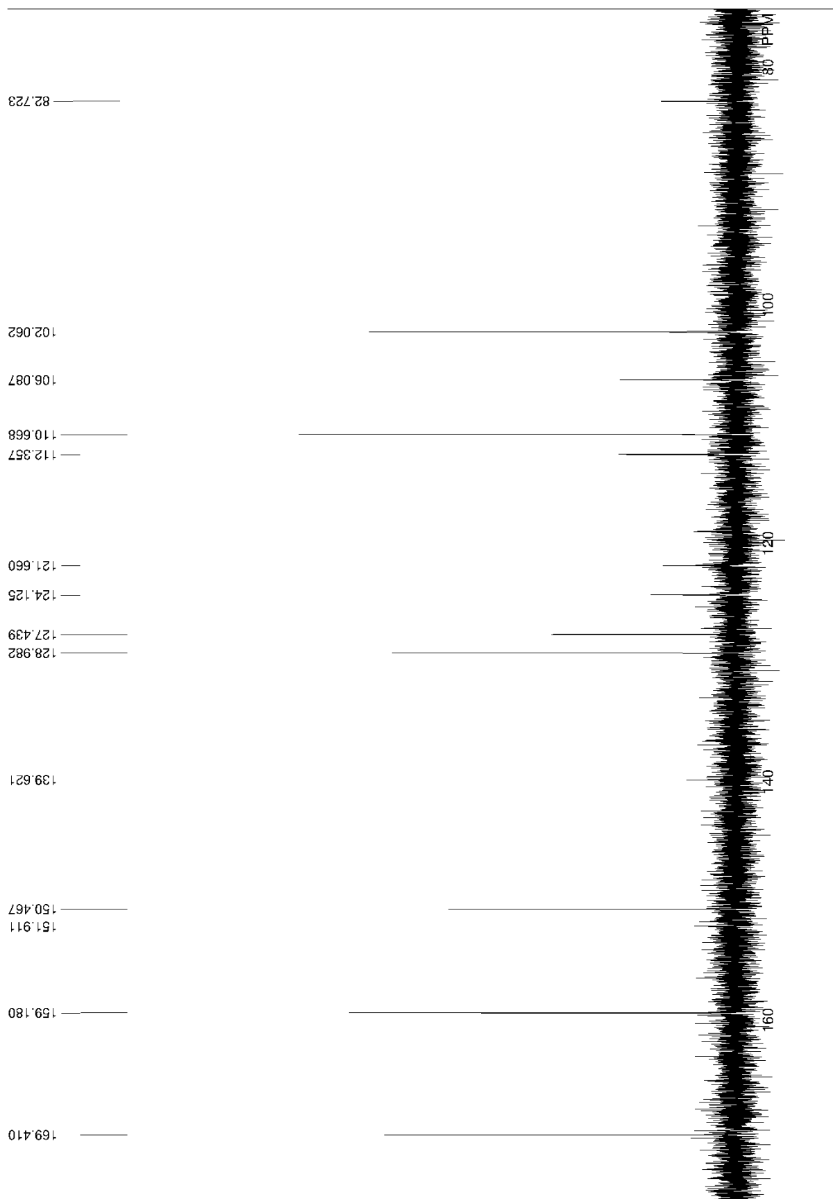
Figure A6: ^{13}\text{C} NMR spectrum of 4'-aminofluorescein (101 MHz, \text{DMSO-}d_6 ).
