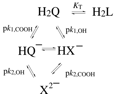
Figure 1.8: Detailed scheme of protolytic equilibrium of hydroxyxanthene dyes in solution.
