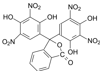
Figure 3.10: The molecular structure of the 2,4,5,7-tetranitrofluorescein with ruptured pyran ring (see also Chapter 2)
