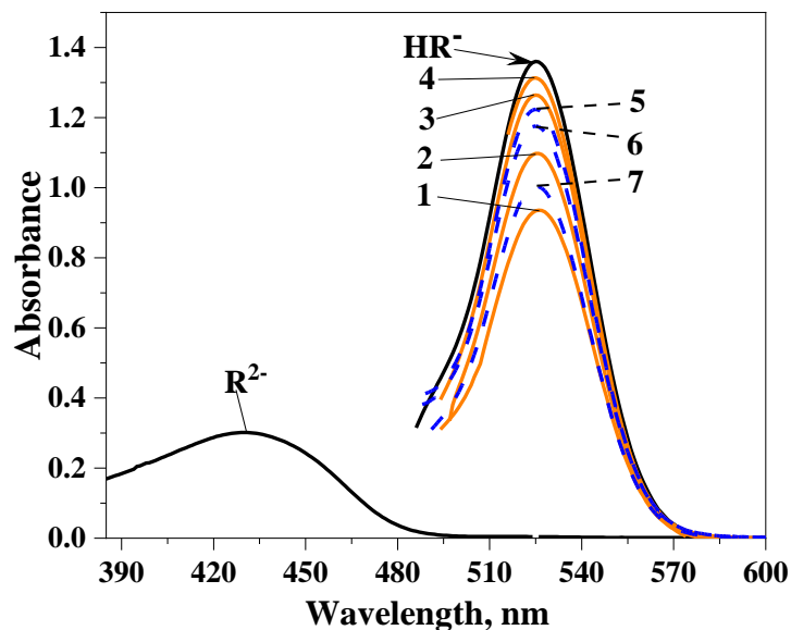
Figure 3.6: Steady-state absorption spectra of 2,4,5,7,4'-pentanitrofluorescein, 1.40 \times 10^{-5} M, in DMSO. The spectrum of the dianion R^{2-} was measured in 0.02 M DBU solution; the same spectrum was obtained in benzoate buffer solutions. The values for the picric acid solutions in the concentration scale, \text{pH}_c = -\log[\text{H}^+] , and in the activity scale \{ \text{p}a_{\text{H}^+}^* \} are as follows: 0.35 {0.66} (1); 0.66 {0.93} (2); 1.27 {1.44} (3); 1.81 {1.92} (4); 3.38 {3.40} (5); 3.51 {3.53} (6); 3.98 {3.99} (7); the spectrum within the range of 1.84 {1.92} to 3.08 {3.11} are almost invariable and correspond to the single-charged anion, \text{HR}^- . This is a representative set of points from a much larger body of data (see Figure 3.8).
