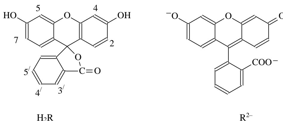
Figure 1.1: Molecular structures of neutral and dianionic forms of fluorescein.
