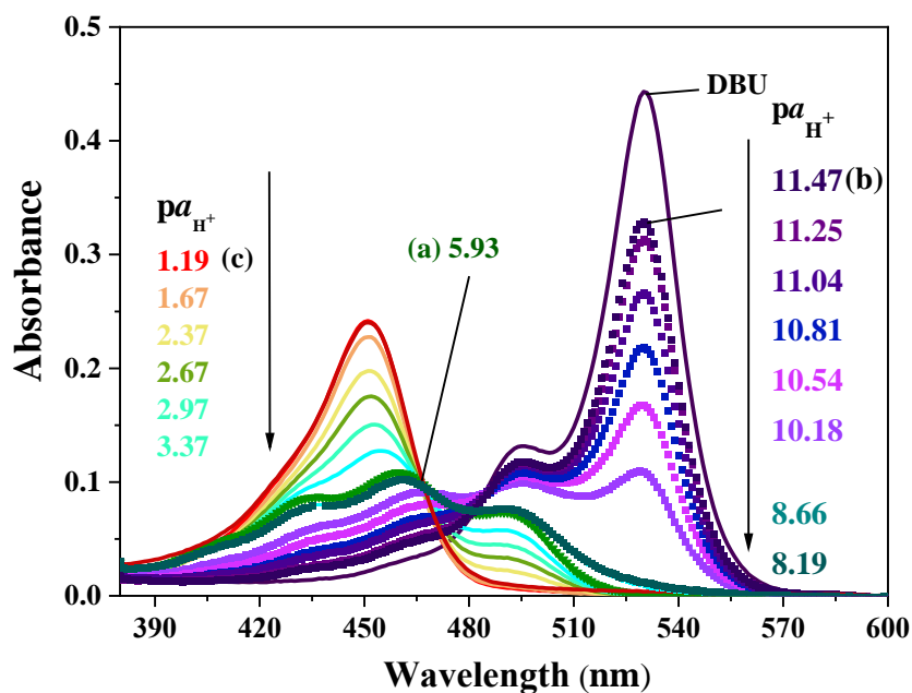
Figure C1: Steady-state absorption spectra of ethyl ester of fluorescein in DMSO at different pK_{aH^+} values in salicylate (a) and benzoate (b) buffer solutions and in p -toluenesulfonic acid solutions (c).
