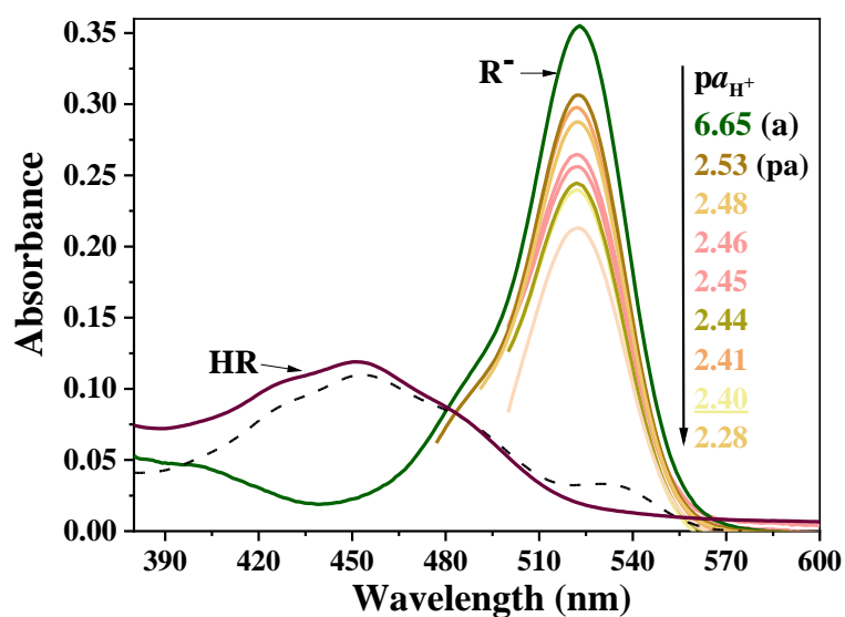
Figure 3.13: Steady-state absorption spectra of 2,4,5,7-tetranitrofluorescein methyl ester ( 3.1 \times 10^{-6} M) in the binary solvent at different picric acid solutions (pa). The spectrum of the anionic form R^- was obtained in a salicylate buffer solution (a). The spectrum of the entire HR form was measured in benzene with 0.1 M sulfuric acid; without such acidifying, some amounts of the anion R^- are present in the solution (dotted curve).
