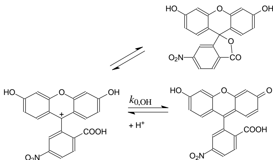
Figure 3.29: The dissociation scheme of the 5'-nitrofluorescein cation with the formation of the \text{H}_2\text{L} and \text{H}_2\text{Q} tautomers.
