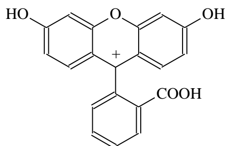
Figure 1.2: Molecular structure of fluorescein cation, H_3Z^+ .
