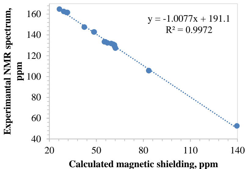
Figure 2.7: Correlation between the experimental and theoretical ( b3lyp/cc-pvdz/PCM ) ^{13}\text{C} NMR spectra of the anionic form of the 2,4,5,7-tetranitrofluorescein methyl ester in \text{DMSO-d}_6 .
