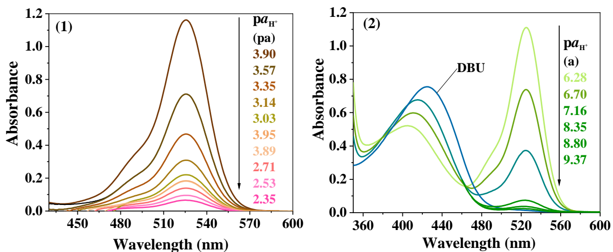
Figure 3.16: Steady-state absorption spectra of 2,4,5,7,4'-pentanitrofluorescein ( 4.7 \times 10^{-5} M) in diluted solutions of the picric acid (pa) (1) and in the salicylate buffer solutions (a) (2). The R^{2-} spectrum was obtained in 0.02 M DBU solution.
