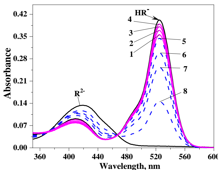
Figure 3.7: Steady-state absorption spectra of 2,4,5,7,5'-pentanitrofluorescein, 4.17 \times 10^{-6} M, in DMSO. The spectrum of the dianion R^{2-} was measured in 0.02 M DBU solution; the same
