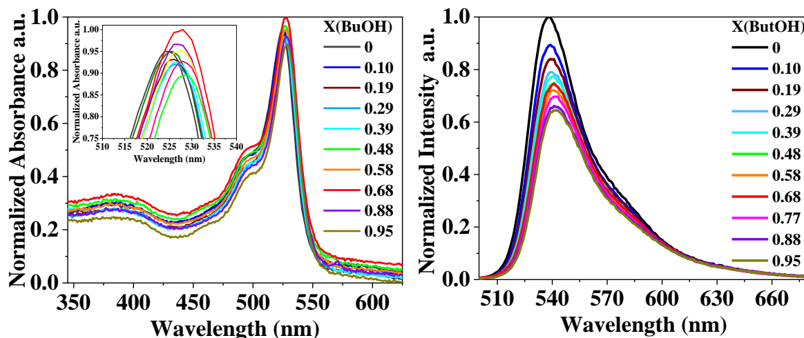
Figure 6.3: Normalized steady-state absorption (left) and emission (right) spectra of BDP1 in whole mixture composition of AN and BuOH ( \lambda_{\text{excitation}}=470 nm). The absorption spectra at the maximum are shown in the inset.
