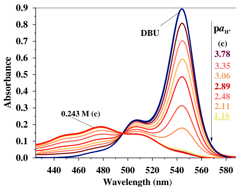
Figure 4.5: Steady-state absorption spectra of methyl ester of eosin in DMSO at different concentrations of p -toluenesulfonic acid (c); pa_{H^+}^* = -\log c_{H^+} - \log f_1 . The values below pa_{H^+}^*
