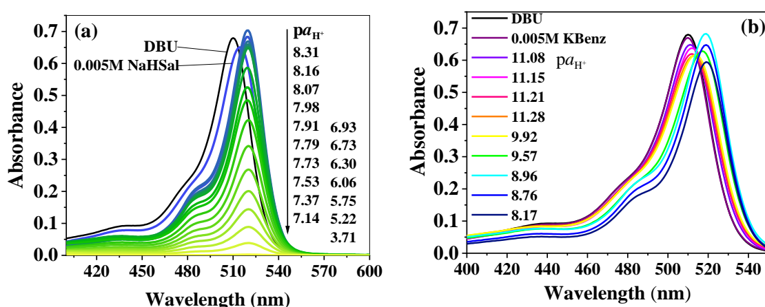
Figure 3.2. Steady-state absorption spectra of 4,5-dinitrofluorescein in DMSO at different pa_{H^+}^* values in salicylate (a) and benzoate (b) buffer solutions.
