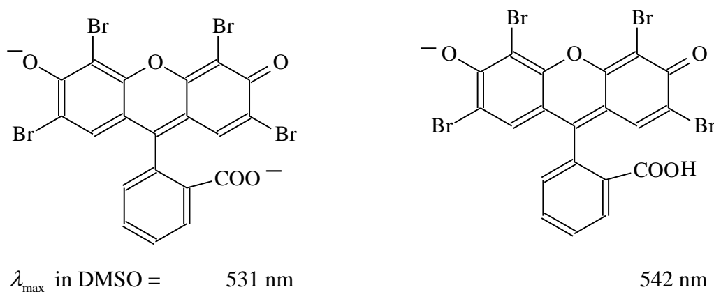
Scheme 4.1: Ions \text{R}^{2-} and \text{HR}^- anions of eosin
