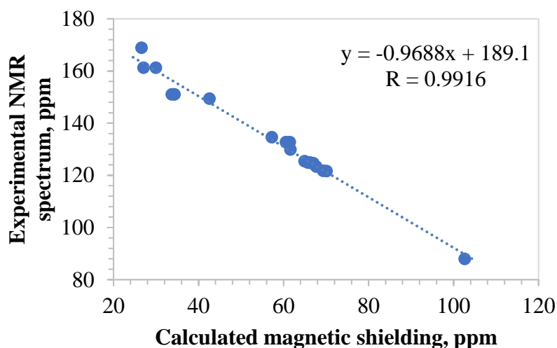
Figure 2.5: Correlation between the experimental and theoretical ( b3lyp/cc-pvdz/PCM ) ^{13}\text{C} NMR spectra of the 2,4,5,7-tetranitrofluorescein with the cleaved pyran ring, shown in Figure 2.4, in DMSO- \text{d}_6 .
