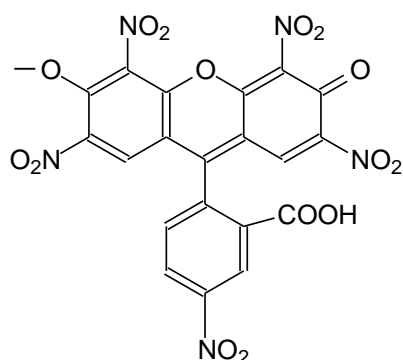
Figure 5.6: 2,4,5,7,4'-pentanitrofluorescein anion R^- .
