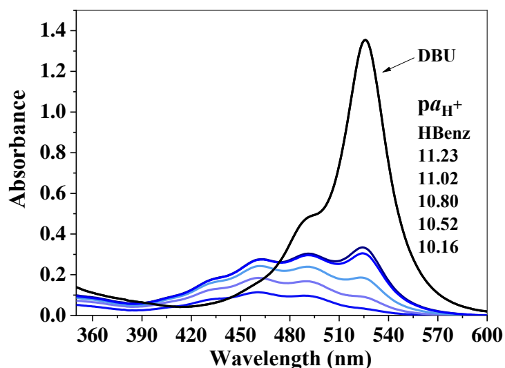
Figure 3.25: Steady-state absorption spectra of 4'-nitrofluorescein in DMSO in benzoate buffer solutions
