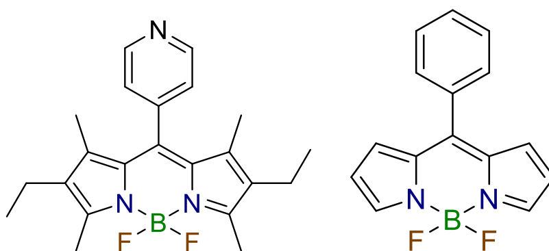
Figure 6.2: 1,3,5,7-tetramethyl-4,4-difluoro-2,6-diethyl-8-(4-pyridine)-4-boron-3a,4a-diaza-s-indacene – BDP1 (left) and 8-phenyl-4,4-difluoro-4-boron-3a,4a-diaza-s-indacene – BDP2 (right).
