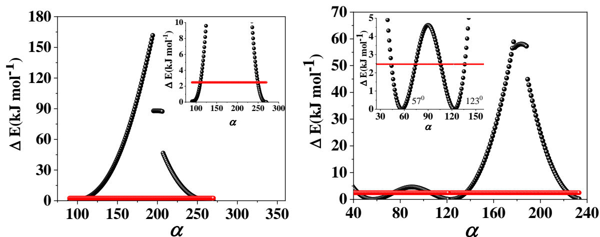
Figure 6.12: Potential energy profiles in the ground state for BDP1(left) and BDP2(right) along the dihedral angle ( C_1-C_5-C_6-C_7 , \alpha ) obtained with a hybrid functional cam-B3LYP at 6-311+G(d) basis set. The horizontal red line value is equal to the thermal energy 2.5 \text{ kJ}\cdot\text{mol}^{-1} . The potential energy curve lower than 2.5 \text{ kJ}\cdot\text{mol}^{-1} is presented closer (inset).
