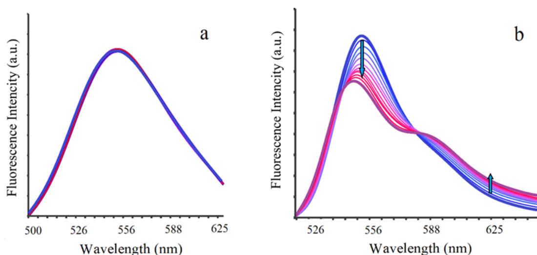
Figure 5.4: Time-resolved spectrum of 5'-aminofluorescein in DMSO at different p\alpha_{\text{H}^+} values. a: monoanion spectrum at p\alpha_{\text{H}^+} = 10.1 , benzoate buffer (a); spectrum at p\alpha_{\text{H}^+} = 12.0 , benzoate buffer (b). Starting curve is approximately 0.3 ns after pulse, the final curve is for 3 ns delay; the time gap between neighboring spectral curves is 0.1 ns.
