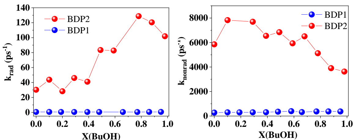
Figure 6.10: Evolution of fluorescence radiative and nonradiative rate constants of BDP1 and BDP2 in acetonitrile/butanol mixtures as a function of the molar fraction of the solvent.
