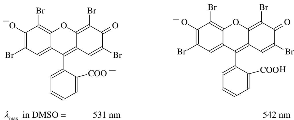
Scheme 4.1: Ions R 2- and HR - anions of eosin
