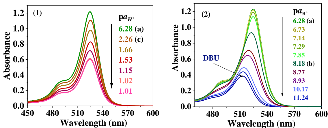
Figure 3.18: Steady-state absorption spectra of 4,5-dinitro-2,7-dibromofluorescein in DMSO at different pa_{H^+}^* : in p -toluenesulfonic acid solutions (c) and salicylate (a) and benzoate (b) buffer solutions.
