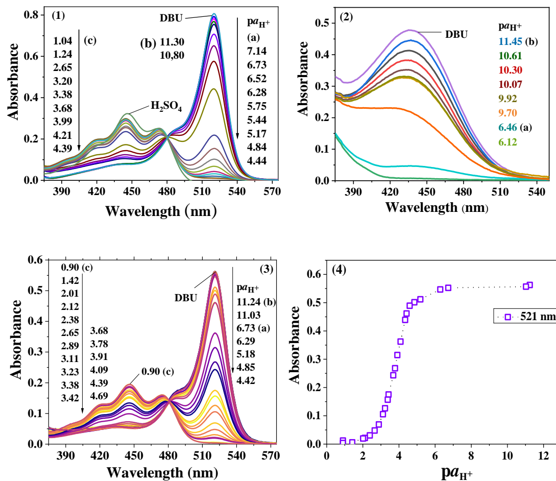
Figure 3.1: Steady-state absorption spectra in DMSO at different p\alpha_{\text{H}^+}^* values: 4,5-dinitrosulfofluorescein (1); 4,5-dinitrofluorescein methyl ether (2); 4,5-dinitrofluorescein methyl ester (3); and dependence of 4,5-dinitrofluorescein methyl ester absorbance at 522 nm on p\alpha_{\text{H}^+}^* (4) in DMSO at different p\alpha_{\text{H}^+}^* : in salicylate (a) and benzoate (b) buffer solutions and in p -toluenesulfonic acid solutions (c).
