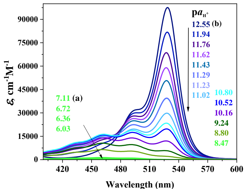
Figure 3.20: Steady-state absorption spectra of 5'-nitrofluorescein at different \text{p}a_{\text{H}^+}^* values in DMSO: salicylate (a) and benzoate (b) buffer solutions.
