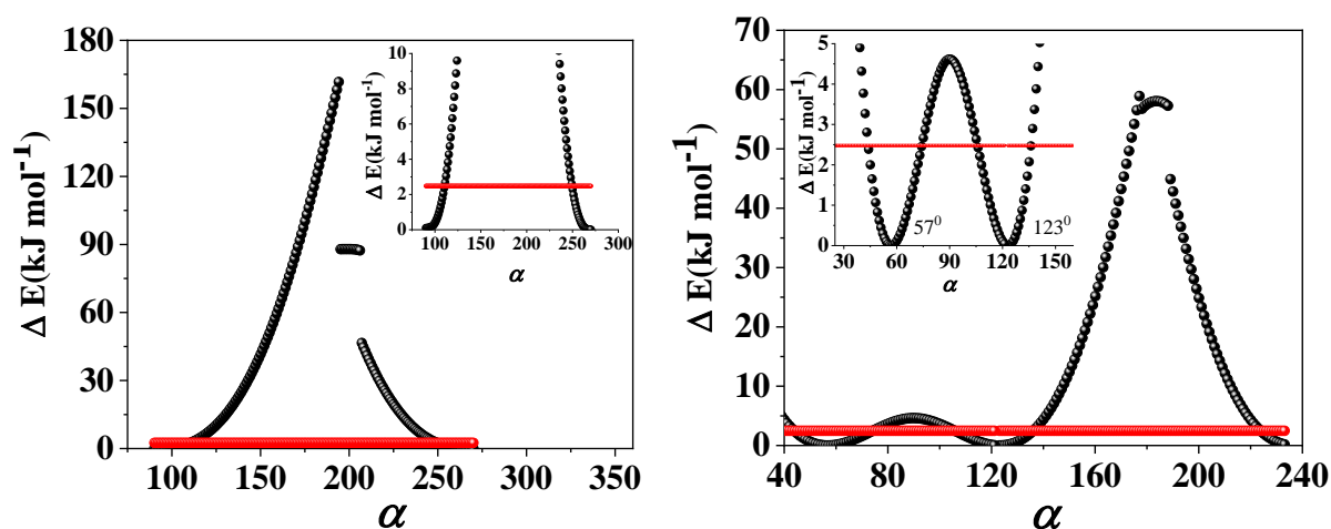
Figure 6.12: Potential energy profiles in the ground state for BDP1(left) and BDP2(right) along the dihedral angle ( C_1-C_5-C_6-C_7 , \alpha ) obtained with a hybrid functional cam-B3LYP at 6-311+G(d) basis set. The horizontal red line value is equal to the thermal energy 2.5 \text{ kJ}\cdot\text{mol}^{-1} . The potential energy curve lower than 2.5 \text{ kJ}\cdot\text{mol}^{-1} is presented closer (inset).
