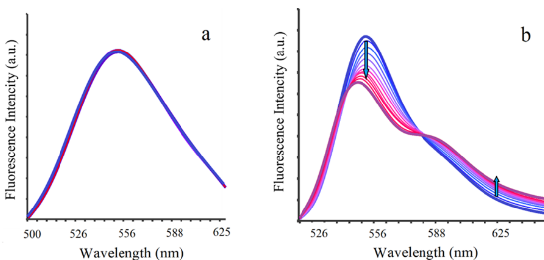
Figure 5.4: Time-resolved spectrum of 5'-aminofluorescein in DMSO at different p a_{\text{H}^+} values. a: monoanion spectrum at p a_{\text{H}^+} = 10.1 , benzoate buffer (a); spectrum at p a_{\text{H}^+} = 12.0 , benzoate buffer (b). Starting curve is approximately 0.3 ns after pulse, the final curve is for 3 ns delay; the time gap between neighboring spectral curves is 0.1 ns.
